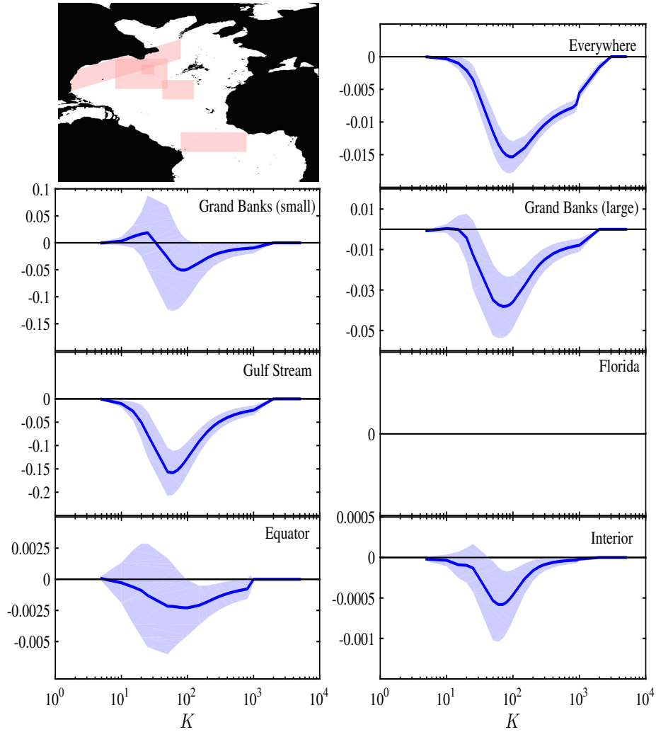
Figure 7: At 2,000 m depth: \langle \Pi_\ell \rangle (solid-blue line) as in the previous Figure 4. Units on the y-axis are in \text{W}/\text{km}^2/\text{m} . This is within the deep ocean, where stratification effects are, on average, weakest in the ocean. We notice that the energy transfer across scales is two order of magnitude smaller than in the mixed layer, near the surface.
