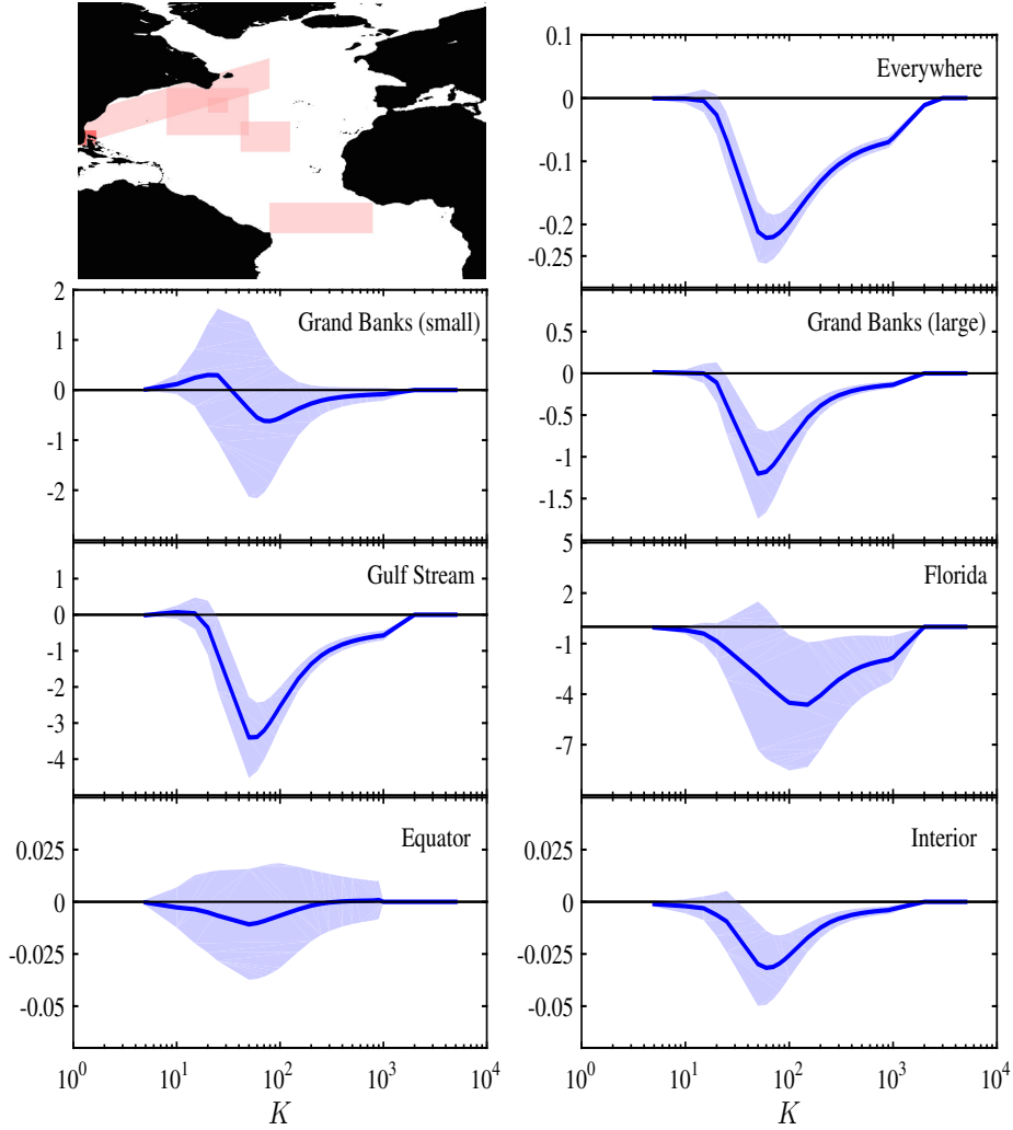
Figure 6: At 500 m depth: \langle \Pi_\ell \rangle (solid-blue line) as in the previous Figure 4. Units on the y-axis are in \text{W}/\text{km}^2/\text{m} . This depth is within the thermocline, where stratification effects are, on average, strongest in the ocean. We notice that the energy transfer across scales is an order of magnitude smaller here than in the mixed layer, near the surface.
