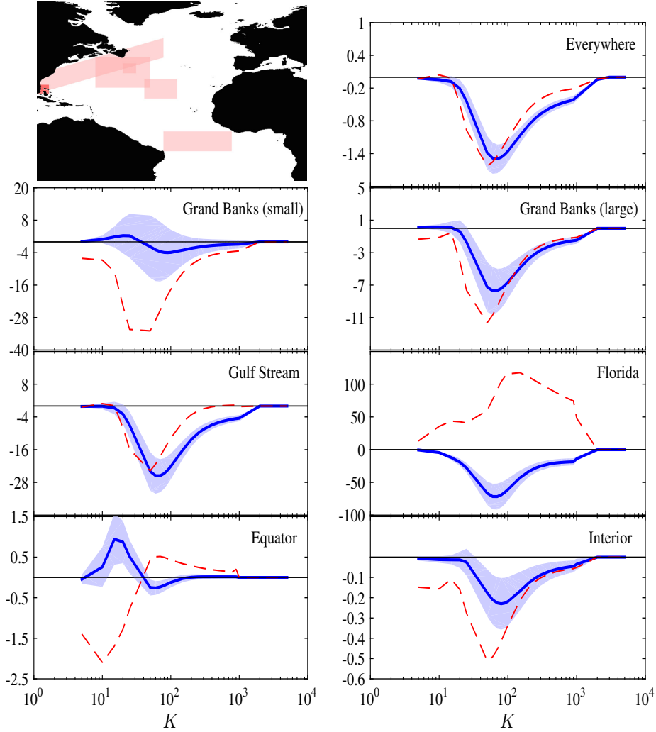
Figure 5: As in Figure 4 but at 100 m depth: \langle \Pi_\ell \rangle (solid-blue line) and \langle \Pi_\ell^{\text{HT}} \rangle (dashed-red). Units on the y-axis are in \text{W}/\text{km}^2/\text{m} . We again see significant differences between the two measures of energy transfer, especially in Florida, the Equator, and the Grand Banks where strong mean currents sweep through the box.
