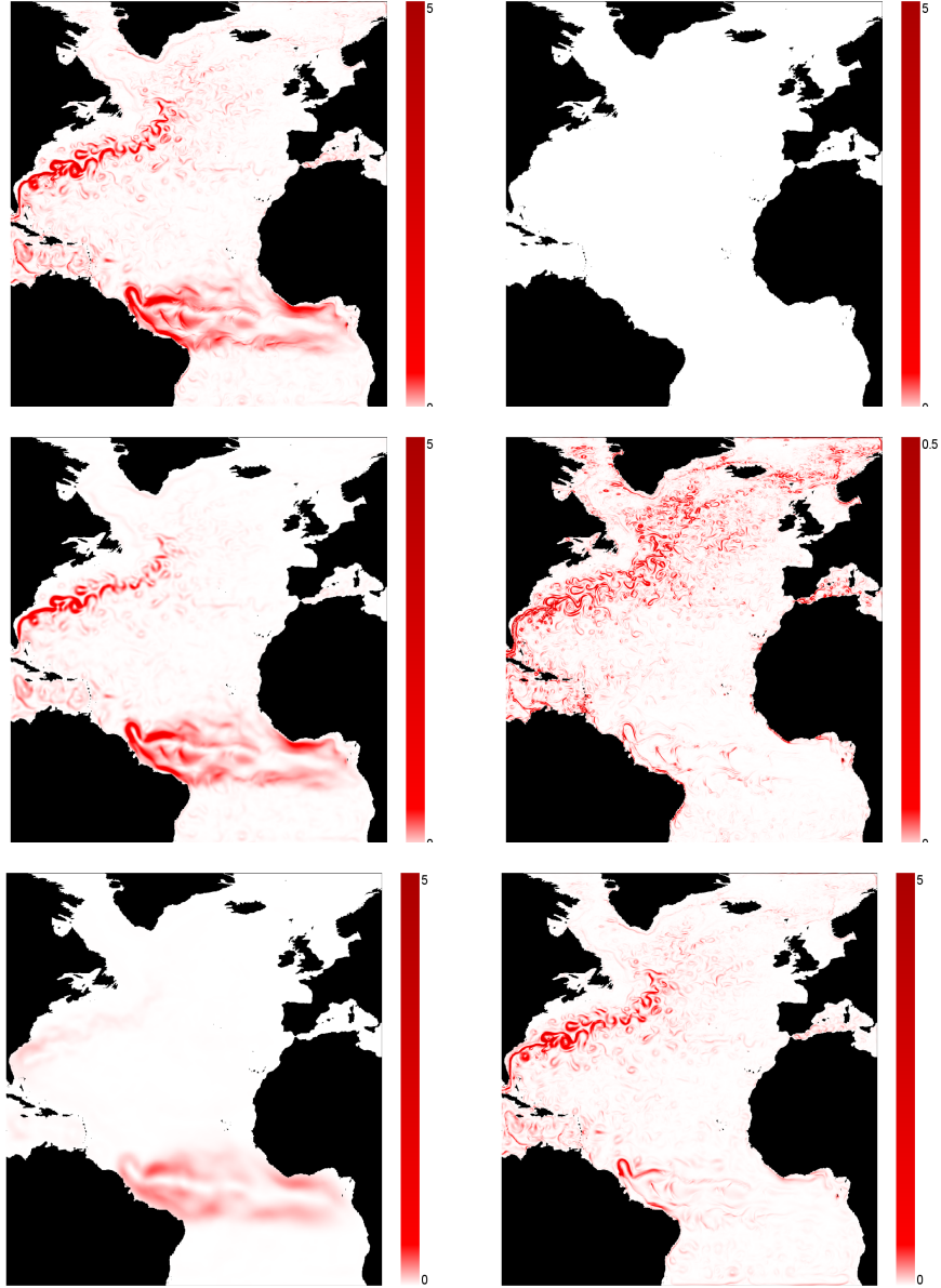
Figure 2: Our scale decomposition applied to model output (see Sec. 3) at a single instant of time. Left column shows KE |\bar{\mathbf{u}}_\ell|^2/2 (divided by density, in units of \text{m}^2/\text{s}^2 ), at scales larger than filtering scale \ell (eq. 1). Right column shows KE, |\mathbf{u}'_\ell|^2/2 , in the complementary small-scales (eq. 3). Rows show different filtering scales: (top) unfiltered with \ell = 0 km, (middle) filtered at scales \ell = 100 km and (bottom) \ell = 500 km. Note the order of magnitude change in color scale to show energy below \ell = 100 km (right middle panel). When visualizing in this manner, it is important to ensure the grid has sufficient resolution before taking the square of velocity to avoid aliasing effects.
