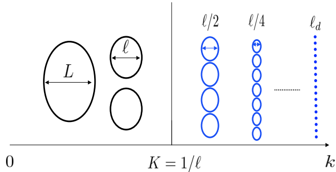
Figure 1: The coarse-graining approach. The system’s size is L , the largest scale. Below the viscous dissipation scale \ell_d , the dynamics is linear and modes are uncoupled. The dynamics over the entire scale-range L \geq \ell \geq \ell_d is given from a numerical simulation or an experiment. Scales are then partitioned (post-processing) into large and small. Length \ell represents the smallest scale that is resolved after coarse-graining. Scales < \ell (in blue) are averaged out.
