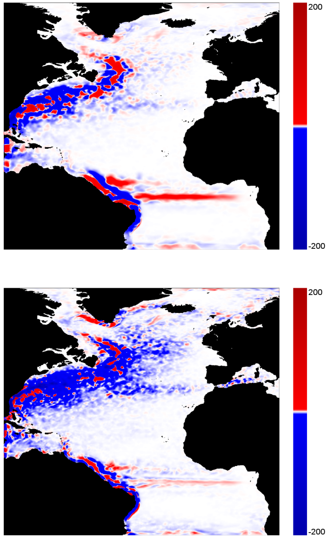
Figure 9: Maps of \Pi_\ell(\mathbf{x}) , as in Figure 8, but at 100 m depth, where \ell = 400 km (top) and \ell = 200 km (bottom). We notice in the Gulf Stream a pattern similar to that at the surface. In fact, almost the exact red/blue patch patterns that appear at the Gulf Stream surface appear at 100 m and 500 m depth (see next Fig. 10), suggesting that \Pi_\ell(\mathbf{x}) , as a scalar field, is depth-independent at high latitudes. On the other hand, we notice that there is a downscale transfer of energy in the Equatorial Counter Current, which in our simulation, is approximately at 0^\circ\text{N} and 100 m depth, indicating an obvious departure from the QG model.
