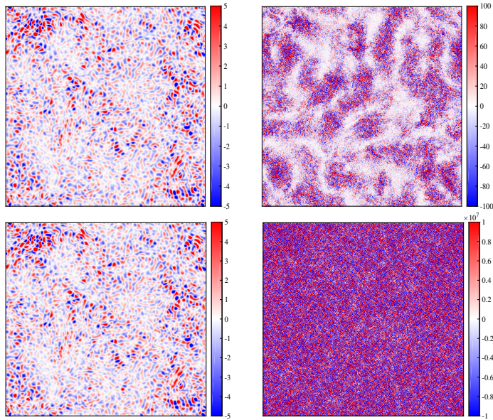
Figure 3: The energy transfer across scale \ell = L/30 ( L is the domain size), at a single time-instant, at every \mathbf{x} . Data is from a 3D triply periodic simulation of homogeneous isotropic turbulence forced at large-scales. Red (blue) is energy transferred from scales larger (smaller) than \ell to scales smaller (larger) than \ell . Top-left panel uses the SFS cascade measure, which is Galilean invariant, whereas the top-right panel uses the HT definition Frisch (1995), which is not, yielding an unphysical imprint of the large scales. Bottom two panels measure the energy transfer using the respective definitions after embedding the fluctuations in a uniform mean flow, underscoring the dependence of \Pi_\ell^{\text{HT}} on the observer’s inertial frame of reference.
