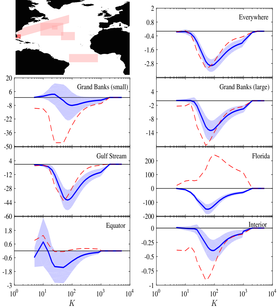
Figure 4: At the ocean surface: spatially averaged SFS flux (solid-blue line), \langle \Pi_\ell \rangle ( \text{W}/\text{km}^2/\text{m} ), as a function of scale, K = 10^4/\ell \text{ km}^{-1} . Here, K is not a wavenumber, just a number proportional to \ell^{-1} . The uppermost left panel shows the various regions over which \Pi_\ell(\mathbf{x}) is averaged. The transparent blue shade depicts the temporal standard deviation in the SFS flux over a 3-year period (110 snapshots), while the solid blue line is the temporal average. This is compared to the homogeneous turbulence flux (dashed-red), \langle \Pi_\ell^{\text{HT}} \rangle , without artificial tapering or boosting. Significant qualitative (and not just quantitative) differences in Florida, the Equator, and the Grand Banks where strong mean currents exist (Gulf stream and N. Equatorial current), sweeping through the box.
