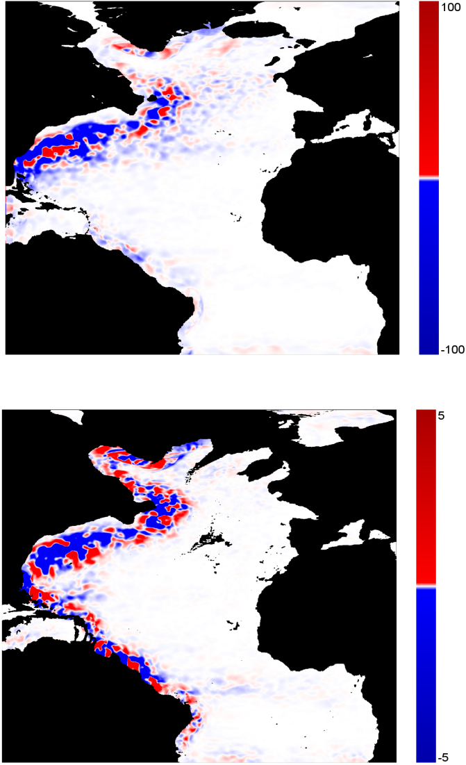
Figure 10: Map of \Pi_\ell(\mathbf{x}) , as in Figure 8, but at depths of 500 m (top) and 2,000 m (bottom), where \ell = 400 km. We notice that within the thermocline (top), scale-transfer is weak with the exception of the Gulf Stream which is known for its deep penetration. The red/blue patch patterns are similar to those appearing at the Gulf Stream surface and at 100 m. It is also clear from the color bar magnitudes of the bottom panel that there is relatively weak scale-transfer in the deep ocean.
