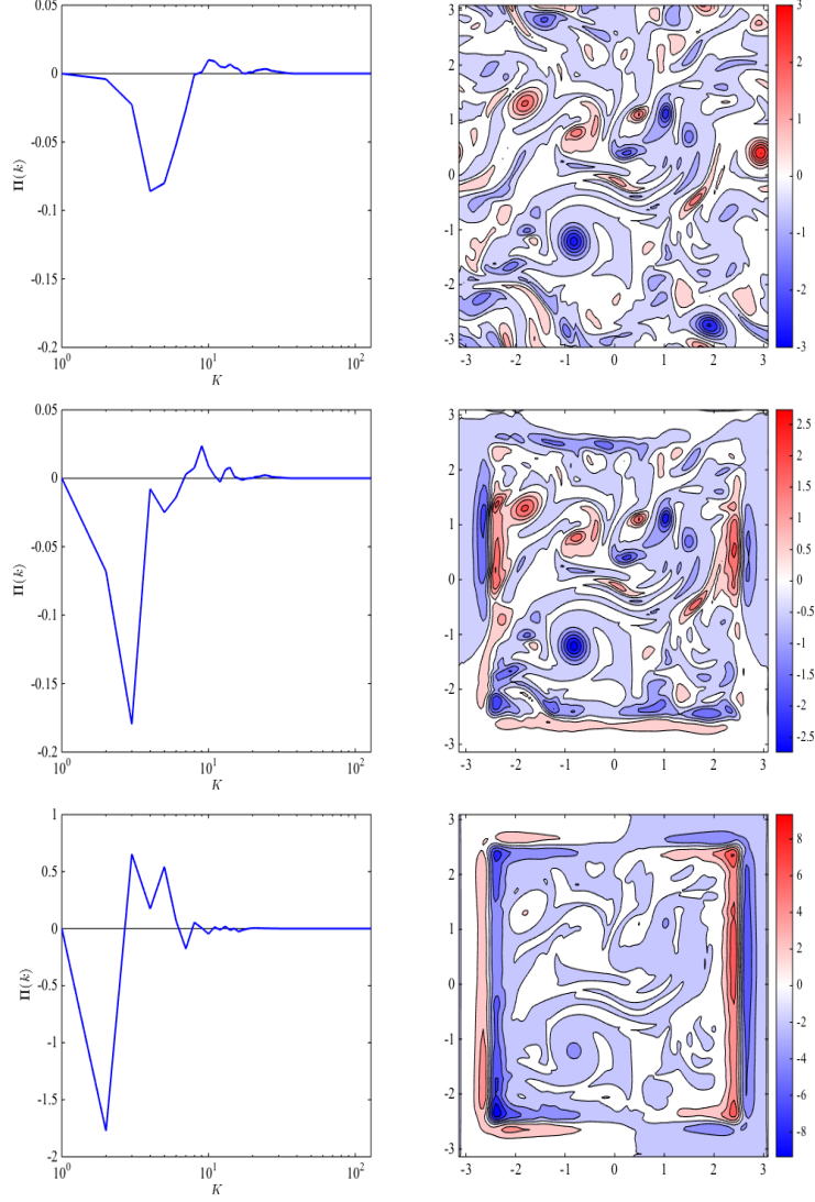
Figure 11: Left column shows \langle \Pi_K \rangle as a function of scale K = 2\pi/\ell . Right column shows vorticity contours. Top panels use original, \psi_{\text{orig}} , from a 2D flow with periodic boundaries. Middle panels use tapered streamfunction, similar to what was done in Arbic et al. (2013). Bottom panels adds a uniform velocity, U_0 \hat{\mathbf{i}} , to the original flow before tapering the streamfunction, \psi_{\text{orig}} + U_0 y , which illustrates the effect of tapering a jet. Even in the absence of a jet (middle), we see that tapering introduces artificial vorticity and shear to the flow, along with spurious length-scales. This is reflected as a shift in \langle \Pi_K \rangle to larger scales (smaller K ), along with significant changes in the magnitude of energy transfer.
