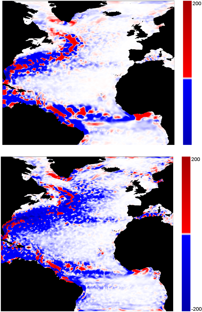
Figure 8: Geographic maps of the inter-scale energy transfer, \Pi_\ell(\mathbf{x}) ( \text{W}/\text{km}^2/\text{m} ), at the surface, time-averaged over 3 years (110 snapshots), where \ell = 400 km (top) and \ell = 200 km (bottom). The color map used, which has units of \text{W}/\text{km}^2/\text{m} , is not linear: most of the color shown has small values close to zero (white) and some blue/red regions exceed the maximum values on the color bar. We observe a downscale transfer in the current South of Florida, as the Gulf Stream turns northward, possibly indicative of eddy shedding or even just the small-scale associated with the sharp turn in the trajectory. We also observe a strong (dark blue) upscale transfer in the Gulf Stream core East of Florida and the Carolinas. This persists well beyond the separation point (Cape Hatteras), indicating that energy is transferred from mesoscale eddies into the Gulf Stream, accelerating and focusing the current. Flanking both sides of this (dark blue) core, we see downscale transfer (red) most probably associated with barotropic instabilities resulting from strong shear. Overall, an upscale transfer dominates in the Gulf Stream, in accord with QG. A similar pattern, though not as pronounced, exists in the N. Brazil Current. The (shallow) N. Equatorial Current, which in our simulation is around 5^\circ\text{N} , exhibits an upscale energy transfer.
