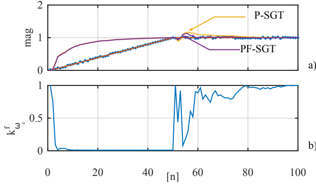
Fig. 5. Proposed fusion mechanism. a) evolution of the module. b) evolution of the gain. g_{h\omega_e} = 5 , \max(\Delta X_{h\omega_e}^{sgt}) = 1.1
