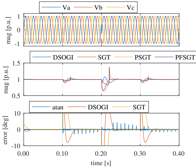
Fig. 14. Experimental results. Comparison between the DSOGI and the proposed PF-SGT methods for a phase step change. No harmonics are injected. From top to bottom: a) grid voltages, b) grid voltage magnitude, c) grid voltage phase error.
