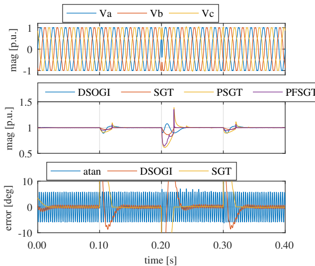
Fig. 15. Experimental results. Comparison between the DSOGI and the proposed PF-SGT methods for a phase step change. Harmonics as listed in Table I are injected. From top to bottom: a) grid voltages, b) grid voltage magnitude, c) grid voltage phase error.
