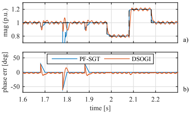
Fig. 7. Experimental results. Detail on the comparison of the PF-SGT method with respect to the ideal 1 st harmonic and the DSOGI implementation. a) module, b) phase.
