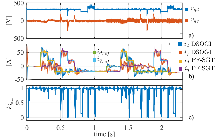
Fig. 8. Experimental results. Close loop comparison between the DSOGI and the proposed PF-SGT methods. a) grid voltages, b) grid currents, c) adaptive fusion gain for the PF-SGT method.
