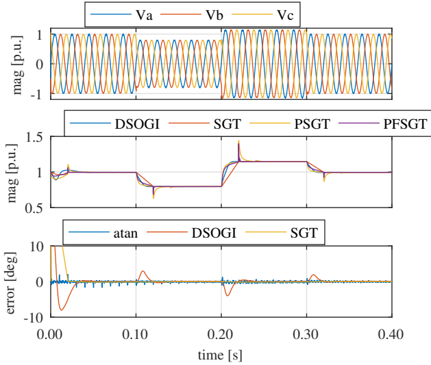
Fig. 10. Experimental results. Comparison between the DSOGI and the proposed PF-SGT methods for a magnitude step change. No harmonics are injected. From top to bottom: a) grid voltages, b) grid voltage magnitude, c) grid voltage phase error.
