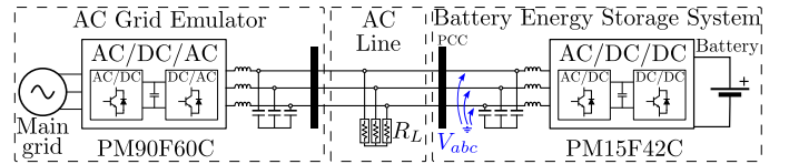
Fig. 9. Setup used for the experimental validation. Two converters are coupled together, PM90F60C unit is used to create the varying grid conditions and PM15F42C runs the proposed estimation method.
