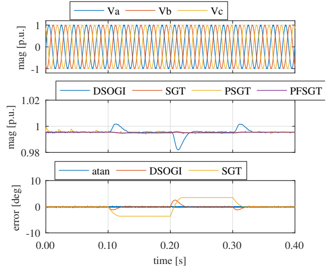
Fig. 12. Experimental results. Comparison between the DSOGI and the proposed PF-SGT methods for a frequency step change. No harmonics are injected. From top to bottom: a) grid voltages, b) grid voltage magnitude, c) grid voltage phase error.
