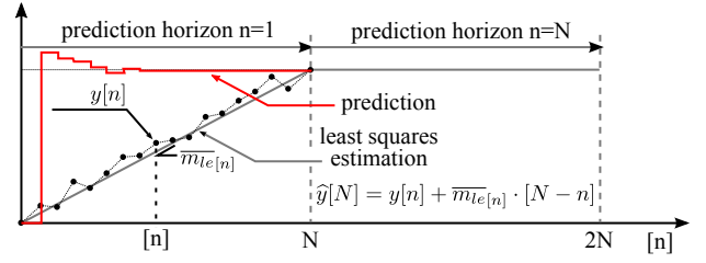
Fig. 3. Graphical representation of the proposed predictive algorithm. The slope at each of the points is filtered by a moving average filter for reducing the derivative noise.
