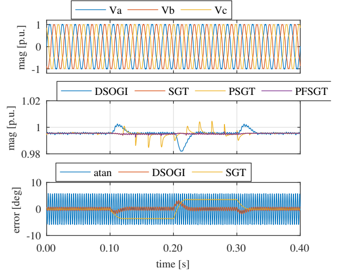
Fig. 13. Experimental results. Comparison between the DSOGI and the proposed PF-SGT methods for a frequency step change. Harmonics as listed in Table I are injected. From top to bottom: a) grid voltages, b) grid voltage magnitude, c) grid voltage phase error.
