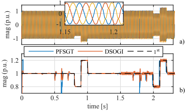
Fig. 6. Experimental results. Comparison of the PF-SGT method with respect to the ideal 1 st harmonic and the DSOGI implementation. a) evolution of time domain waveforms, b) evolution of the module estimation.
