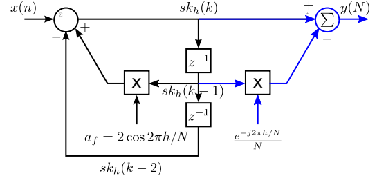
Fig. 1. IIR implementation of the Goertzel algorithm. Black traces are for the recursive part implementation. Blue traces represent the operations to be done at the last step ( k = N ).
