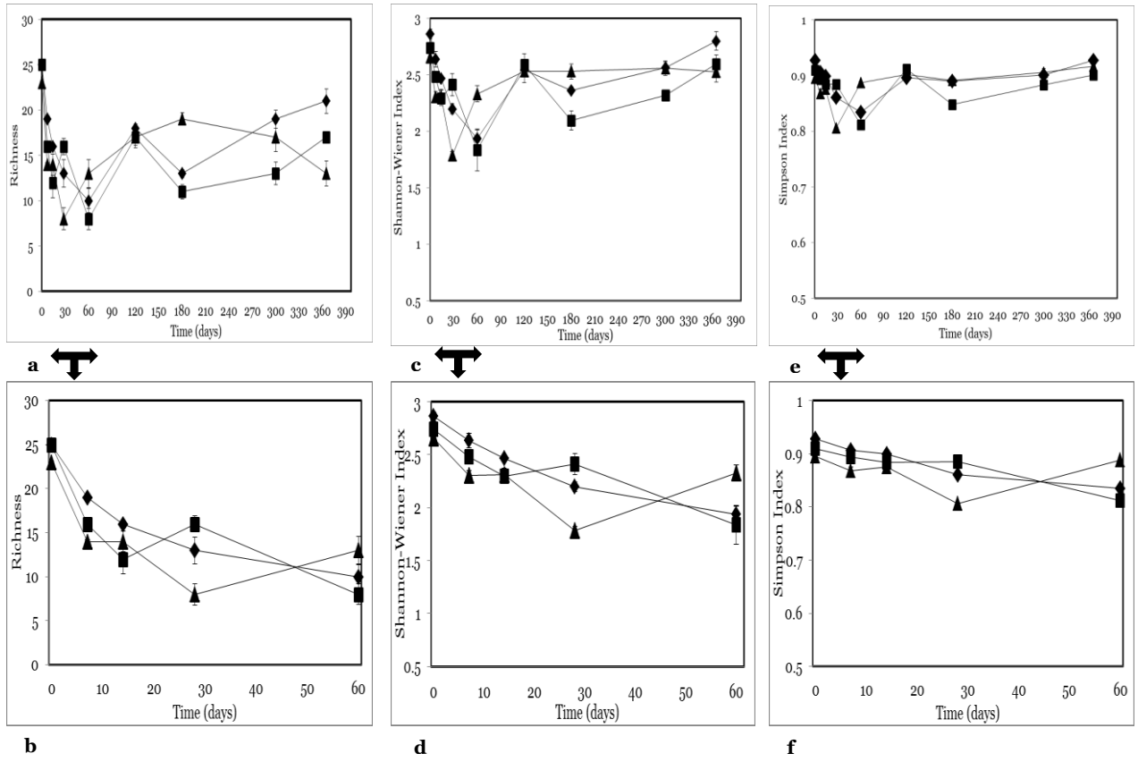
Fig. 4. a, 4c and 4e: average ( n=3 ) richness, Shannon-Wiener diversity index and Simpson diversity index for 18S fungal communities for control ( \blacklozenge ), Sus scrofa domestica ( \blacksquare ) and grass ( \blacktriangle ) soil microcosms during 365 days of study. b, 4d and 4f: Average ( n=3 ) richness, Shannon-Wiener diversity index and Simpson diversity index for 18S fungal communities for control ( \blacklozenge ), Sus scrofa domestica ( \blacksquare ) and grass ( \blacktriangle ) soil microcosms from day 0 to day 60.
