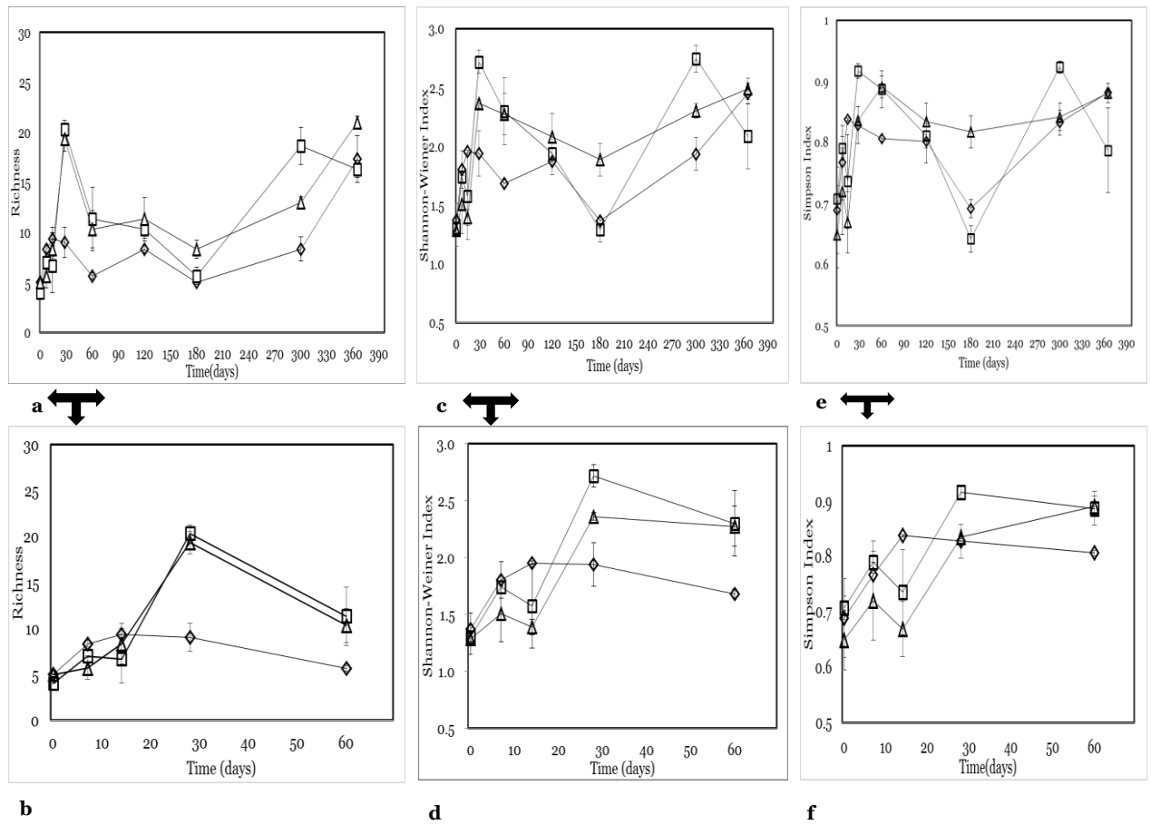
Fig. 3. a, 3c and 3e: Average ( n=3 ) richness, Shannon-Wiener diversity index and Simpson diversity index for 16S bacteria communities of control ( \diamond ), Sus scrofa domestica ( \square ) and grass ( \Delta ) soil microcosms during 365 days of study. b, 3d and 3f: Average ( n=3 ) richness, Shannon-Wiener diversity index and Simpson diversity index for 16S bacteria communities of control ( \diamond ), Sus scrofa domestica ( \square ) and grass ( \Delta ) soil microcosms from day 0 to day 60.
