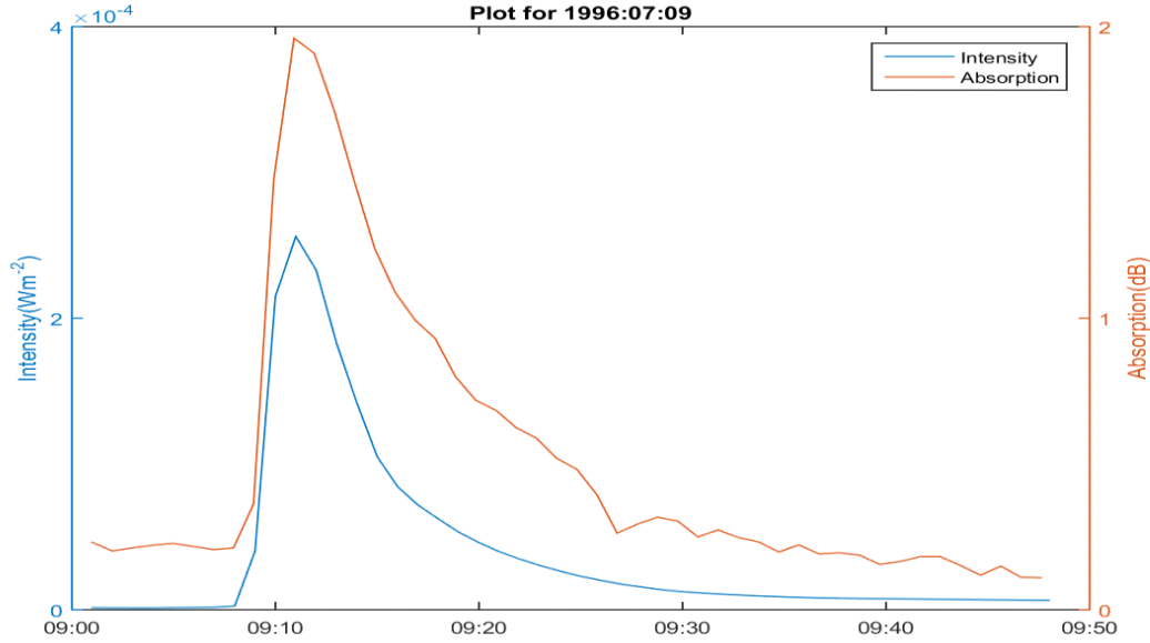
Figure 9: Typical relationship between absorption (dB) and flare intensity ( \text{Wm}^{-2} ) for M-class flare event (upper panel-6 th June 2000) and an X-class event (lower panel- 9 th July 1996).
