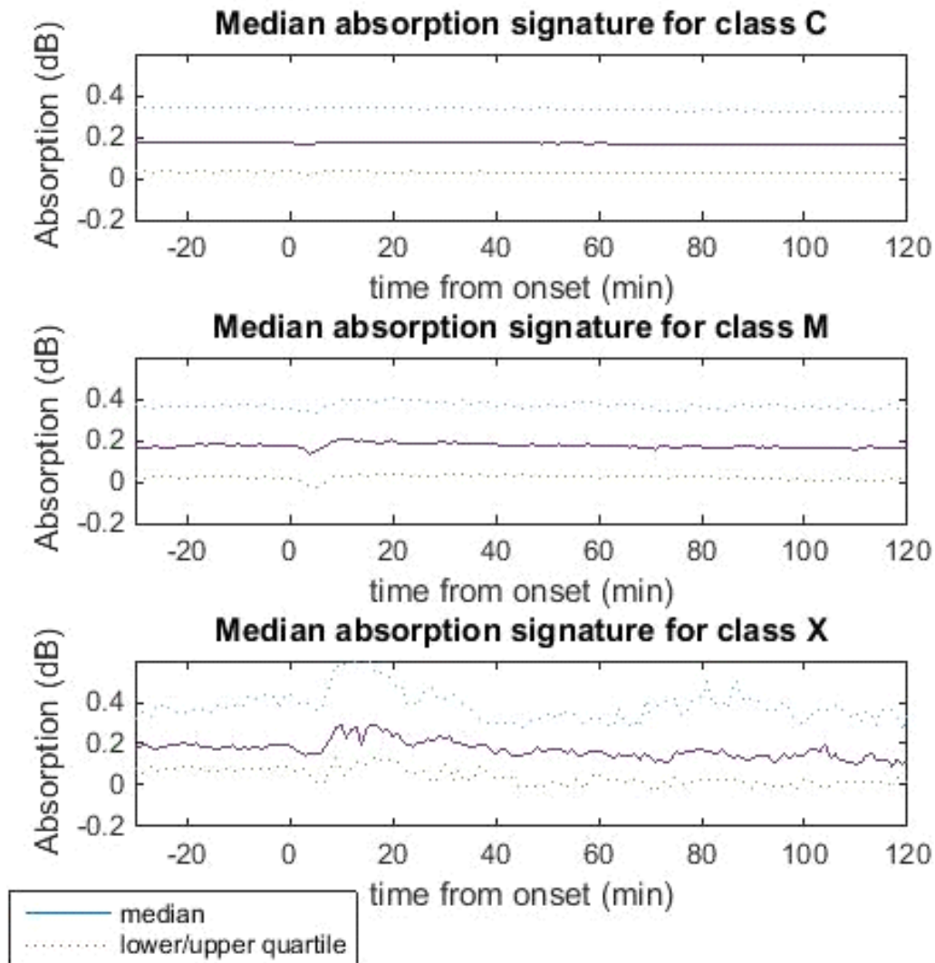
Figure 5: Superposed epoch analysis of median absorption signature for X, M and C class flare (1996-2009). The start times are as recorded by GOES. Absorption data is from beam 25 of IRIS Kilpisjarvi.
