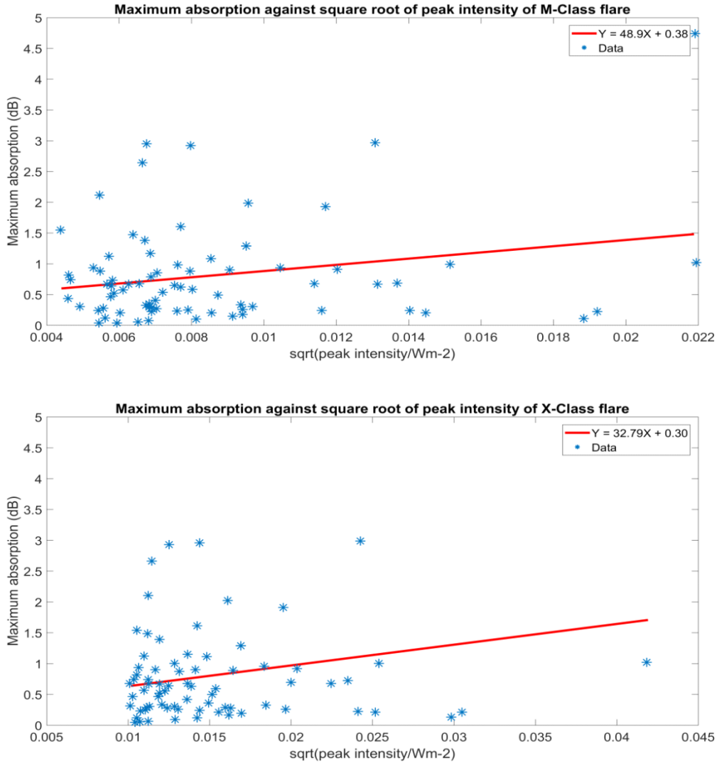
Figure 8: Plot of maximum absorption (dB) vs. square root of maximum flare intensity ( Wm^{-2} ), Top panel show M-class relation, bottom panel shows X-class relation.
