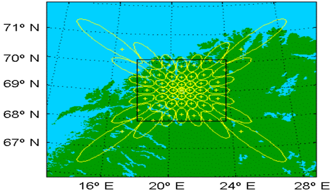
Figure 2: Beam projection of IRIS at 90 km altitude. The contours define the -3 dB points and the black square shows the calculated field of view used in the IRIS images.
