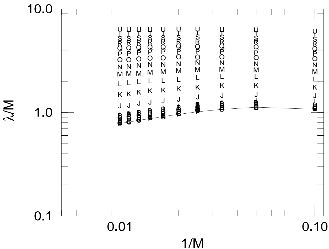
FIG. 13. Reduced localization lengths \lambda(M)/M vs. 1/M at E = 0 for random hopping and an additional small potential disorder W = 0.0001 . The \lambda/M scale is the same as in Fig. 11 for easier comparison. The line connects data corresponding to c = 0.25 .
