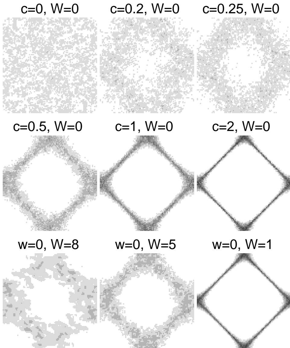
FIG. 2. Probability density of the Fourier transforms of eigenfunctions with the same parameters as shown in Fig. 1, but averaged over 10 states close to the band center. Different gray levels ( i = 0, 1, \dots, 6 ) distinguish whether |\phi_j(k_n, k_m)|^2 > 2^i/L^2 .
