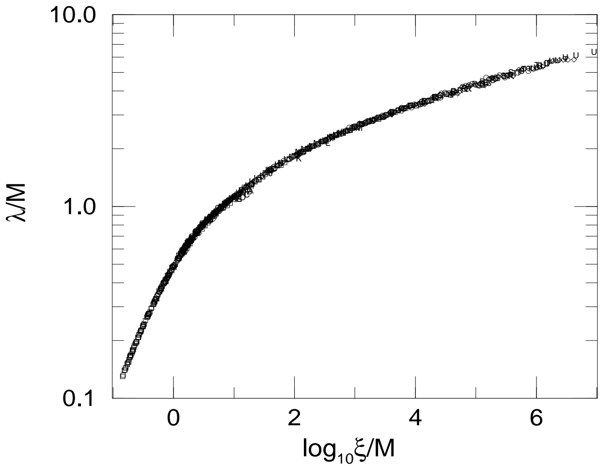
FIG. 11. Finite-size scaling plot of the reduced localization lengths \lambda(M)/M for random hopping at E = 0 and additional potential disorder W = 0.0001 ( \diamond ), 0.001 (characters as in Fig. 8), 0.01 ( \circ ) and 0.1 ( \square ). For W = 0.0001 , only data with M \geq 40 has been used. The small deviations from FSS at \xi/M \approx 10 , \lambda/M \approx 1 are coming from data for W = 0.001 and M = 10 .
