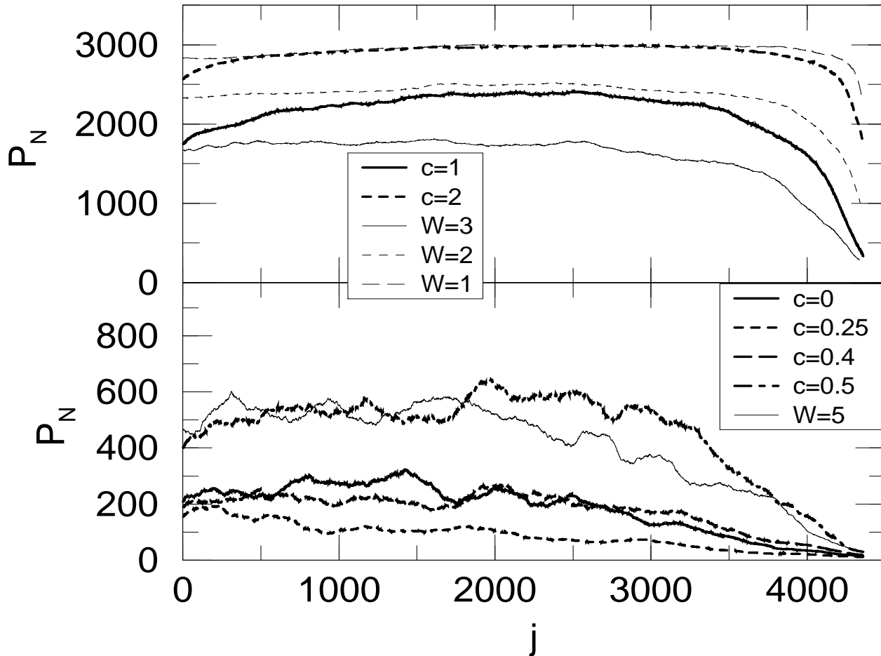
FIG. 4. Averaged participation numbers P_N versus the number j of the eigenstate ordered with increasing energy ( 0 \leq E_j \leq E_{j+1} ) and N = 96 \times 96 . Purely off-diagonal disorders are shown by thick lines, purely diagonal disorders by thin lines.
