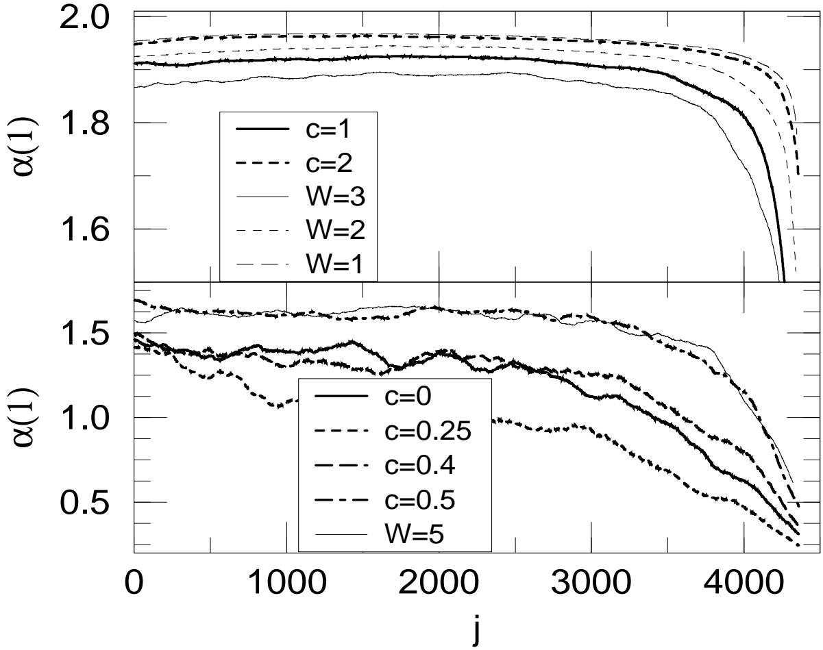
FIG. 6. Singularity strength \alpha(1) versus the number j of the eigenstate ordered with increasing energy ( 0 \leq E_j \leq E_{j+1} ) and N = 96 \times 96 . Purely off-diagonal disorders are shown by thick lines, purely diagonal disorders by thin lines.
