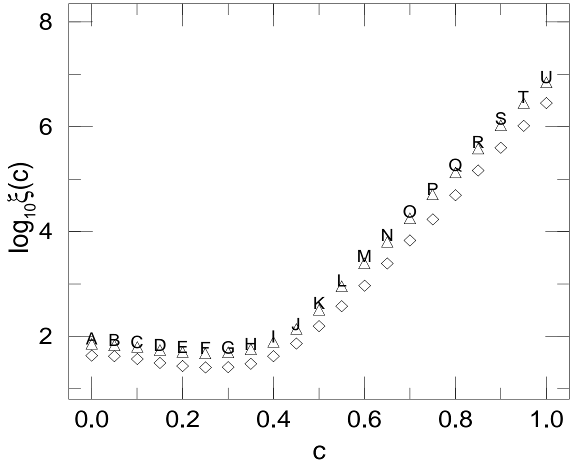
FIG. 9. Scaling parameter \xi as a function of off-diagonal disorder center c for W = 0 and E = 0.005 (characters), 0.01 ( \triangle ) and 0.1 ( \diamond ).
