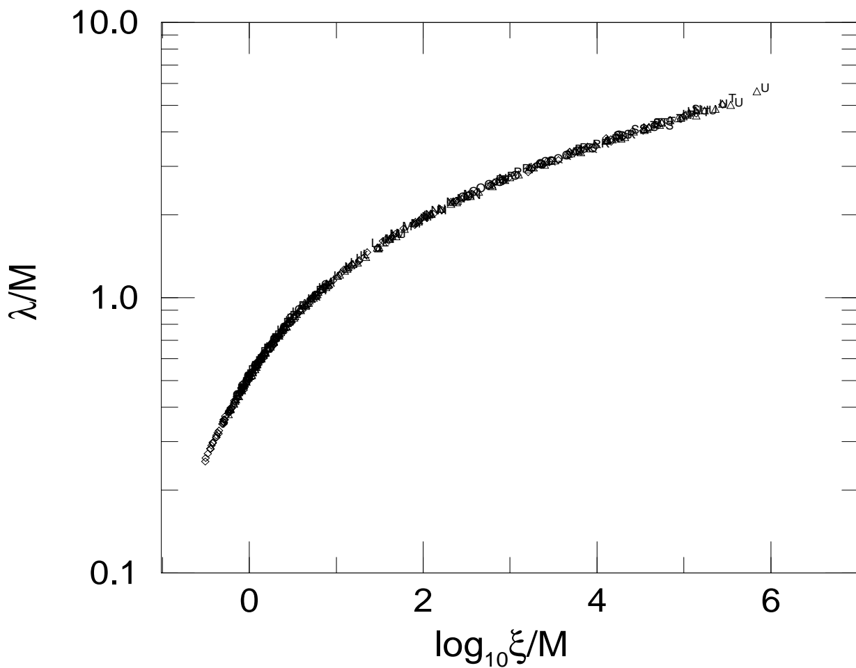
FIG. 8. Finite-size scaling plot of the reduced localization lengths \lambda(M)/M for purely random hopping ( W = 0 ) outside the band center with energies E = 0.005 (characters), E = 0.01 ( \Delta ) and E = 0.1 ( \diamond ). The off-diagonal disorder strengths corresponding to c = 0, 0.05, \dots, 1 are indicated by A, B, \dots , U, respectively.
