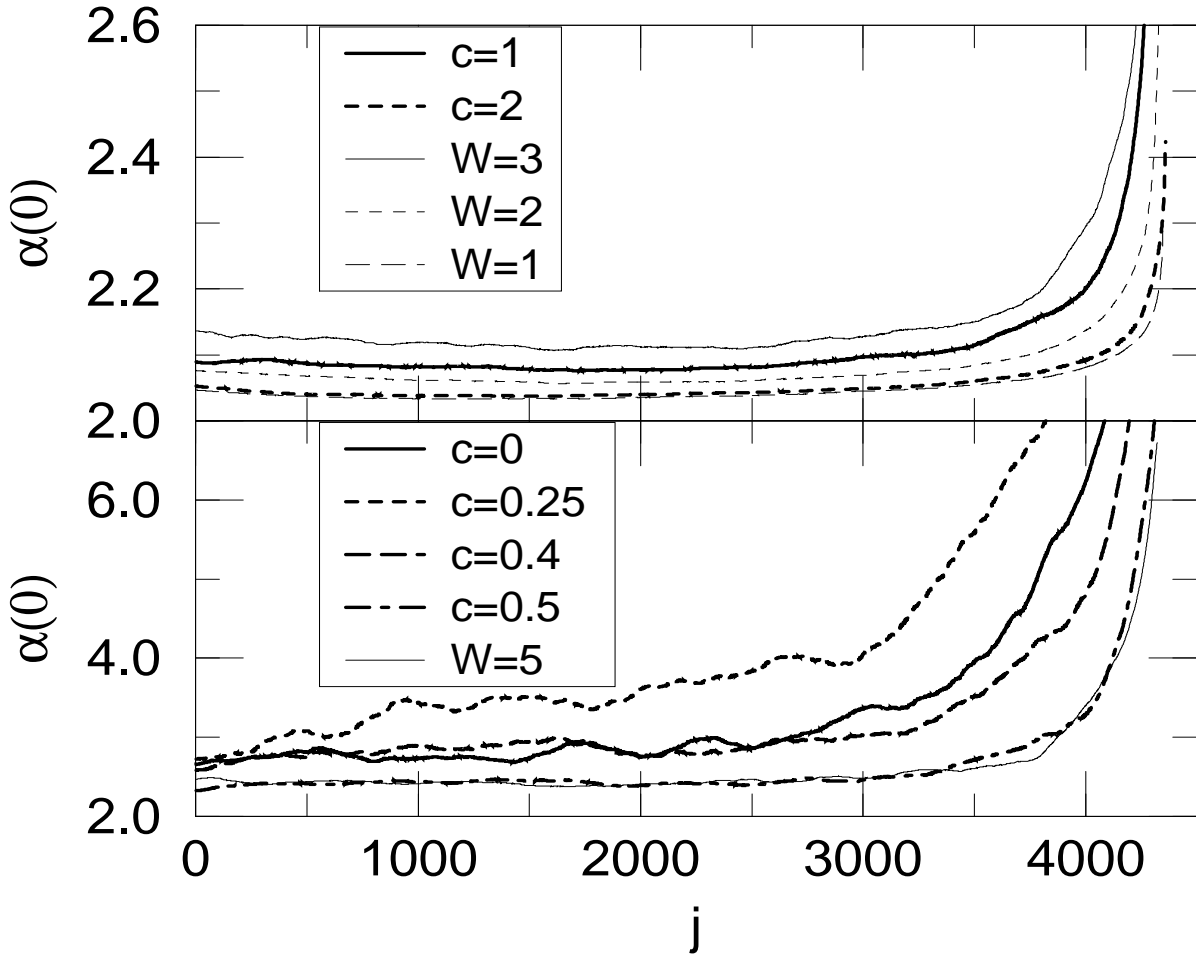
FIG. 5. Singularity strength \alpha(0) versus the number j of the eigenstate ordered with increasing energy ( 0 \leq E_j \leq E_{j+1} ) and N = 96 \times 96 . Purely off-diagonal disorders are shown by thick lines, purely diagonal disorders by thin lines.
