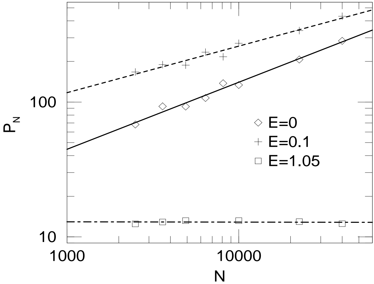
FIG. 7. Finite-size dependence of the participation numbers P_N for eigenstates with c = 0 at energies in the band center ( E = 0 ), outside the band center but still close to the peak in the DOS ( E = 0.1 ), and close to the band edge ( E = 1.05 ).
