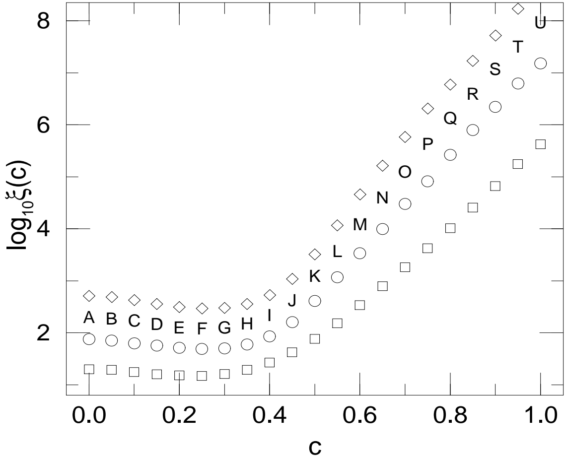
FIG. 12. Scaling parameter \xi as a function of off-diagonal disorder center c at E = 0.0 and diagonal disorder W = 0.0001 ( \diamond ), 0.001 (characters), 0.01 ( \circ ) and 0.1 ( \square ).
