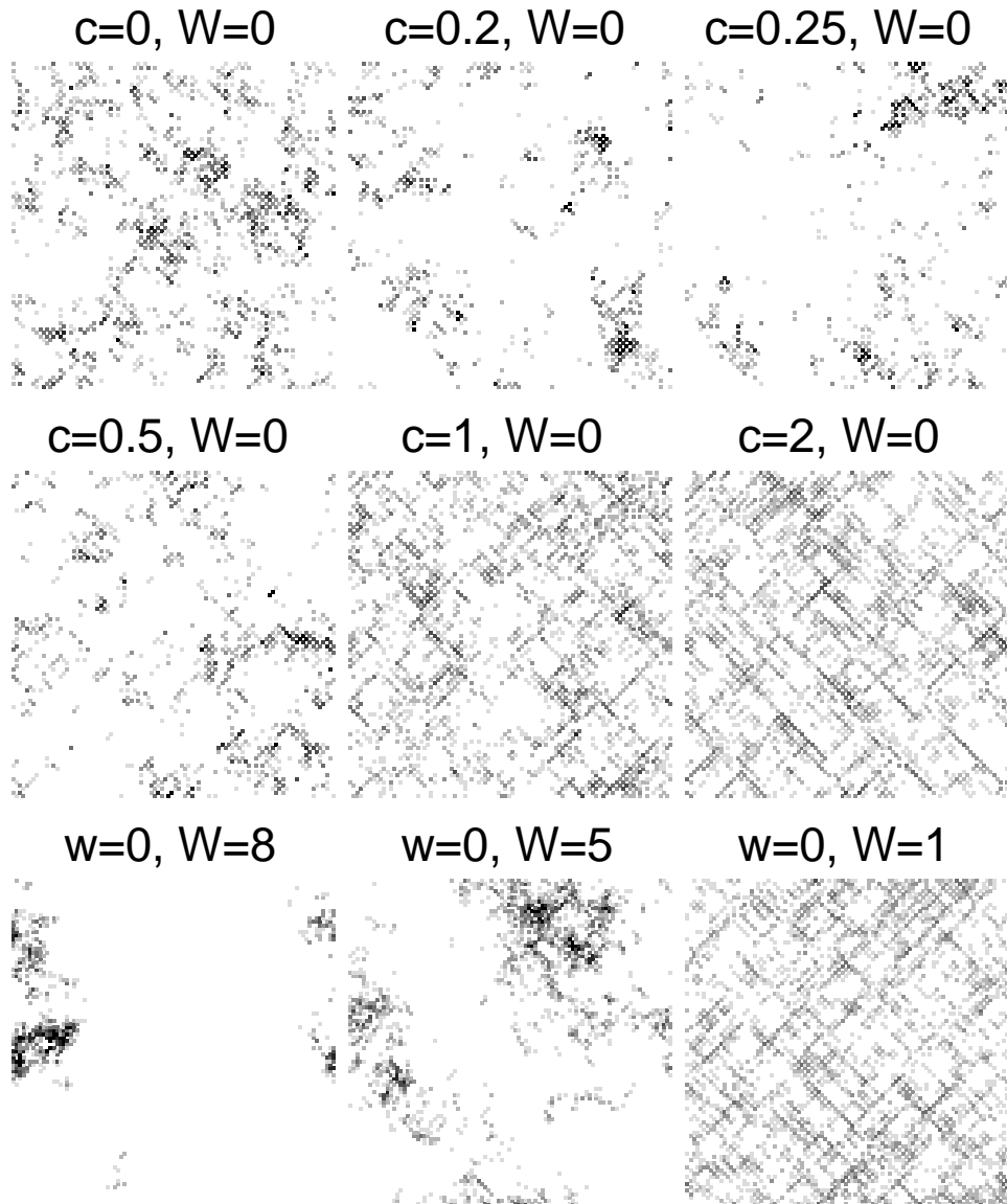
FIG. 1. Probability density |\phi_j|^2 of the eigenstate j closest to the band center for various off-diagonal and diagonal disorders and system size L = 96 . Different gray levels ( i = 0, 1, \dots, 6 ) distinguish whether |\phi_j(n, m)|^2 > 2^i/L^2 .
