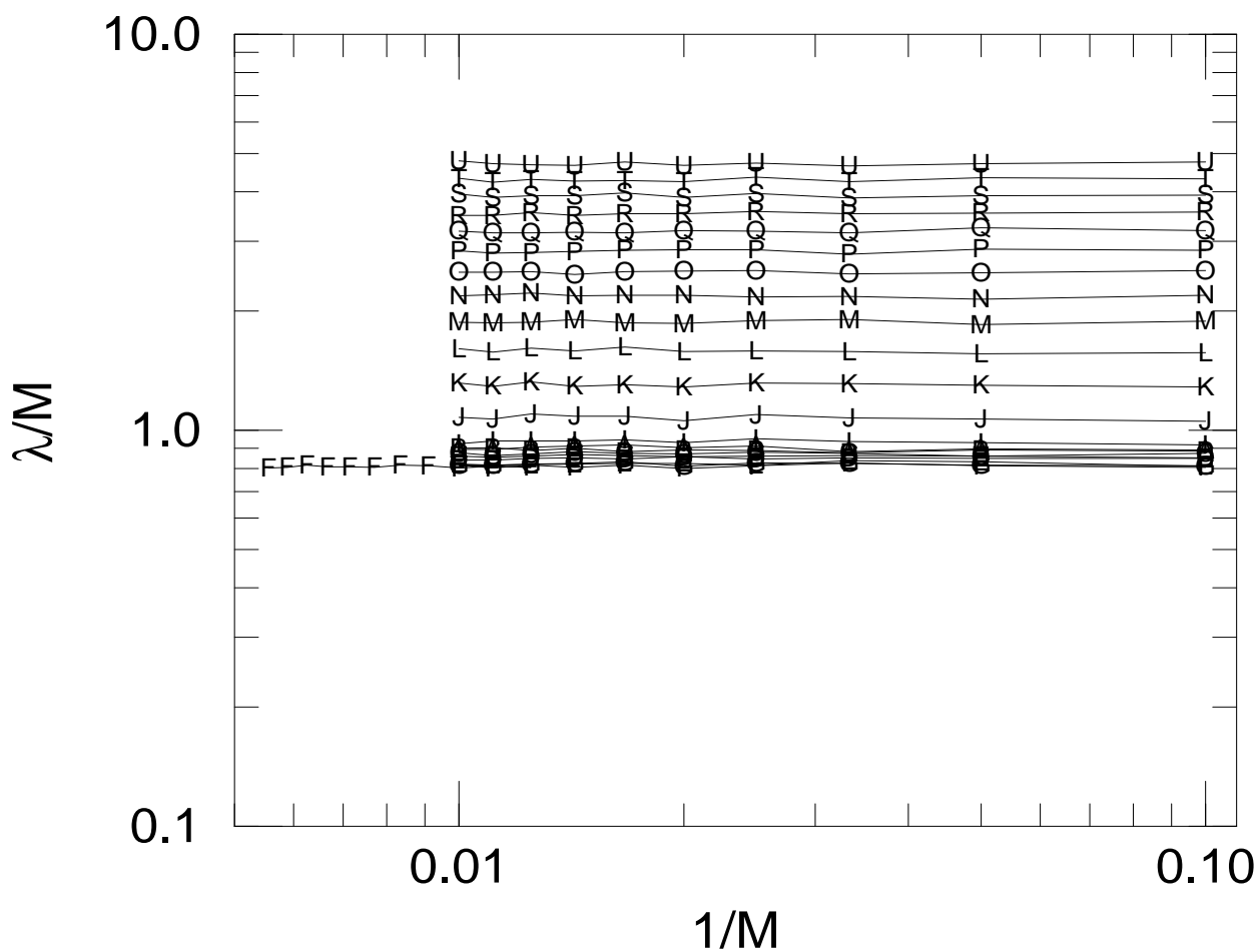
FIG. 10. Reduced localization lengths \lambda(M)/M vs. 1/M for purely random hopping ( W = 0 ) and E = 0 . The characters represent different c values as in Figs. 8 and 9. The \lambda/M scale is the same as in Fig. 8 for easier comparison. All curves are parallel to the 1/M -axis even up to M = 180 for c = 0.25 (F).
