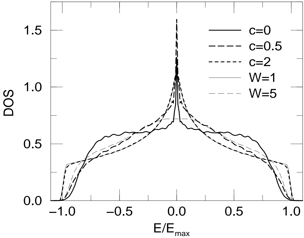
FIG. 3. Scaled density of states for purely off-diagonal disorder (thick lines, W = 0 ) and, for comparison, purely diagonal disorder (thin lines, w = 0 ).
