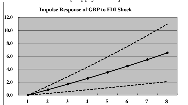
Graph 2. Impulse Responses
