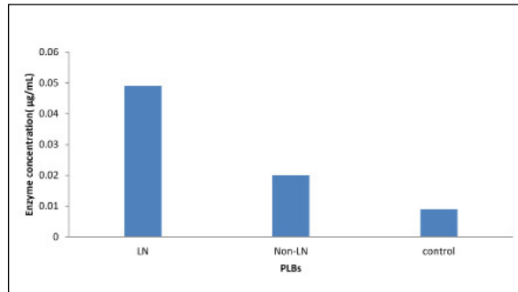
Figure 5. Effects of peroxidase enzyme of control, treated and cryopreserved PLBs of Brassidium Fly Away in encapsulation-dehydration.
