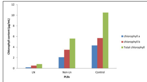
Figure 6. Effects of variuos tretaments on the chlorophyll contents of cryopreserved, treated and untreated PLBs in encapsulation-dehydration experiment.
