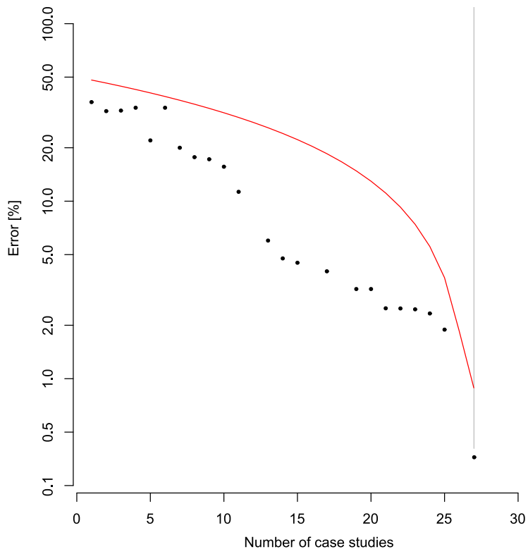
Figure 5: Average norm of the difference between the average UR distribution of a subset of n case studies and the UR distribution of all studies. The red line is the theoretical convergence for random distributions of UR.
