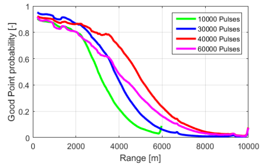
Figure 6: Averaged frequency of valid measurement points per range gate for different number of pulses.
