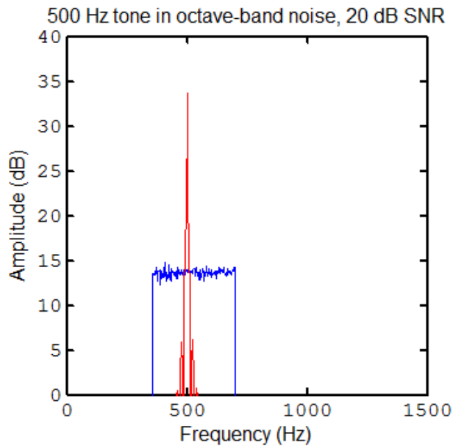
Figure 1. Example output of a fast Fourier transform illustrating how the signal-to-noise ratio was calibrated using Spectrum level (Lps), rather than RMS dB SPL. This calibration method follows the frequency-discrimination-in-noise methods in the literature (e.g., Dye and Hafter, 1980).
