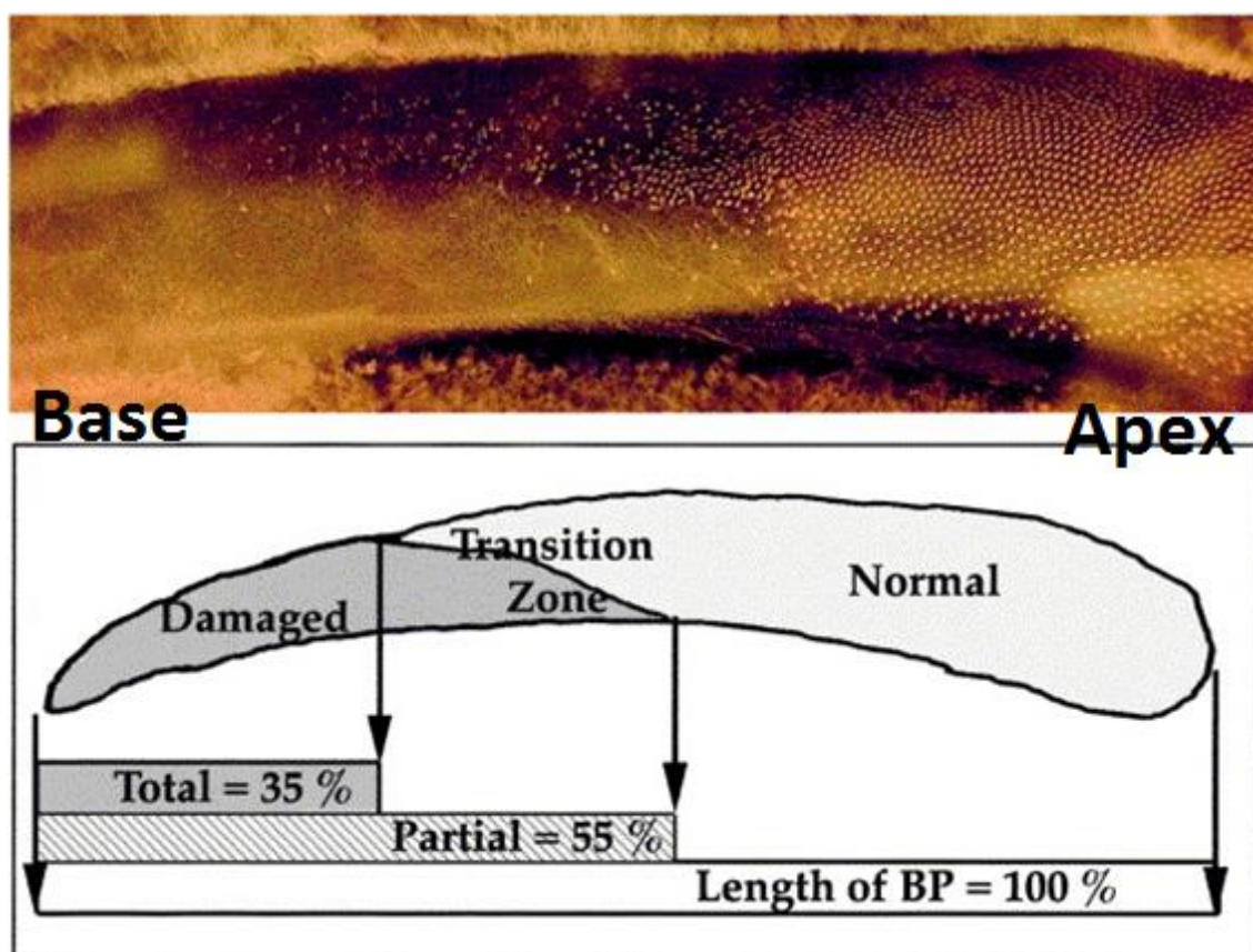
Figure 12: Basilar papilla of a chick following a single, large injection of gentamicin. Images taken from Roberson, Alosi, Messana, & Cotanche, 2000.
