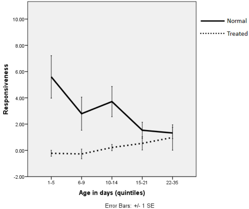
Figure 5: Age vs. Responsiveness to high frequencies in the 31-37 dBQL range.
