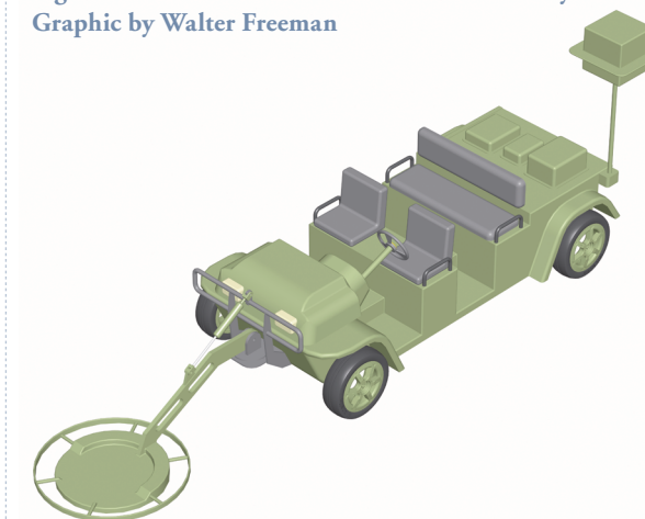
Figure 3: Vehicle-mounted landmine-detection system. Graphic by Walter Freeman
