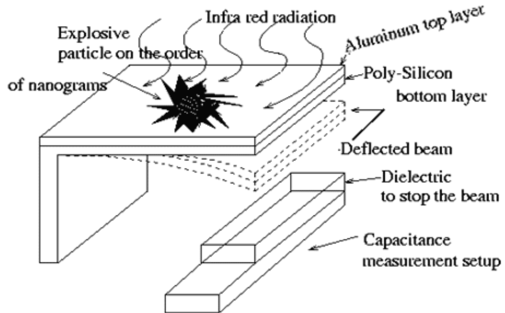
Figure 8: Schematic of MEMS trace explosive particle detector (V. Pamula, Duke (Fai97))
