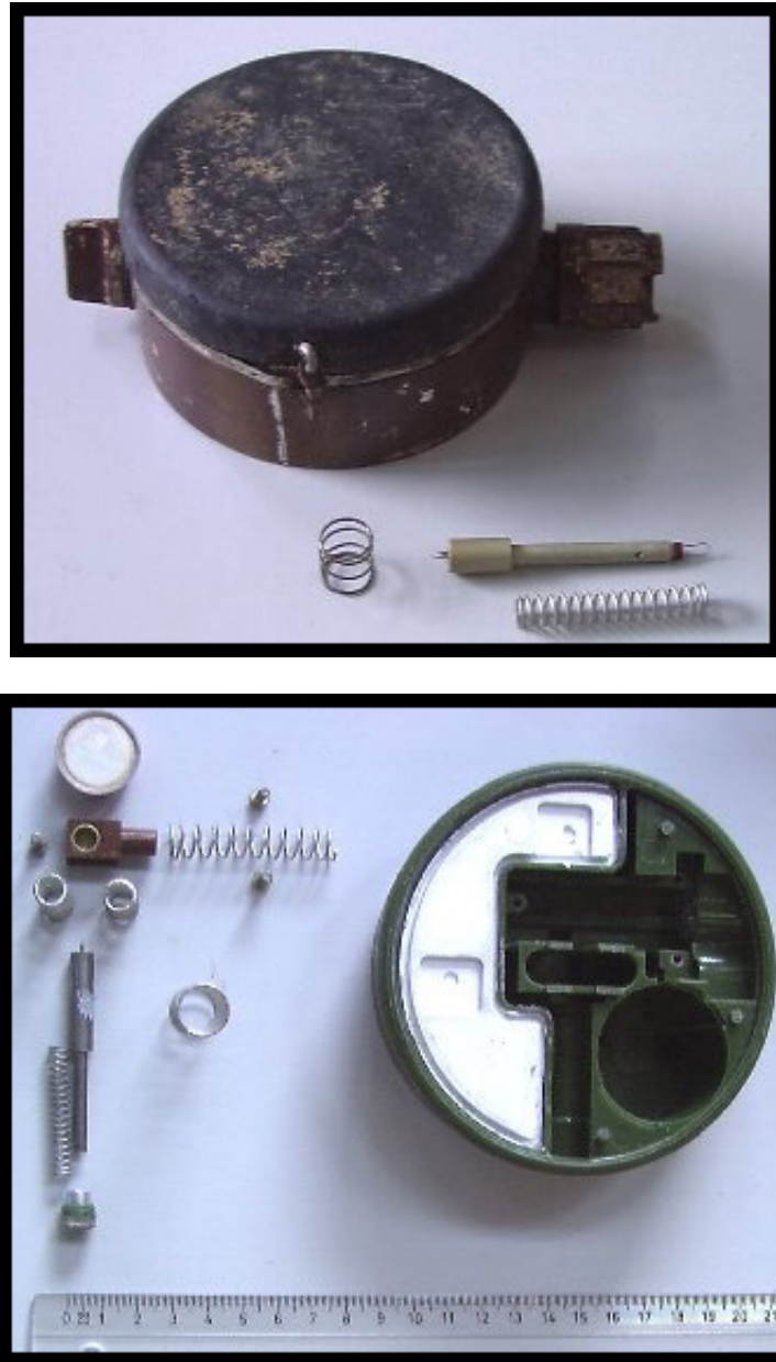
Figure 2: Metallic content of a PMN AP (top) and a PMN2 AP (bottom)
