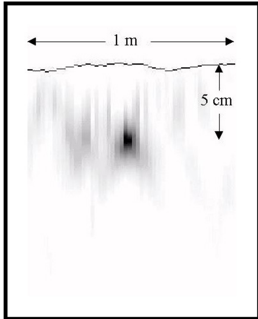
Figure 12: Line scan of a plastic AP using 1 msec acoustic pulses (C. Don, Monash Univ.)
