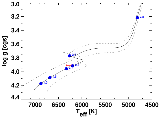
Figure 11. Theoretical H-R diagrams based on the YY stellar evolution models (Demarque et al. 2004). The red cross shows the values of and 1\sigma uncertainties on T_{\text{eff}} and \log g_* from the adopted global fit in Table 4. The black curve shows the best-fit evolutionary track, while the dashed lines show evolutionary tracks for the 1\sigma uncertainties on [\text{Fe}/\text{H}] and M_* . The blue filled circles denote the \log g_* and T_{\text{eff}} for KELT-12 at the listed ages (in Gyr).
