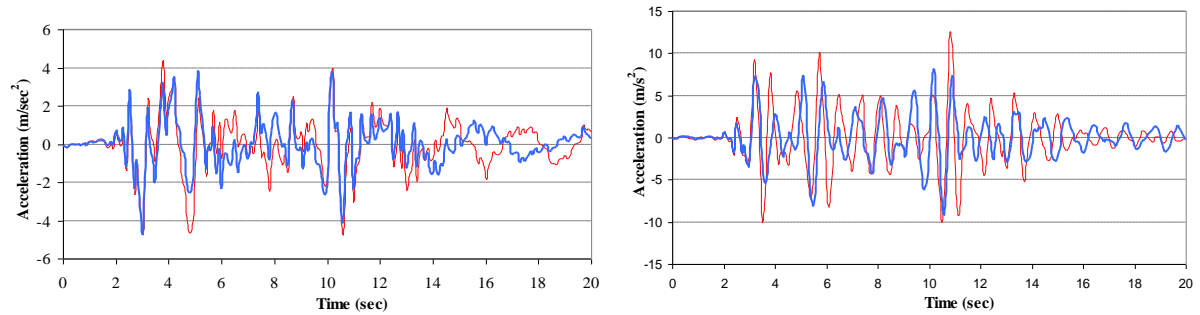
Figure 13. Time history Acc_{x,J49} , Acc_{y,J49}
