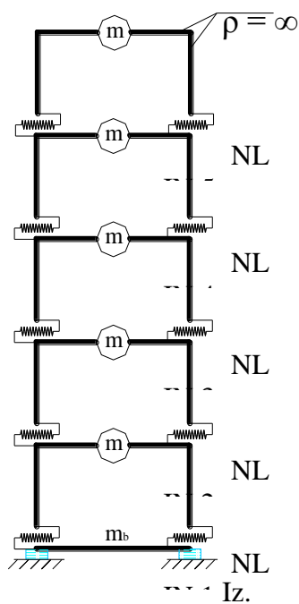
Figure 6: Elasto-plastic (nonlinear) model of base isolated frame
