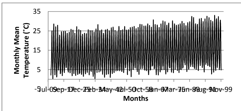
Figure 7: Monthly mean temperature between the years of 2007-2010 for A2 scenario
