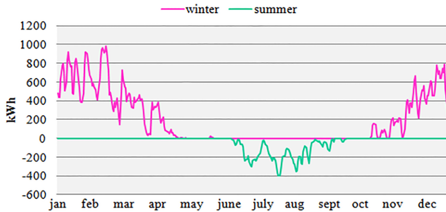
Figure 3: Trend of building energy need during the year
