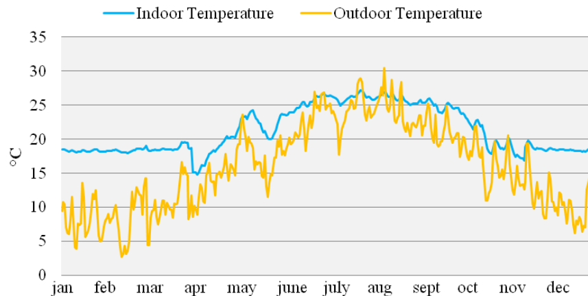
Figure 2: Trend of indoor and outdoor temperature during the year.
