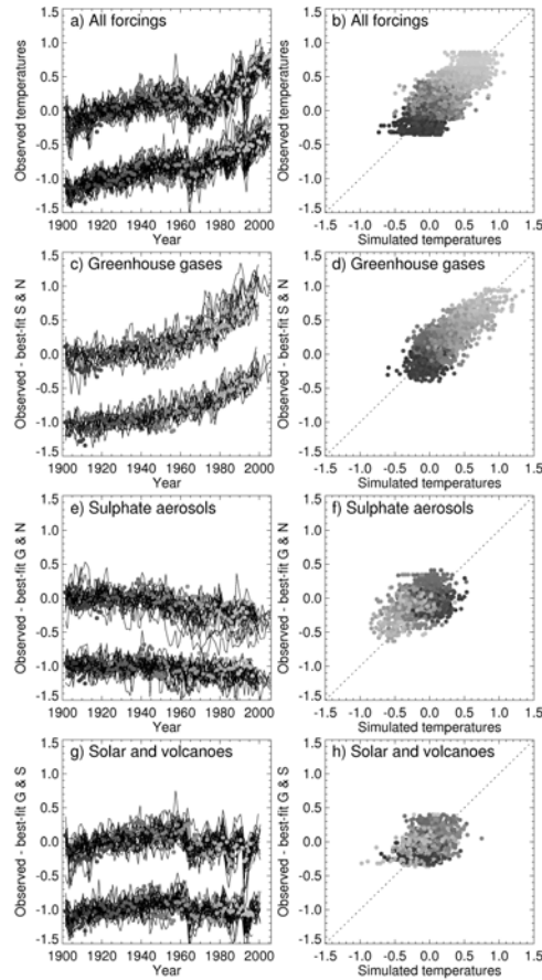
Figure 3: A simple attribution analysis, comparing model simulations with observed temperature changes over the twentieth century. (a) Grey dots: Observed Northern and Southern Hemisphere area-averaged near-surface temperature anomalies during the period 1901-2005 relative to average temperatures between 1900-1940. Grayscale indicates time, with lighter being more recent. Black lines: Corresponding simulated temperatures from six of the models shown in Figure 1 driven by the combination of GHG increase, anthropogenic sulfate aerosols, and natural (solar and volcanic) variability. Southern Hemisphere points are offset by 1^{\circ}\text{C} . (b) Same data, plotting model simulations (horizontal) against observations (vertical). Grayscale indicates time, as
