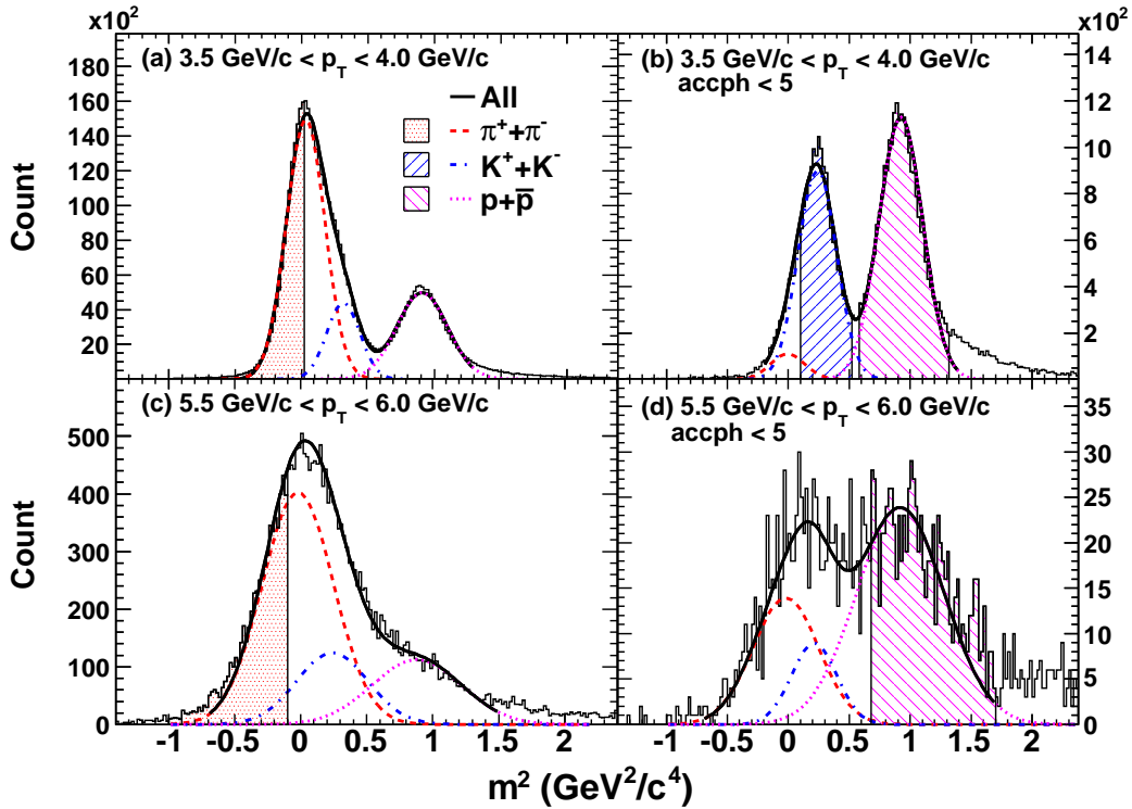
FIG. 4: (color online) The mass-squared distribution in the TOFw without (left panels) and with (right panels) the ACC photon yield ( \text{accph} ) cuts for different p_T regions. The hatched areas show the m^2 cuts used for pion, kaon, and proton selections. The distribution is fit with a 3-Gaussian function (solid line). The individual Gaussian distributions corresponding to \pi , K , and p are as dashed lines.
