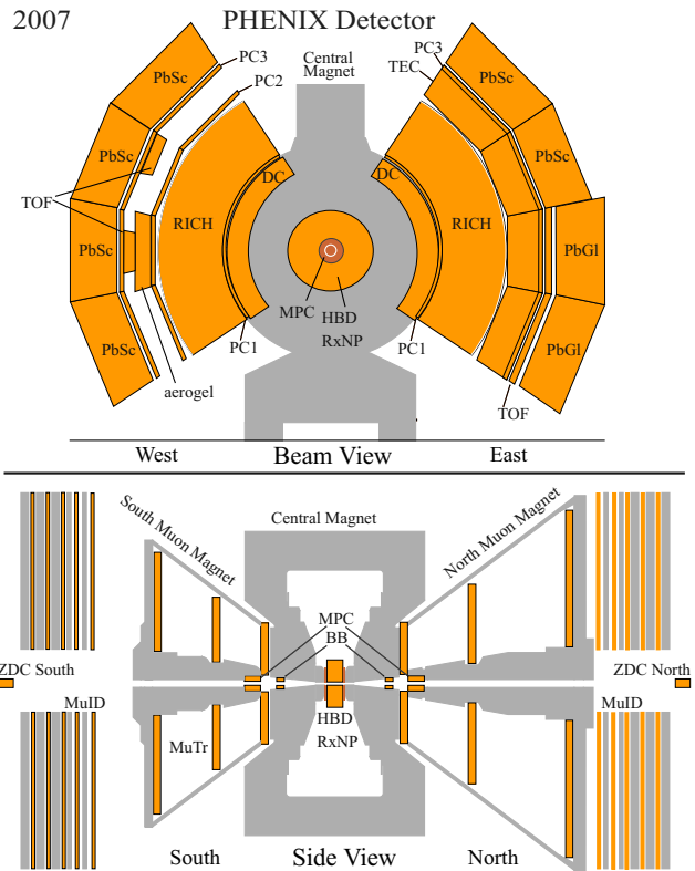
FIG. 1: (color online) The PHENIX detector configuration for RHIC 2007 data-taking period. The beam-beam counters (BBC) are labeled as BB.
