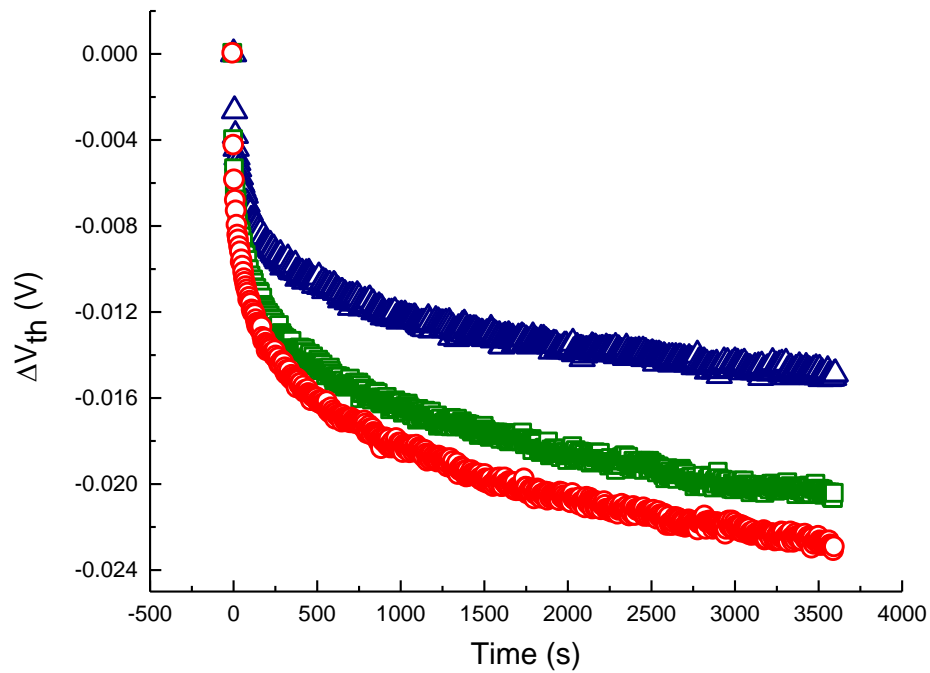
Figure 4-4) Threshold voltage shifts resulting from NBTI as determined from continuous bias method for T=95C (Δ), T=125C (□), T=155C (O). Gate dielectric stack was high-κ HfSiON
