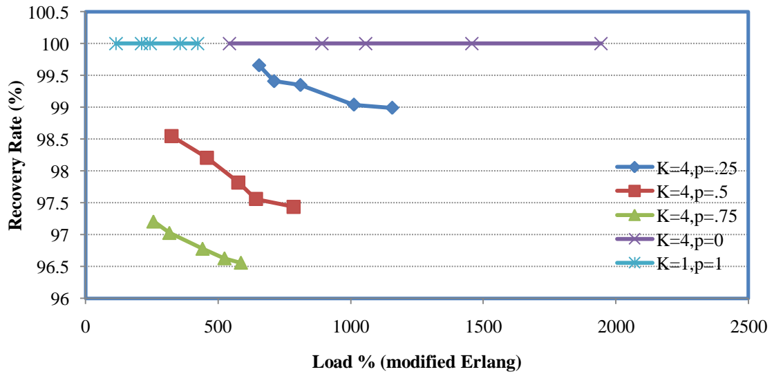
Figure 5.12: LAN restoration for MST overlay and load-balancing (MAC) routing
