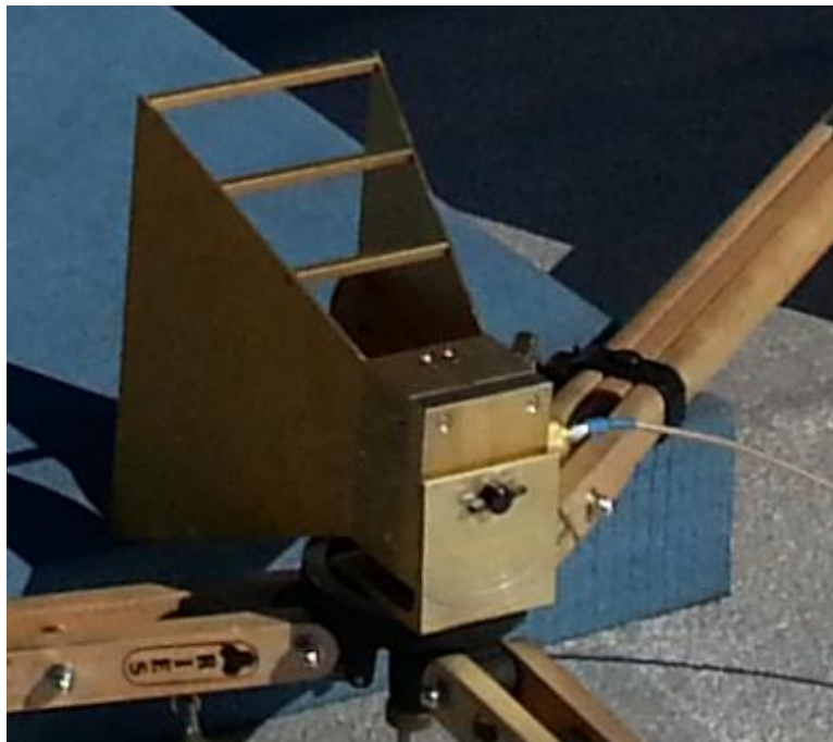
Figure 5.11: Orientation of the standard gain horn antenna in Figure 5.7.
