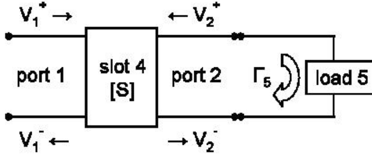
Figure 3.3: Illustration for the first step in the path analysis.
