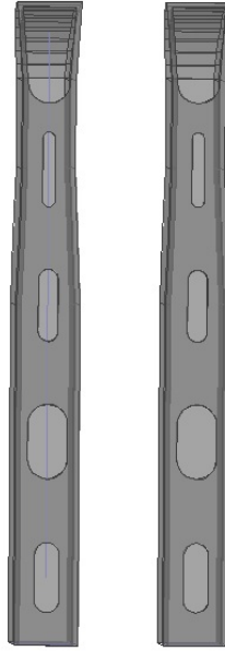
Figure 4.19: Beamsteering mechanism of the narrow-wall longitudinal-slot array.
