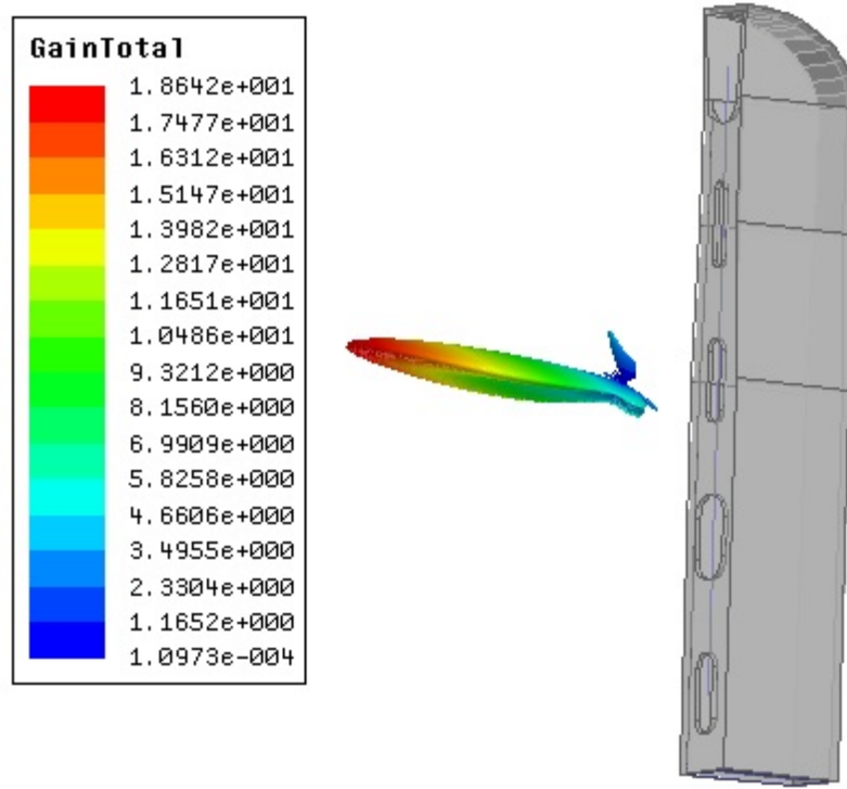
Figure 3.7: slot array along with its 3-D absolute antenna gain in dimensionless units.
