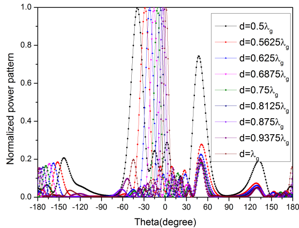
Figure 4.14: H-plane radiation pattern for different element distance d .
