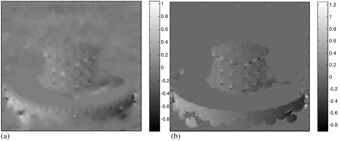
(a) (b) Figure 4.35. Vertical velocity estimates for the Rubik's cube sequence. (a) Horn's estimates. (b) Lucas's estimates.
