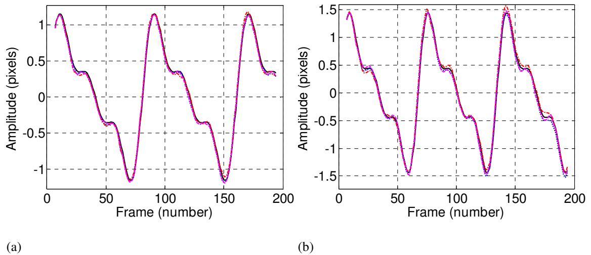
(a) (b) Figure 5.9. Lateral (a) and axial (b) trajectory reconstructions of three selected points of Figure 5.8. Ground truth is shown in solid black line. Point 'x' is shown on a blue '.' line, point '+' shown on a red '-. line', and point '*' shown a magenta '-- line'.
