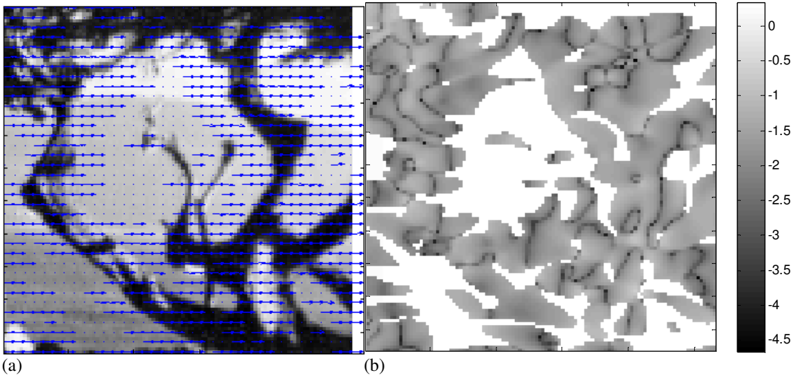
Figure 3.23. Lucas's method results on the Translating Tree sequence. (a) Estimated velocity field and (b) logarithmic plot of the velocity magnitude error
