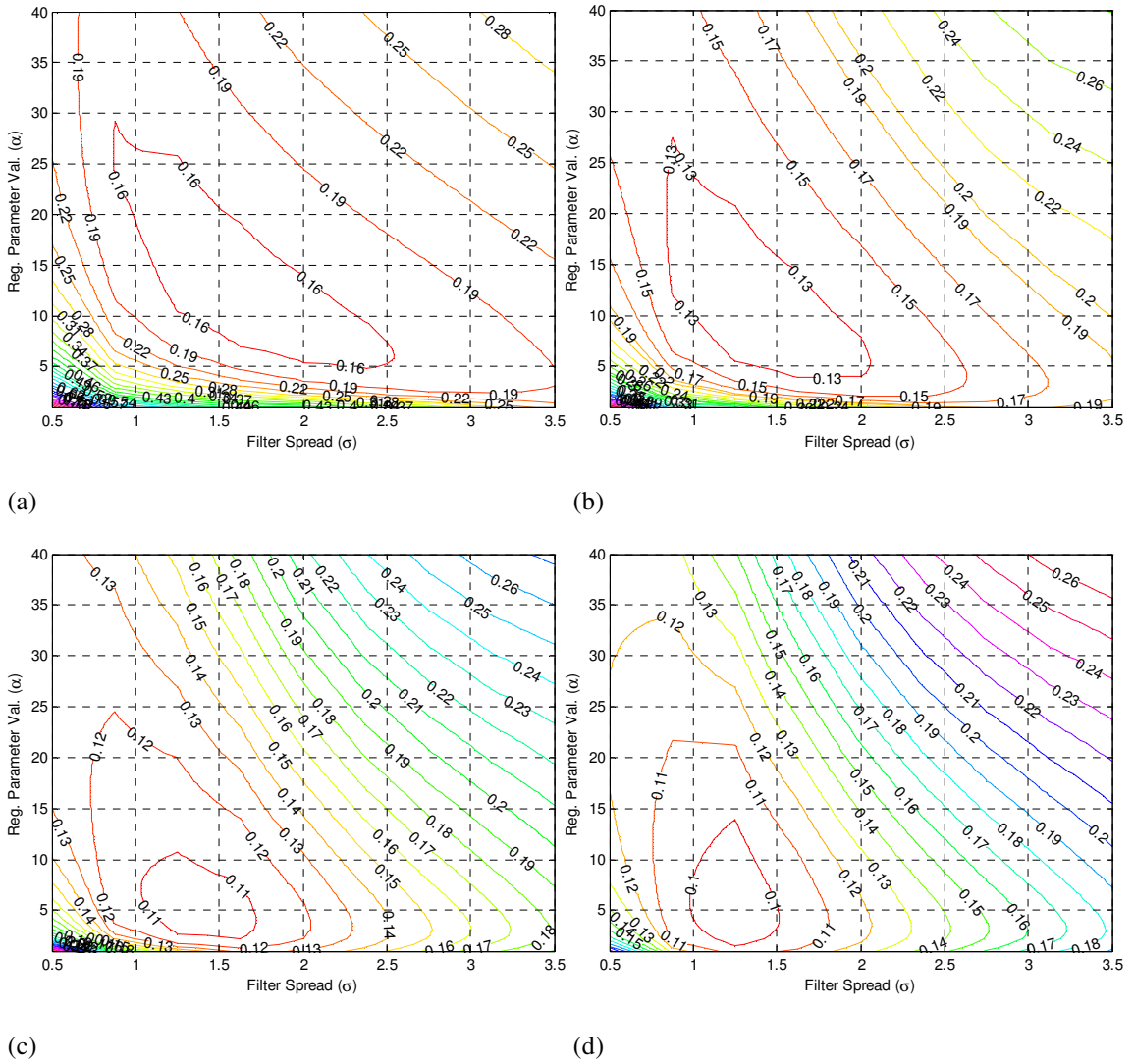
(a) (b) (c) (d) Figure 5.5. Contour plots of the relative error for speckle simulations of SNR =10dB (a), 20 dB (b), 30 dB (c), and 40 dB (d). Compared to noise free cases, higher regularization parameters and filter spreads are necessary to obtain reliable velocity estimates.
