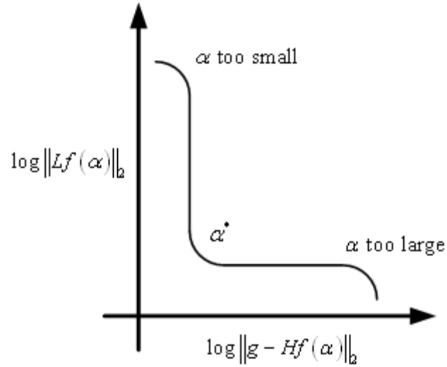
Figure 3.2. Shape of the L-curve. The optimal regularization parameter \alpha^* is the one that corresponds to the corner of the curve.
