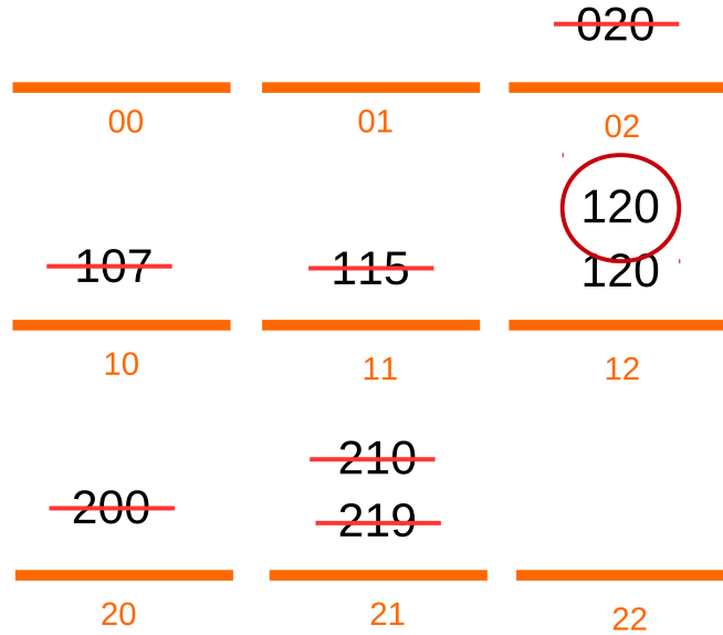
Figure 5.3: Example step 3. The previously selected configurations are discarded and the repeated configuration 120 is the last available one.
