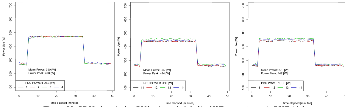
Figure 22: PDU plots during PV2; air cooled (left), 65°F water (center), 75°F (right).
