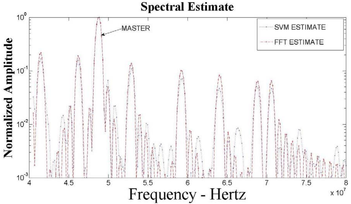
Figure 3.46: Amplitude Difference Estimate, Channel 7 @ 15 dB below Master
