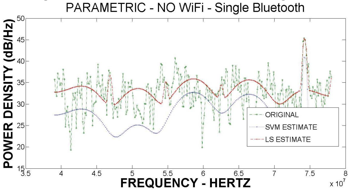
Figure E.13: Parametric Estimator, Channel 70, A+I, Sigma = 5
