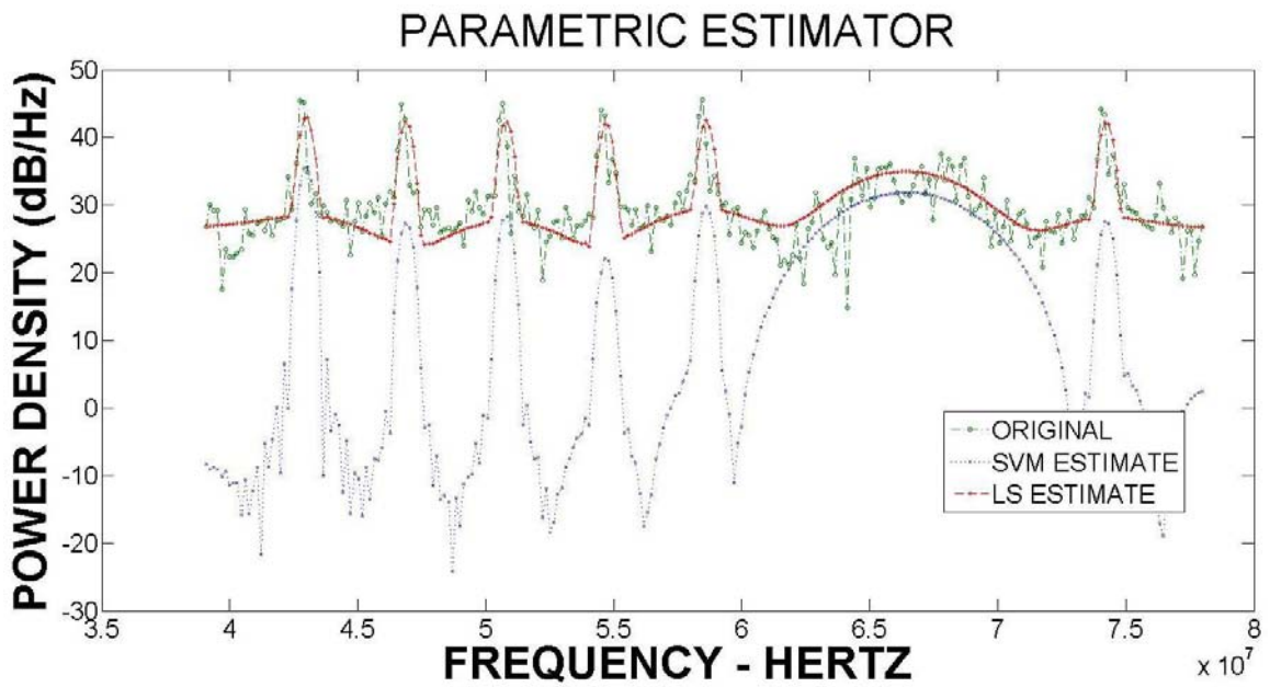
Figure 3.41: Parametric, WiFi And Six Bluetooth, AWGN, Sigma = 1
