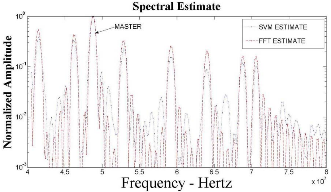
Figure 3.44: Amplitude Difference Estimate, Channel 7 @ 9 dB below Master
