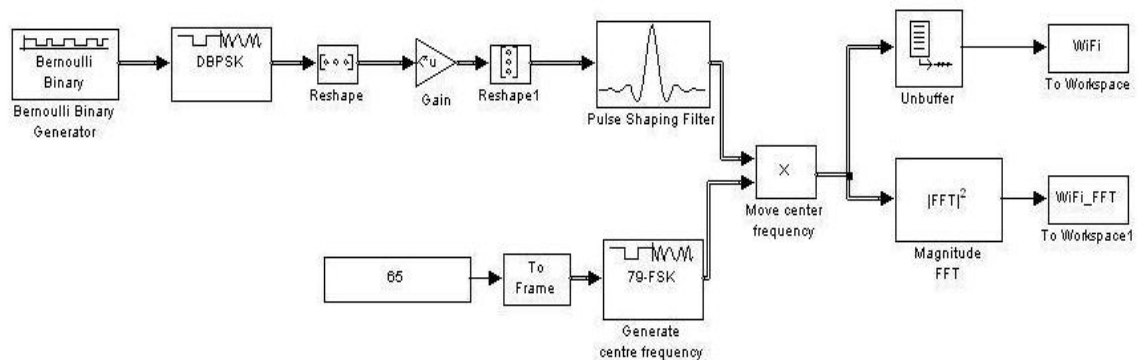
Figure 3.11: 1 Mbps WiFi Transmitter Simulink Model
