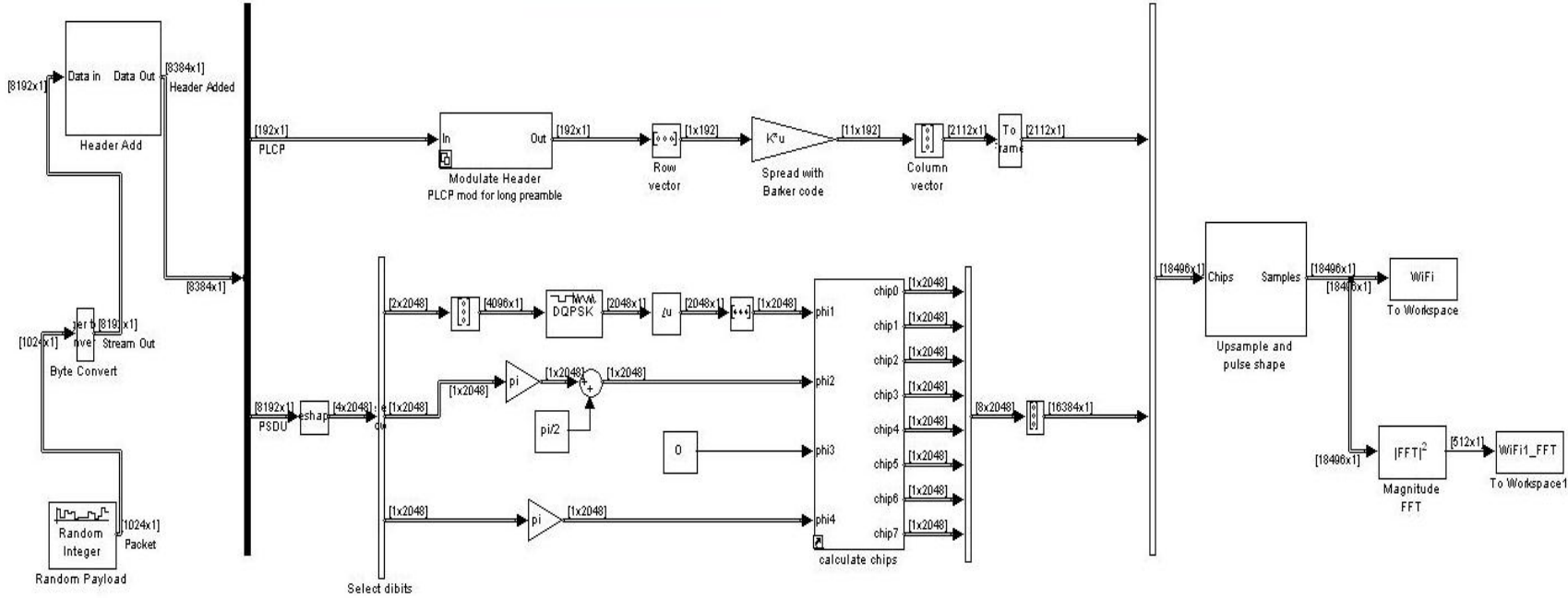
CCK Spreading
