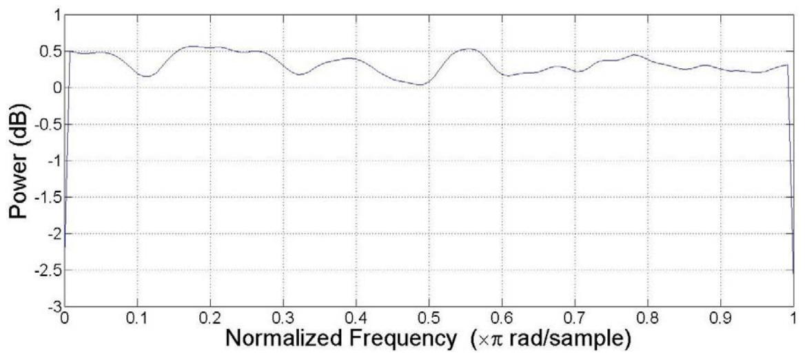
FIGURE C.10: MEAN SQUARE SPECTRUM, AWGN+IMPULSIVE+BLOCK, SIGMA = 5
