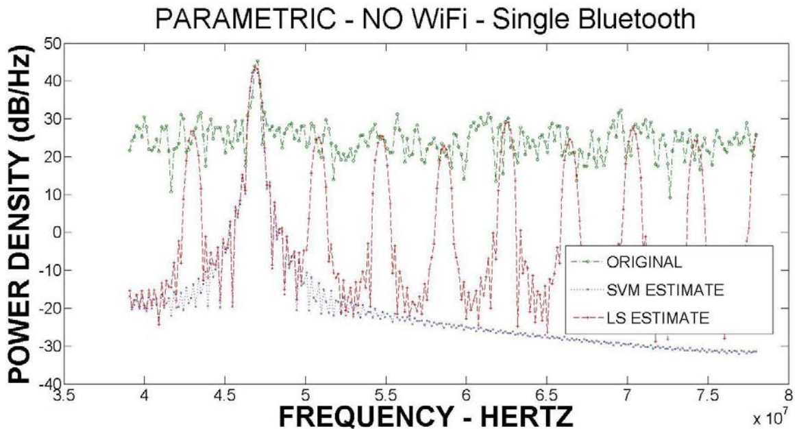
Figure 3.10: Parametric Estimator – Channel 42 – AWGN, Sigma = 1
