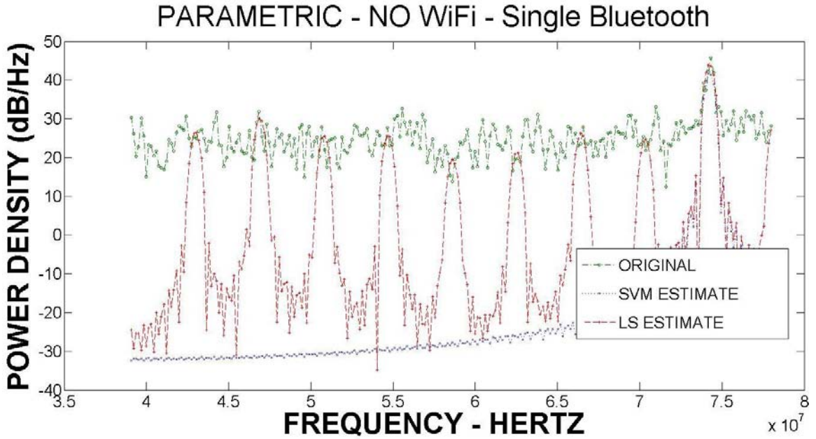
Figure E.7: Parametric Estimator, Channel 70, A+B+I, Sigma = 1
