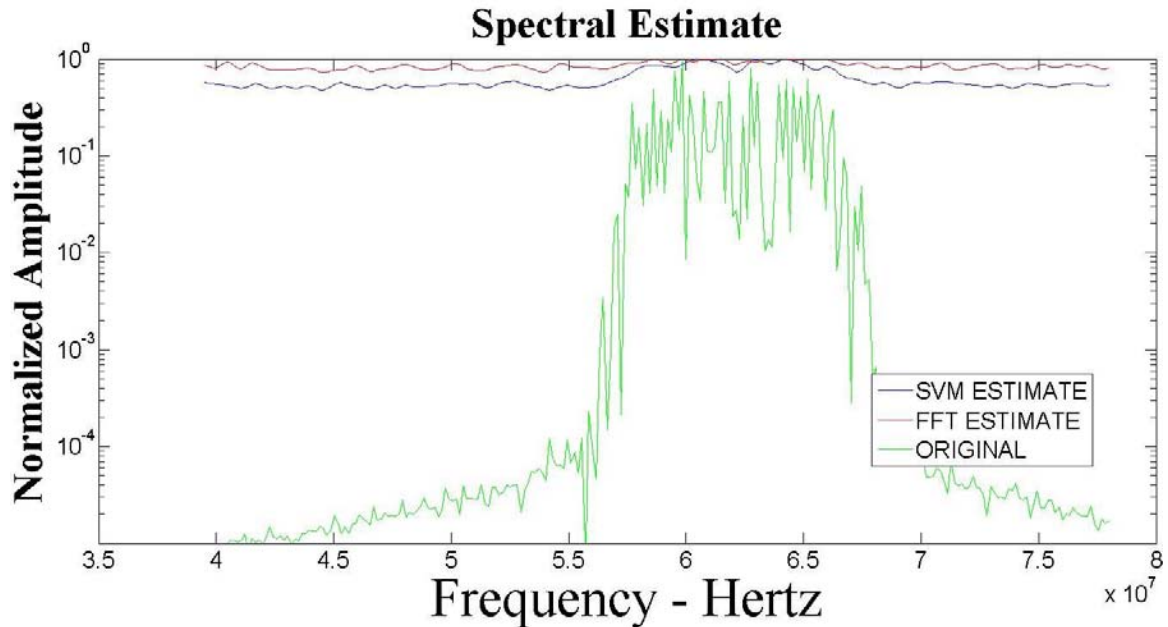
Figure 3.15: Spectral Estimate, AWGN + Block + Impulse, Sigma = 1
