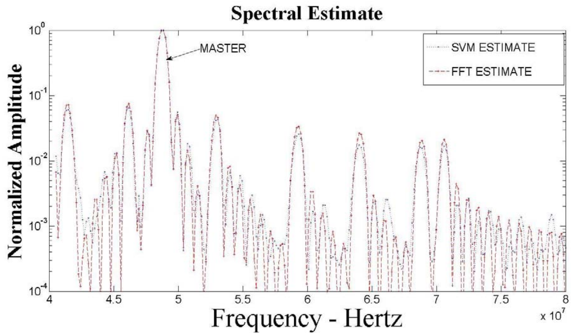
Figure 3.47: Amplitude Difference Estimate, Channel 7 @ 18 dB below Master
