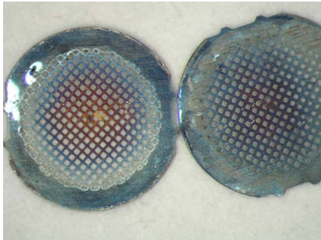
Figure 93 Optical microscope image of TEM grids after experiments of Ni/MgAl 2 O 4 heated to 750°C at 1:1 H 2 :H 2 O 3.6mbar. The left grid is from an experiment using the spacer ring, while the grid on the right used the two 50 mesh grids.
