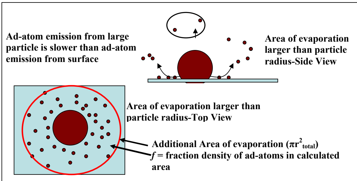
Figure 25 Schematic of a particle and the surrounding area occupied by adatoms on the surface.
