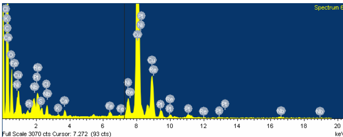
Figure 43 Spectrum of a 10wt% PtRe on Norit Carbon after reaction at low magnification, carbon particles \sim 5\mu\text{m} in size.
