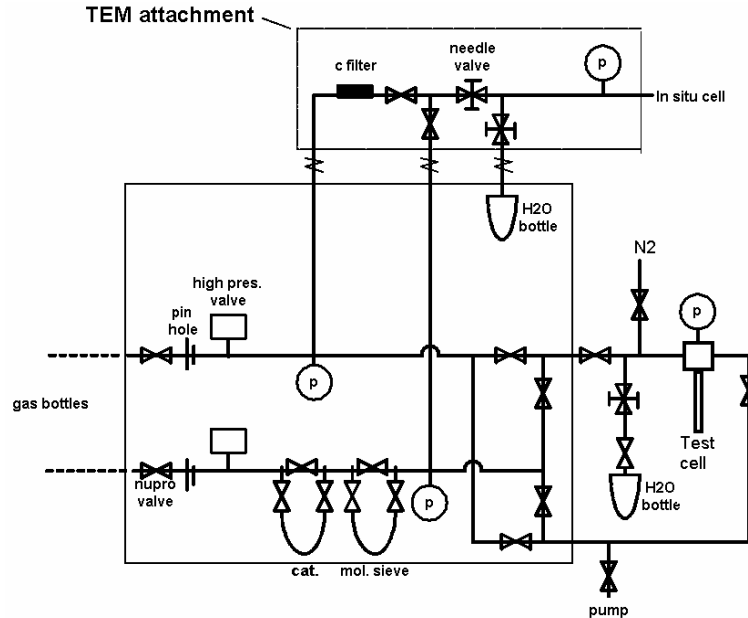
Figure 15 Schematic of the gas inlet system prior to the TEM microscope inlet. The lower inlet without the carbonyl filter was path of primary use.
