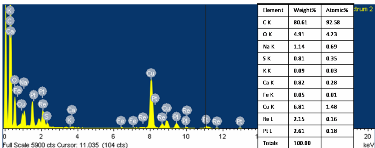
Figure 40 Spectrum of a carbon particle ~5µm in size on the 10wt% PtRe Vulcan Carbon Sample after reaction. Many elements are detected.
