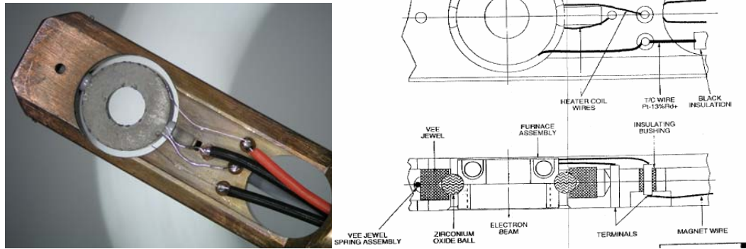
Figure 16 Image and Schematic of the GATAN sample holder used for heating in-situ experiments. The sample, which is on a TEM grid, is placed in the cup and secured with a spacer ring.
