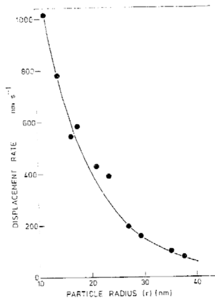
Figure 8 The particle displacement vs. particle radius for Iron particles on graphite at a temperature=740°C. Provided by Baker[25].
