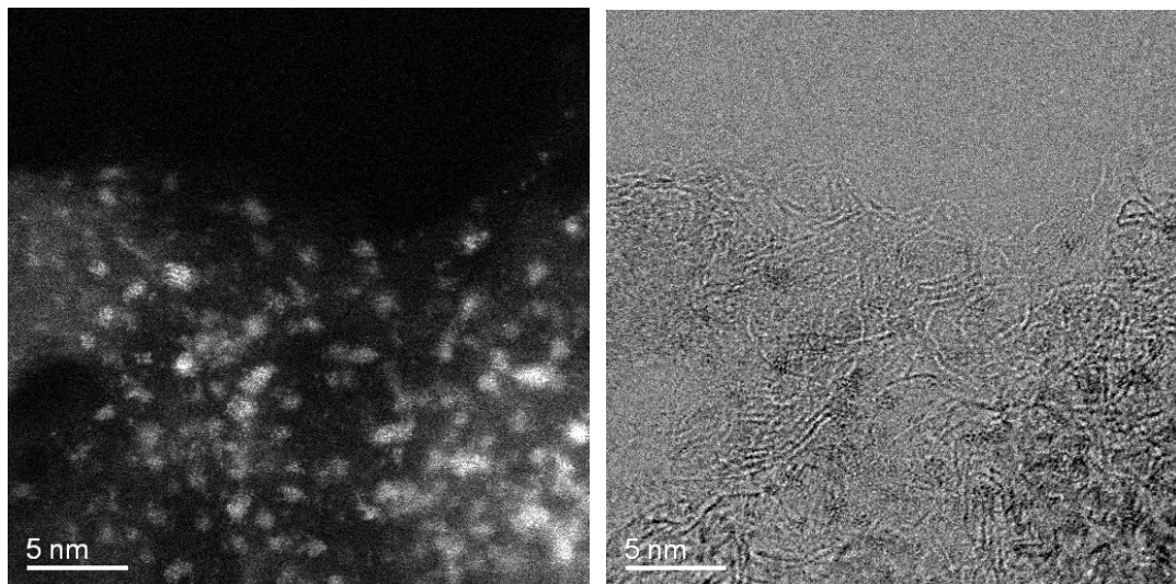
Figure 33 10wt% PtRe on Norit Carbon: The Dark Field Image (left) and Bright Field Image (right) reveal the homogeneously dispersed PtRe particles as well as the carbon structure.
