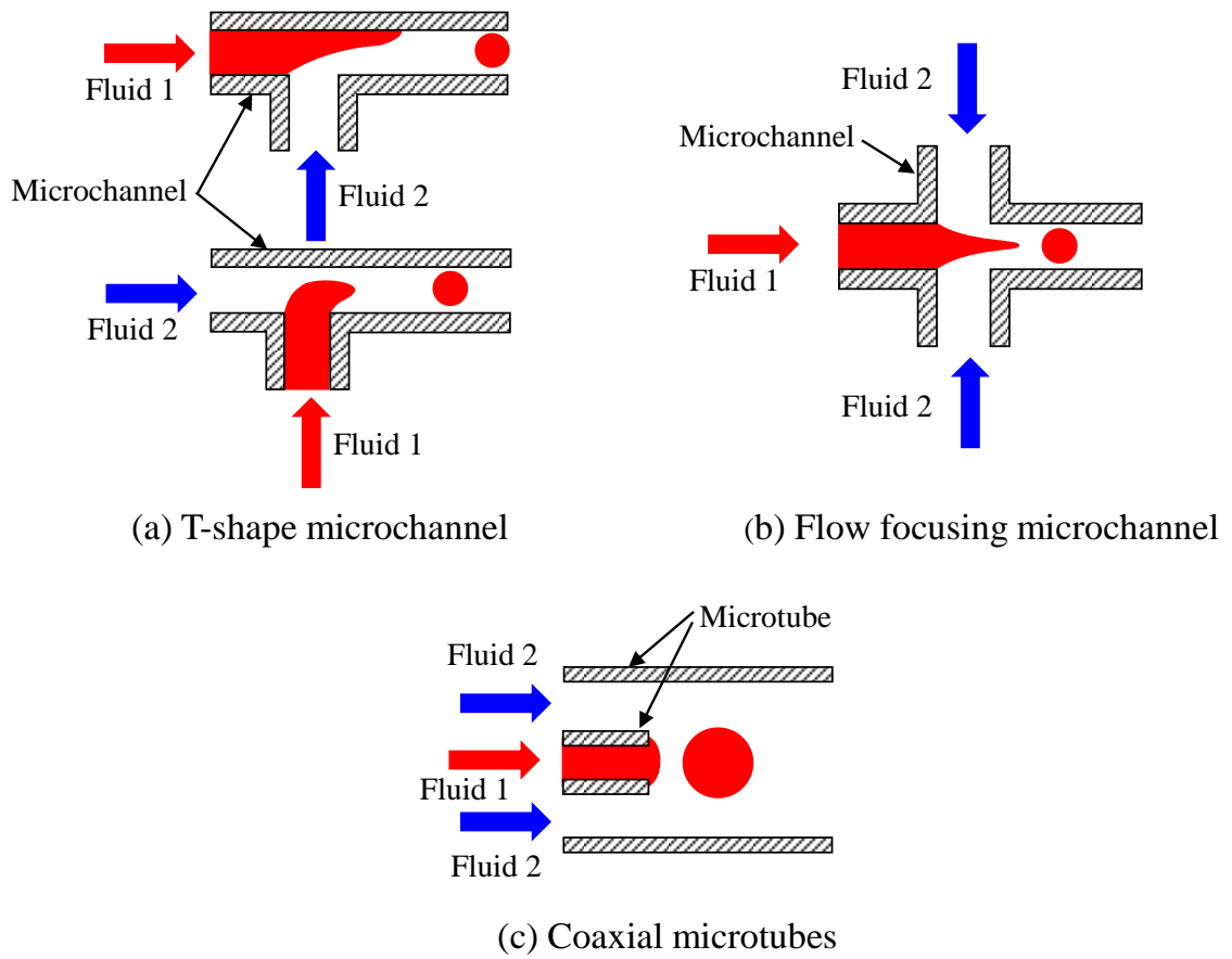
Figure 1.3. Schematic diagrams of different co-flowing emulsion generators: T-shape microchannel (a), flow focusing microchannel (b), coaxial microtubes (c).
