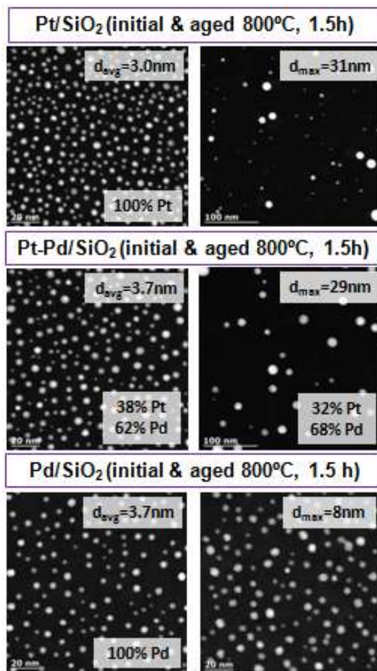
Figure 27. HAADF-STEM images of Pt, Pt-Pd, and Pd/SiO 2 before and after aging at 800°C for 1.5 hr. The mean diameters are provided for the catalysts in the initial state. The maximum particle size is provided for each sample after aging.
