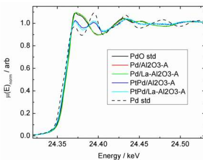
Figure 5(c). XANES at the Pd edge showing that the Pd-only catalysts are fully oxidized while the bimetallics show Pd to be partly oxidized, even after aging at 750°C in air for 10 hours. This plot shows both supports.
