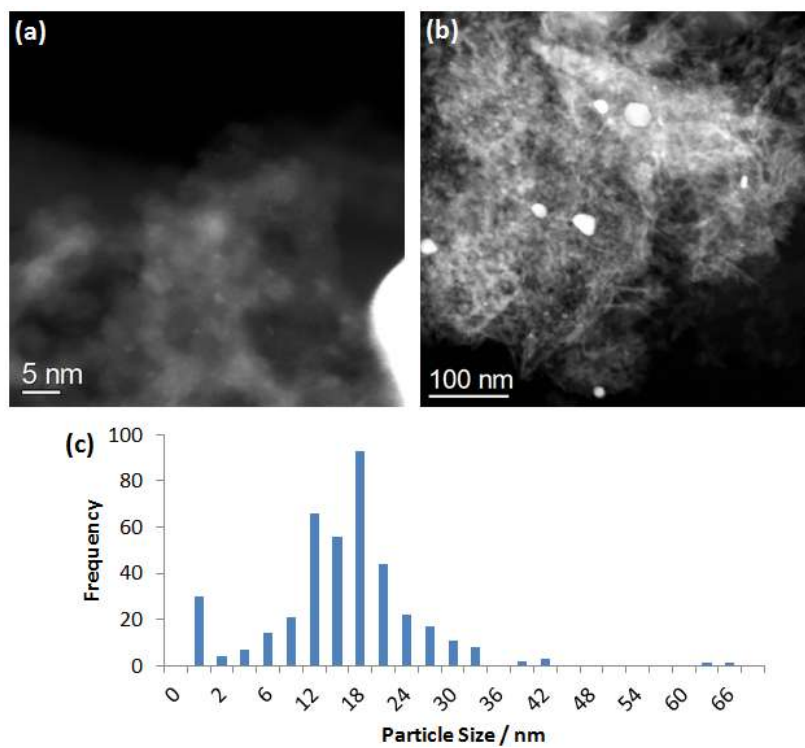
Figure 11. STEM image of (a) dispersed phase and (b) large particles in the aged plus reduced Pt-Pd/La-Al 2 O 3 catalyst; (c) particle size distribution.
