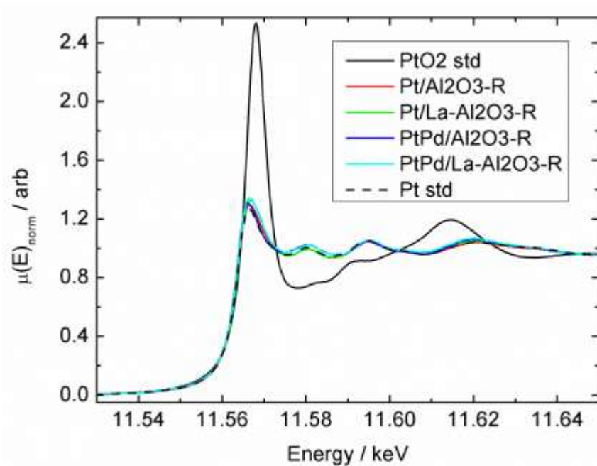
Figure 6(d). XANES at the Pt edge after H 2 reduction shows very little change compared to the aged samples, confirming that Pt stays metallic when treated in air at 750°C. This plot shows both supports.
