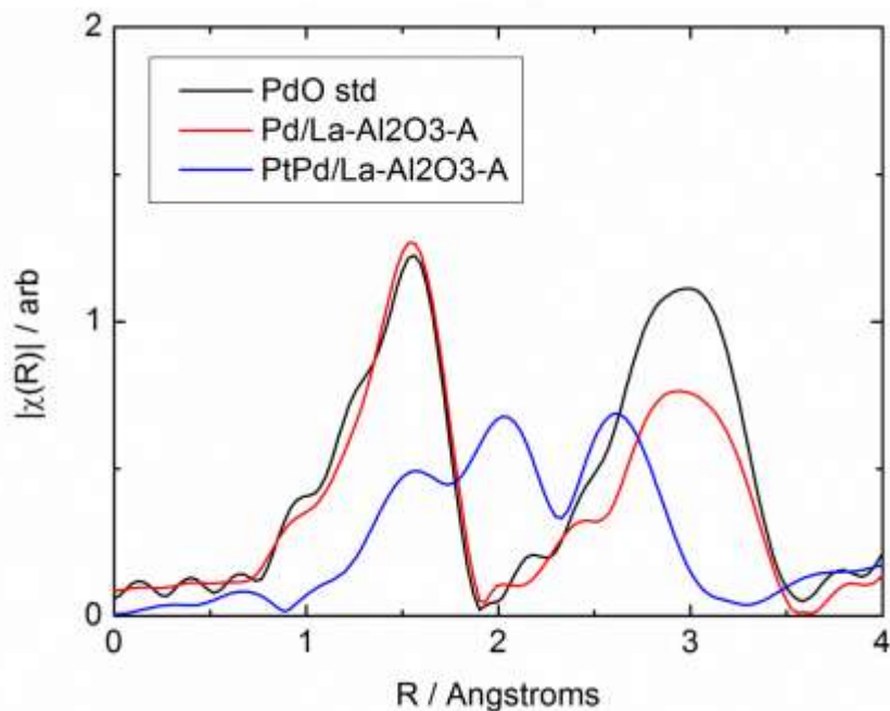
Figure 8(a). Fourier Transform EXAFS Pd K edge results for the aged samples. The monometallic samples show peaks corresponding to Pd-O and a second shell Pd-Pd. The lower amplitude for the second shell is consistent with small, dispersed, PdO on the surface of the catalyst. In contrast, the bimetallic sample shows peaks consistent with Pt neighbors as well as Pd neighbors for metallic Pd and only the first shell oxide, suggesting that the oxide is now a dispersed phase.
