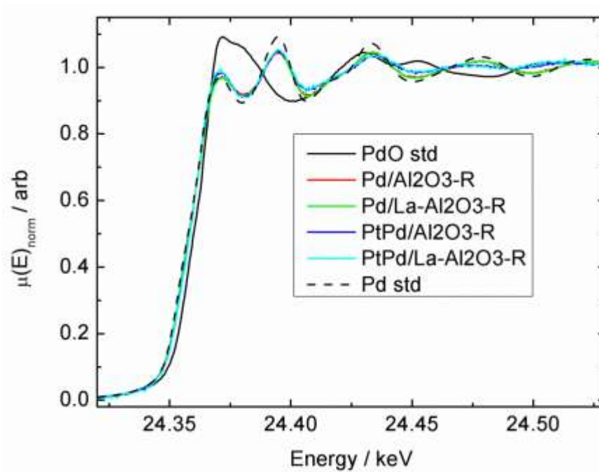
Figure 5(d). XANES at the Pd edge after reduction in H 2 , showing that the Pd is almost fully reduced in all catalysts. This plot shows both supports.
