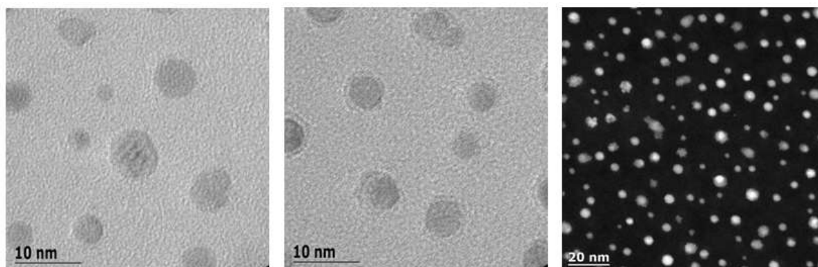
Figure 22. HR-TEM and HAADF-STEM images showing that the Pd sample after being aged at 650°C for 2 min is not fully oxidized.
