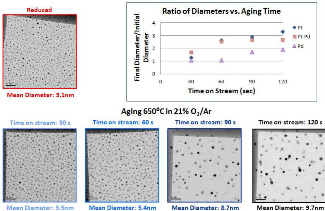
Figure 35. Aging sequence of Pd/SiO 2 showing the sample in its reduced state as well as after a total time-on-stream of 30s, 60s, 90s, and 120s at 650°C in 21% O 2 /Ar to simulate air. The average diameters are provided during each step of the aging process.
