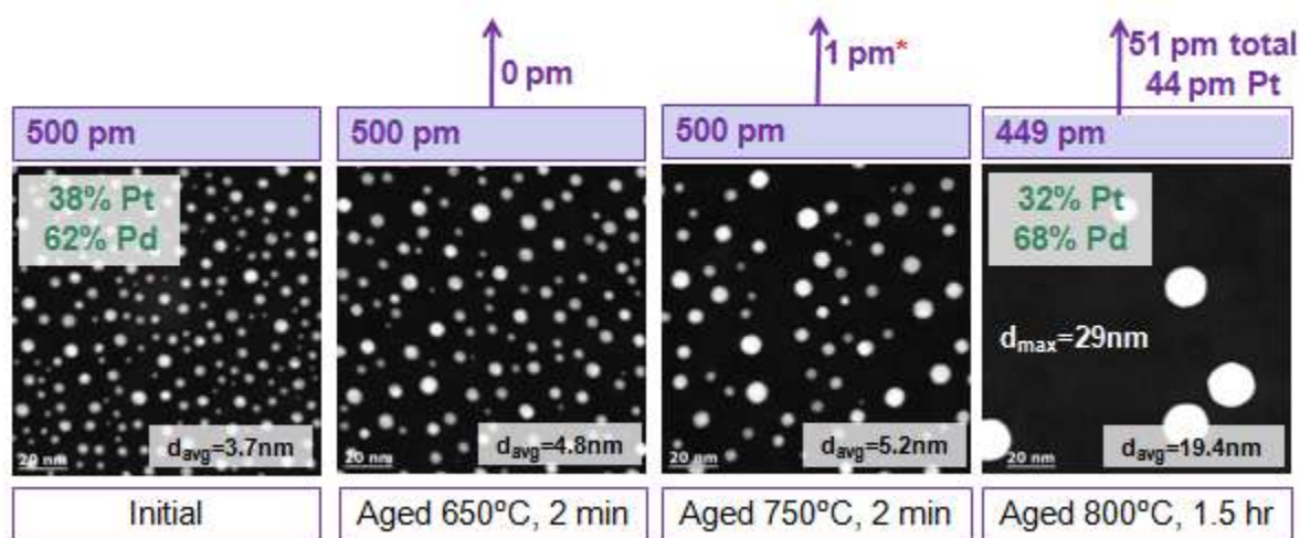
Figure 24. Effect of aging conditions on Pt-Pd sintering and emission in air. (* means estimated from extrapolation.)
