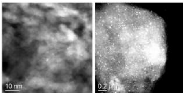
Figure 47. STEM image of (a) dispersed phase and (b) large particles in the aged plus reduced Pt-Pd/La-Al 2 O 3 catalyst.
