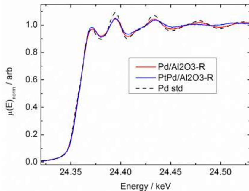
Figure 5(b). XANES at the Pd edge after reduction in H 2 , showing that the Pd is almost fully reduced in all catalysts.
