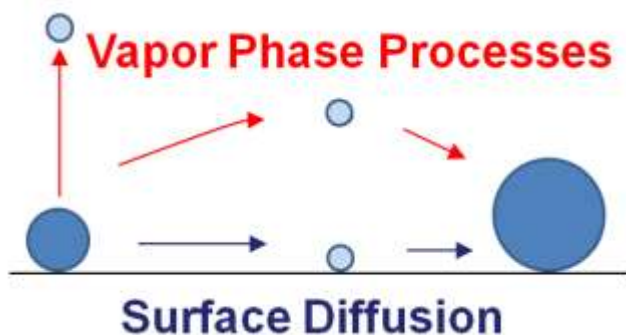
Figure 16. Schematic showing phenomena that could be responsible for Ostwald ripening of a Pt catalyst in air. The vapor phase process is shown in red, and the surface diffusion process is shown in blue. In addition to interparticle transport, it is also possible to emit atoms into the vapor phase, which can be detected by the change in mass of these model catalyst samples.
