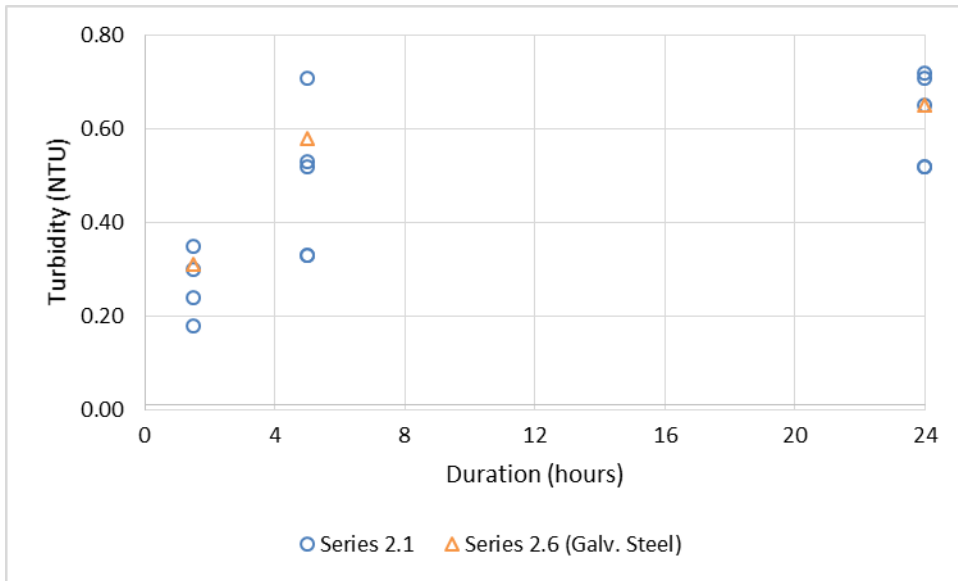
Figure 32. Theme 2 turbidity
