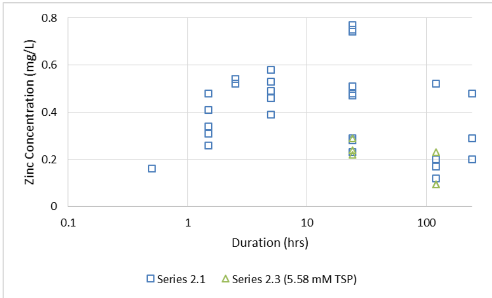
Figure 28. Series 2.3 zinc release
