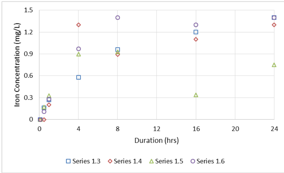
Figure 17. Theme 1 iron release
