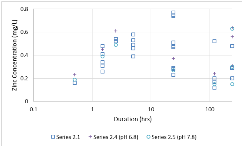
Figure 29. Series 2.4 and 2.5 zinc release
