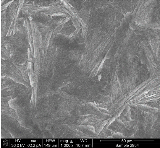
Figure 60. Series 5.3 SEM image after descaling with ammonium acetate
