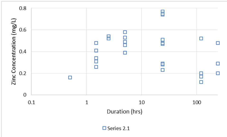
Figure 26. Series 2.1 zinc release
