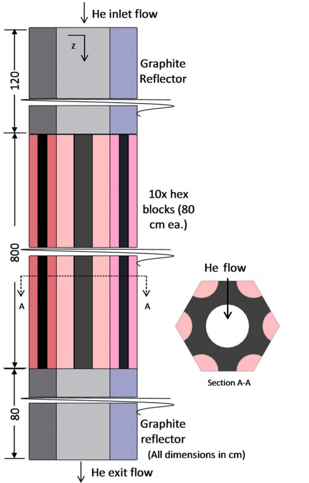
Figure 4.1 - Axial isometric view and a radial cross-section of the single channel fuel module.
