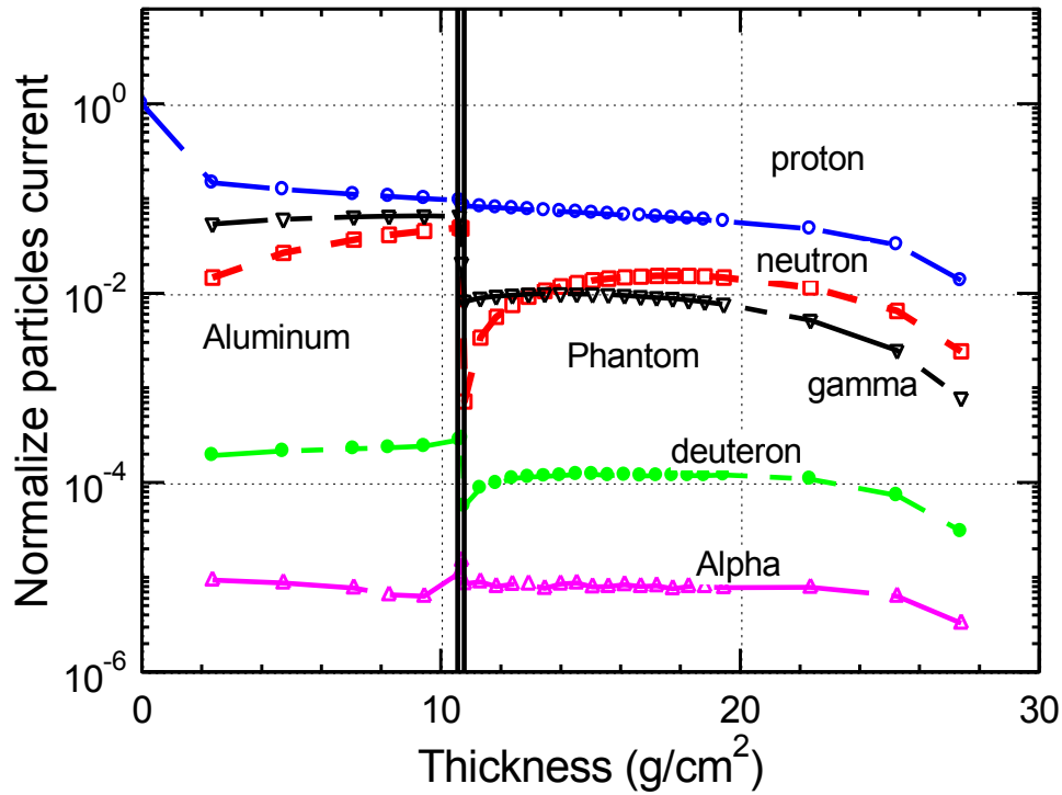
Figure 4.4. Primary and secondary particles for 10.5 \text{ g/cm}^2 aluminum and center seeking incidence mode.
