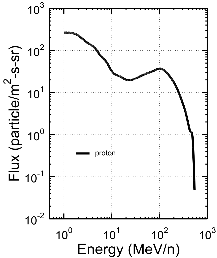
Figure 2.3. Fluxes of trapped protons for apogee 364 km, perigee 347 km, and inclination of 52° [Tylka et al. 1997].
