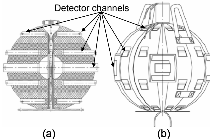
Figure 7.2. Schematic of the MATROSHKA-R phantom (a) cross-section view of phantom showing detector channel (b) phantom covered with working jacket [Akatov et al. 2007; Shurshakov et al. 2008].
