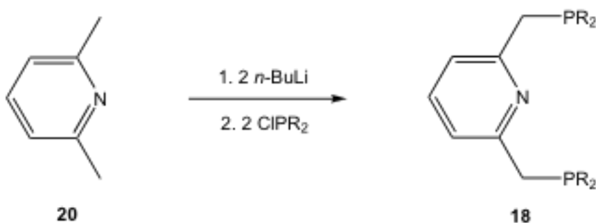
Scheme 12. Preparation of PNP-based Ligands
