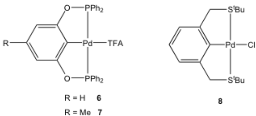
Figure 6. Suzuki-Miyaura Catalysts
