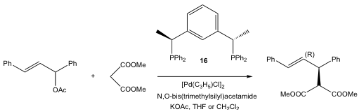
Scheme 9. Asymmetric Allylic Alkylation Catalyst 74
