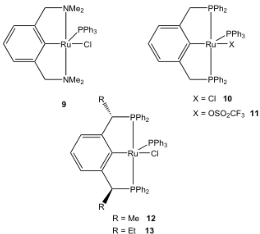
Figure 7. Hydrogen Transfer Catalysts
