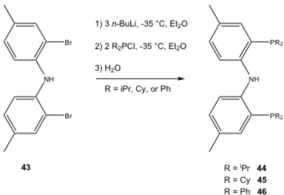
Scheme 22. Preparation of i Pr PNP 44 , Cy PNP 45 , and Ph PNP 46
