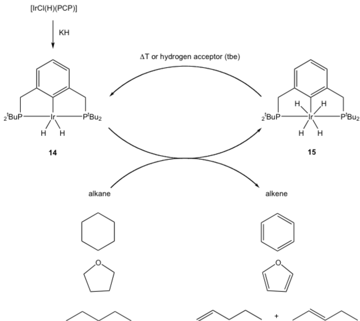
Scheme 8. Alkane Dehydrogenation Catalyst 66
