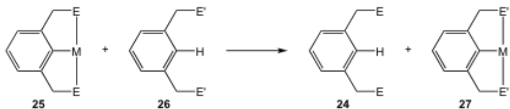
Scheme 14. Various Metalation Techniques 66
