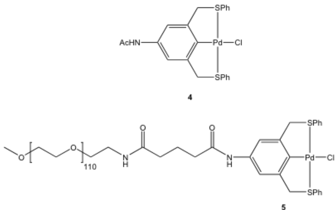
Figure 4. Pd-SCS Heck Catalysts
