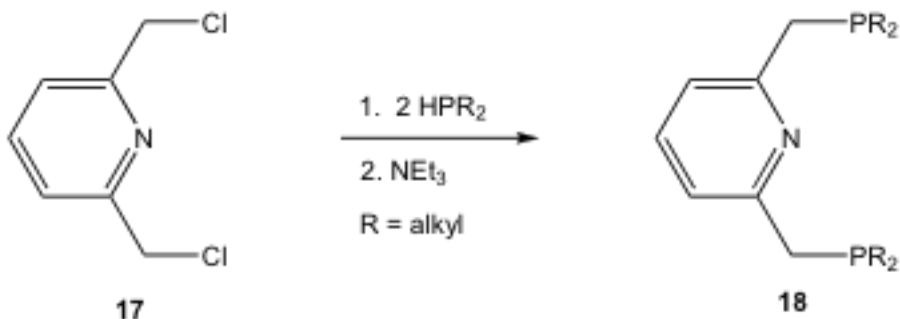
Scheme 10. Preparation of PNP-based Ligands
