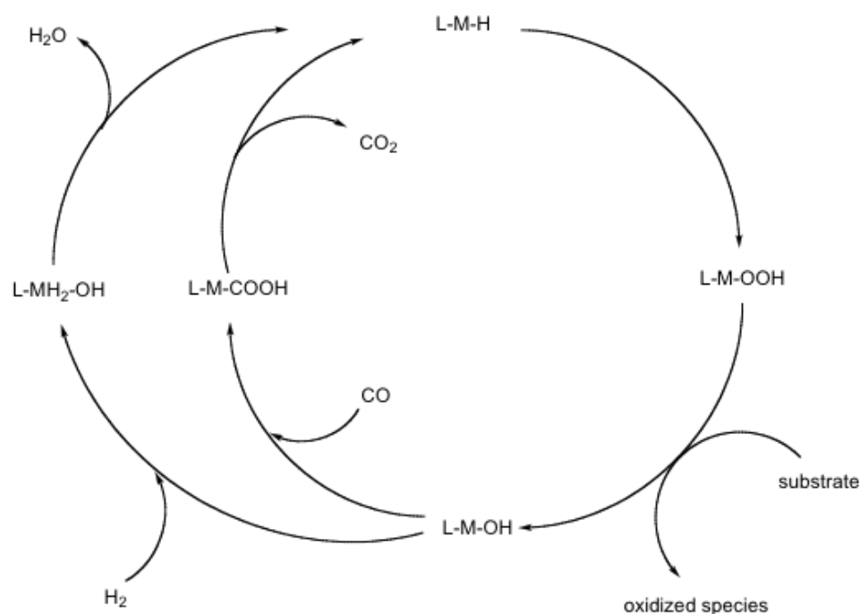
Scheme 4. Proposed Catalytic Cycle for the Partial Oxidation of Organic Substrates
