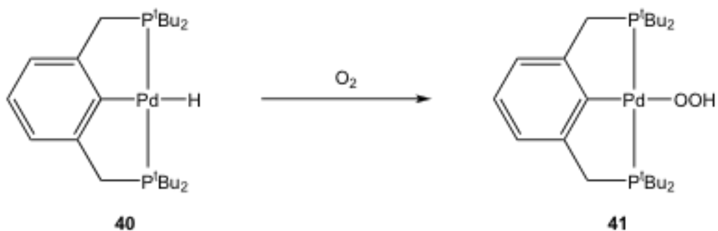
Scheme 20. Synthesis of t BuPCP-Pd-OOH 41
