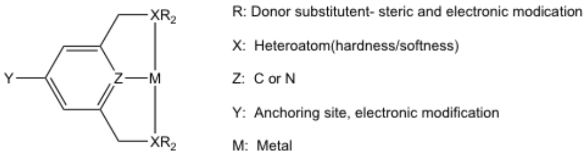
Figure 2: Modification Options of Pincer Ligands
