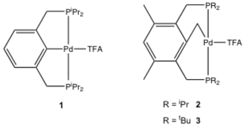
Figure 3. Heck Coupling Catalysts
