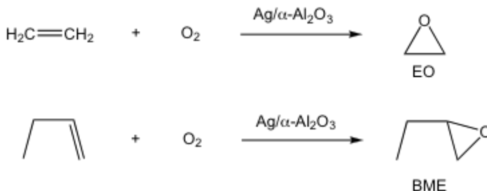
Scheme 1. Direct Epoxidations Using Heterogeneous Catalysts
