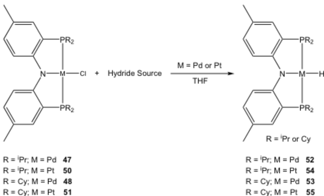
Scheme 24. Preparation of i PrPNP-M-H and CyPNP-M-H
