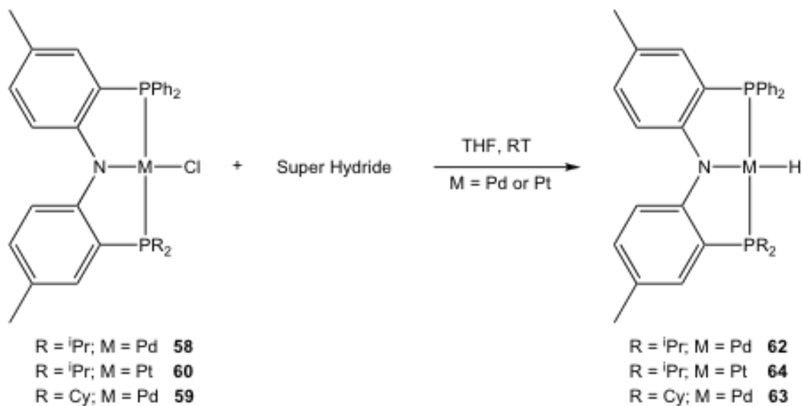
Scheme 27. Preparation of ^{\text{Ph}}\text{PNP}^{\text{iPr}}\text{-M-H} and ^{\text{Ph}}\text{PNP}^{\text{Cy}}\text{-M-H}
