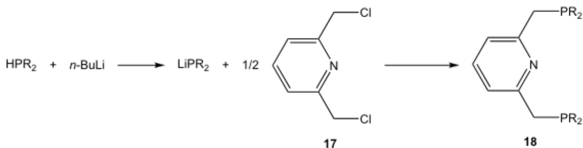
Scheme 11. Preparation of PNP-based Ligands
