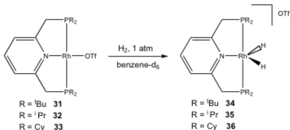
Scheme 18. Preparation of [RPNP-Rh(H) 2 ][OTf]
