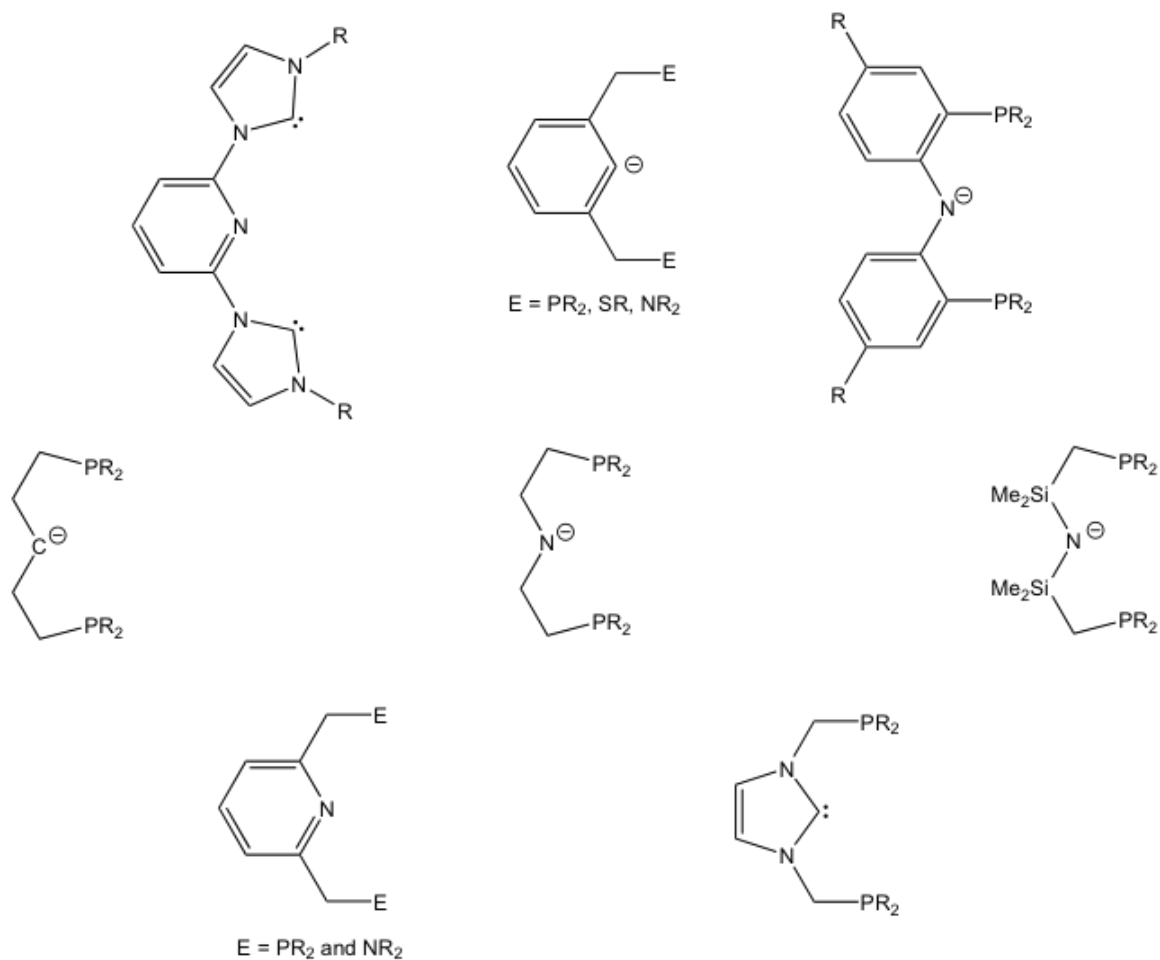
Figure 1. Examples of Pincer Ligands
