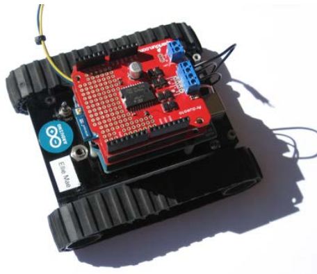
Figure 10 - Motor Driver Shield (stack 2)
