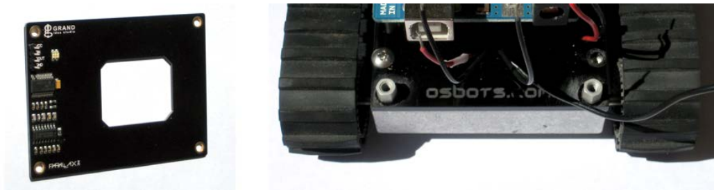
Figure 8 - RFID Module and rear of chassis showing mounting standoffs. Header pins, as supplied were right angle and changed to straight.
