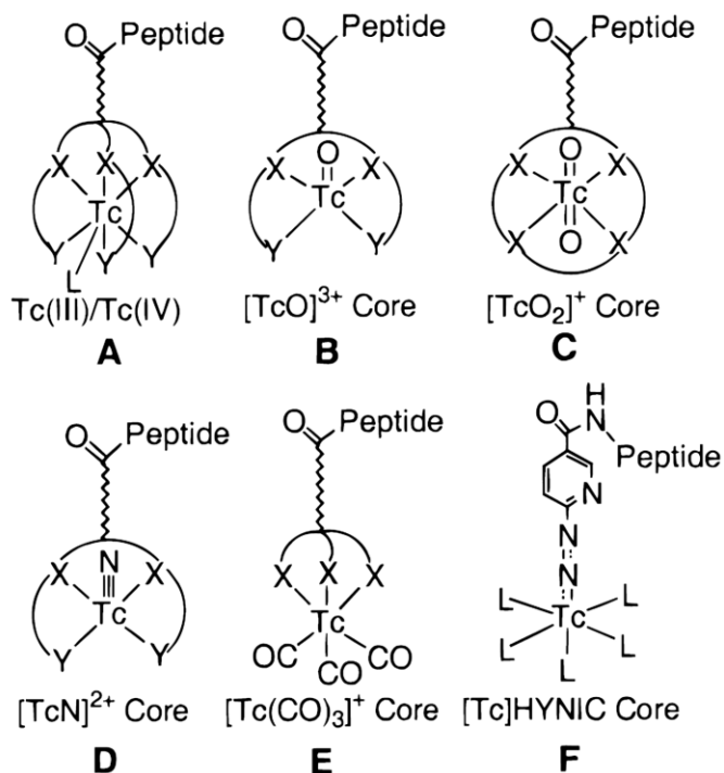
Fig. 1.3- Technetium cores used in ^{99m}\text{Tc} labeling of biomolecules. X= N or S, Y= N or S, L= neutral donor ligand. (Cited from Liu, 1999).
