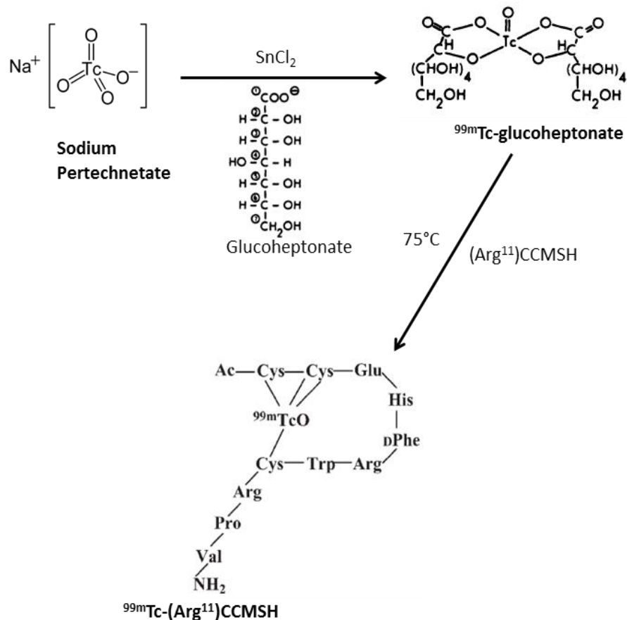
Fig. 1.10- Schematic representation of ligand-exchange radiolabeling with glucoheptonate of ^{99m}\text{Tc} -(Arg 11 )CCMSH. (Adapted from Miao, 2007 and de Kieviet, 1981).
