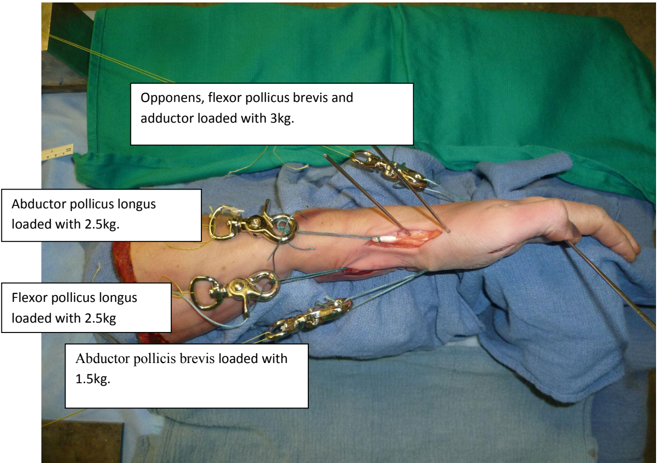
Figure 1: This image represents the specimen, loaded within the jig, with all tendons loaded. Note the k-wire markers placed in the first metacarpal and the scaphoid
