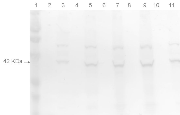
Figure 6. Western blots to detect DB3 protein from Artemia gut extracts. Lane 1, Trichrom ranger TM Molecular marker. Lane 2, 4, 6, 8, and 10, Artemia fed wild type S. bacillarus and harvested 2, 4, 8, 10 and 20 h after the commencement of feeding. Lane 3, 5, 7, 9 and 11, Artemia fed transgenic S. bacillarus and harvested 2, 4, 8, 10 and 20 h after the commencement of feeding.
