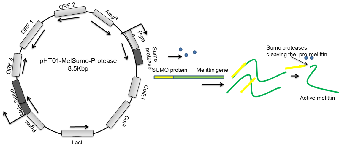
Figure 30. Possible strategy to express melittin in B.subtilis for paratransgenesis. B.subtilis can be transformed with plasmid to express melittin as a fusion protein with SUMO protein (melittin+SUMO protein). The plasmid also expresses and extracellularly secretes SUMO protease, which specifically cleaves SUMO protein from the fusion protein to release the active melittin.
