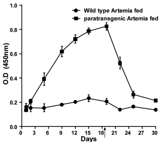
Figure 9. Progesterone-binding activity of gut extracts of shrimp. Shrimp were fed paratransgenic Artemia engorged with DB3-producing E. coli or fed Artemia engorged with nontransgenic E. coli per the trial 1 protocol. The arrow (d 19) indicates the start of wash-out period where the feeding of wild type or paratransgenic Artemia was stopped. Values are represented mean \pm SEM (n-3).
