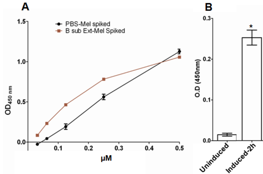
Figure 26. ELISA to detect melittin production from transgenic B. subtilis 168-pHT01-Mel. A) Standard curve of melittin spiked (0.03-0.50 \mu M) in PBS or B.subtilis 168 extract B) Melittin specific signal from 2 h induced samples compared to uninduced control samples. The asterisk represents significant difference in the means ( P < 0.05 ).
