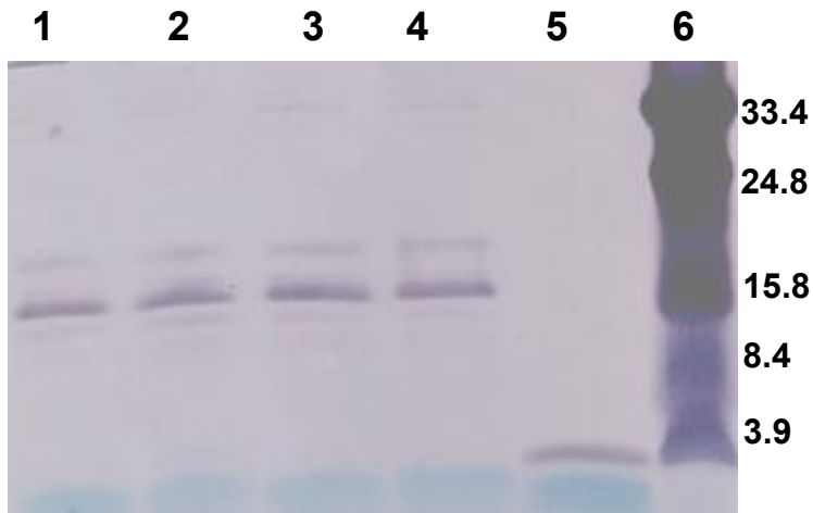
Figure 25. Western blot to detect melittin (Study 4). No melittin specific band was observed from the induced samples. pHT-Mel 3 h Ind (lane 1); pHT-Mel 2h Ind (lane 2); pHT-Mel 1.0 h Ind (lane 3); pHT-Mel Uninduced (lane 4); Syn Mel- positive Control (lane 5); Polypeptide marker (lane 6).
