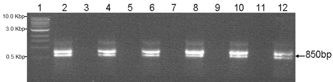
Figure 5. PCR amplification for the detection of DB3 gene from Artemia gut extracts. Lane 1, 1 Kb DNA ladder. Lane 2, positive control (pRrMDWK6). Lane 3, 5, 7, 9 and 11 represents PCR products from Artemia gut extracts fed with wild type S. bacillus after 2, 4, 8, 10 and 20 h after feeding. Lane 4, 6, 8, 10 and 12 represents PCR products from Artemia gut extracts fed with transgenic S. bacillus after 2, 4, 8, 10 and 20 h after feeding.
