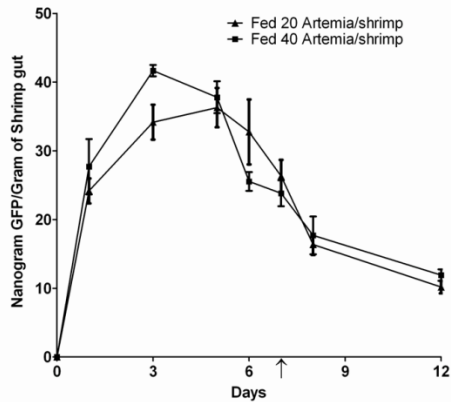
Figure 12. Quantity of GFP in the shrimp gut fed daily with paratransgenic Artemia (at a rate of 20 or 40 Artemia per day) engorged with GFP expressing E. coli . The data are averages \pm SEM from two treatments. The arrow (d 7) indicates the start of wash-out period.
