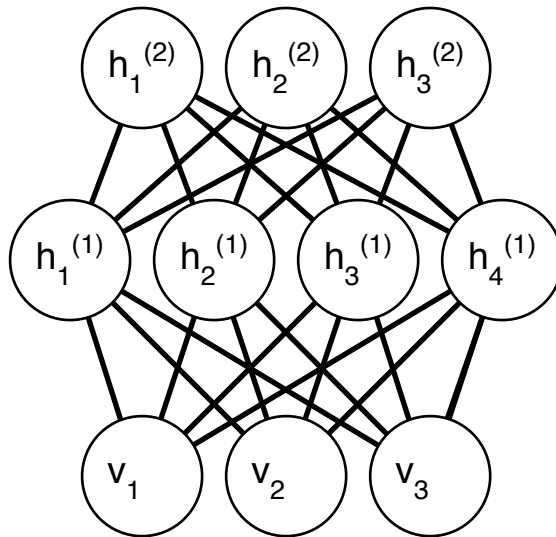
Figure 2.2 – An example graph of a deep Boltzmann machine
