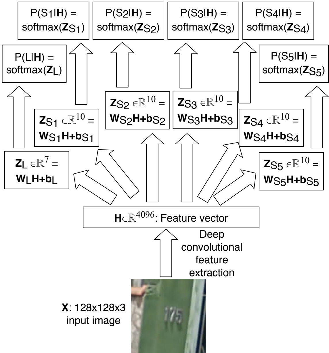
Figure A.1 – Details of the computational graph we used to transcribe house numbers. In this diagram, we show how we compute the parameters of P(\mathbf{S} | \mathbf{X}) , where X is the input image and \mathbf{S} is the sequence of numbers depicted by the image. We first extract a set of features \mathbf{H} from \mathbf{X} using a convolutional network with a fully connected final layer. Note that only one such feature vector is extracted for the entire image. We do not use an HMM that models features explicitly extracted at separate locations. Because the final layer of the convolutional feature extractor is fully connected and has no weight sharing, we have not explicitly engineered any concept of spatial location into this representation. The network must learn its own means of representing spatial location in \mathbf{H} . Six separate softmax classifiers are then connected to this feature vector \mathbf{H} , i.e., each softmax classifier forms a response by making an affine transformation of \mathbf{H} and normalizing this response with the softmax function. One of these classifiers provides the distribution over the sequence length P(L | \mathbf{H}) , while the others provide the distribution over each of the members of the sequence, P(S_1 | \mathbf{H}), \dots, P(S_5 | \mathbf{H}) .
