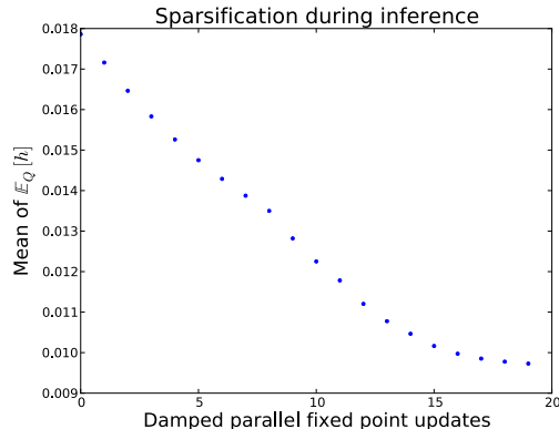
Figure 5.3 – The explaining-away effect makes the S3C representation become more sparse with each damped iteration of the variational inference fixed point equations.
