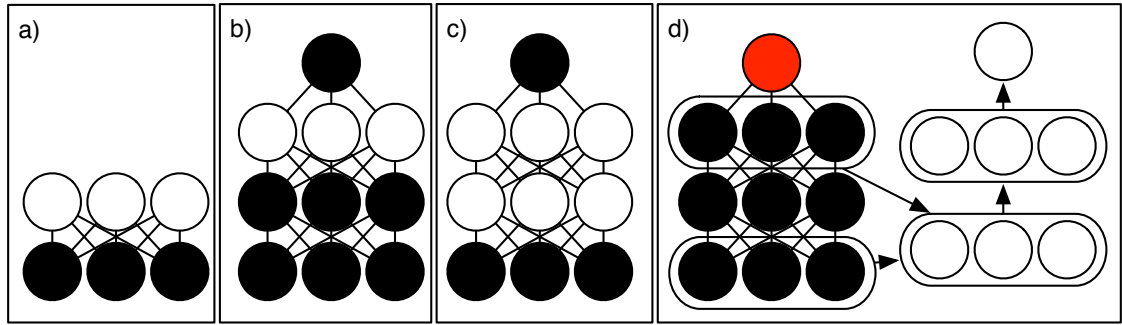
Figure 7.1 – The training procedure used by Salakhutdinov and Hinton (2009) on MNIST. a) Train an RBM to maximize \log P(v) using CD. b) Train another RBM to maximize \log P(h^{(1)}, y) where h^{(1)} is drawn from the first RBM’s posterior. c) Stitch the two RBMs into one DBM. Train the DBM to maximize \log P(v, y) . d) Delete y from the model (don’t marginalize it out, just remove the layer from the model). Make an MLP with inputs v and the mean field expectations of h^{(1)} and h^{(2)} . Fix the DBM parameters. Initialize the MLP parameters based on the DBM parameters. Train the MLP parameters to predict y .
