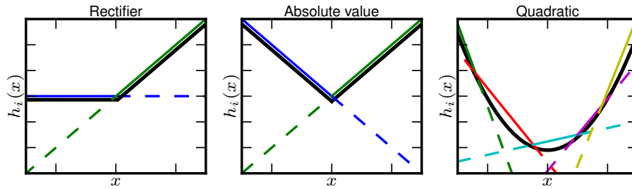
Figure 9.1 – Graphical depiction of how the maxout activation function can implement the rectified linear, absolute value rectifier, and approximate the quadratic activation function. This diagram is 2D and only shows how maxout behaves with a 1D input, but in multiple dimensions a maxout unit can approximate arbitrary convex functions.
