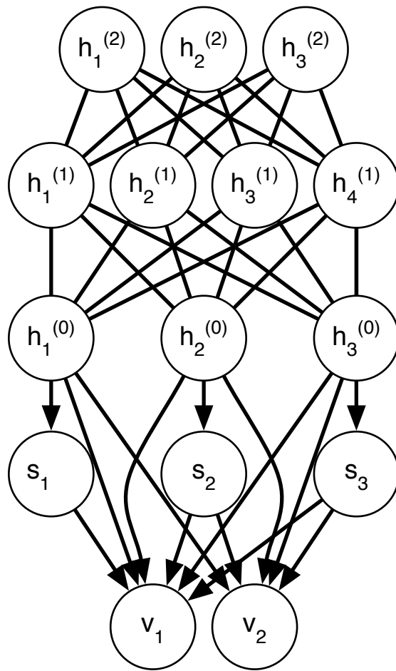
Figure 5.1 – A graphical model depicting an example PD-DBM.
