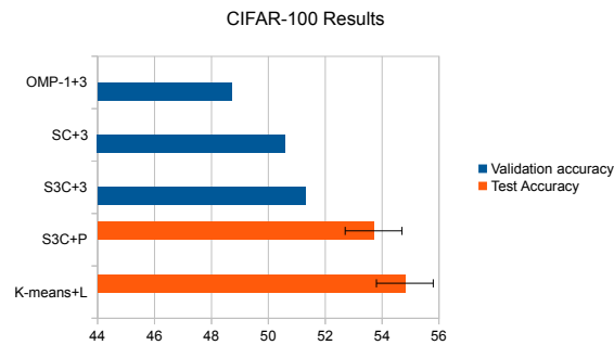
Figure 5.9 – CIFAR-100 classification accuracy for various models. As expected, S3C outperforms SC (sparse coding) and OMP-1. S3C with spatial pyramid pooling is near the state-of-the-art method, which uses a learned pooling structure.
