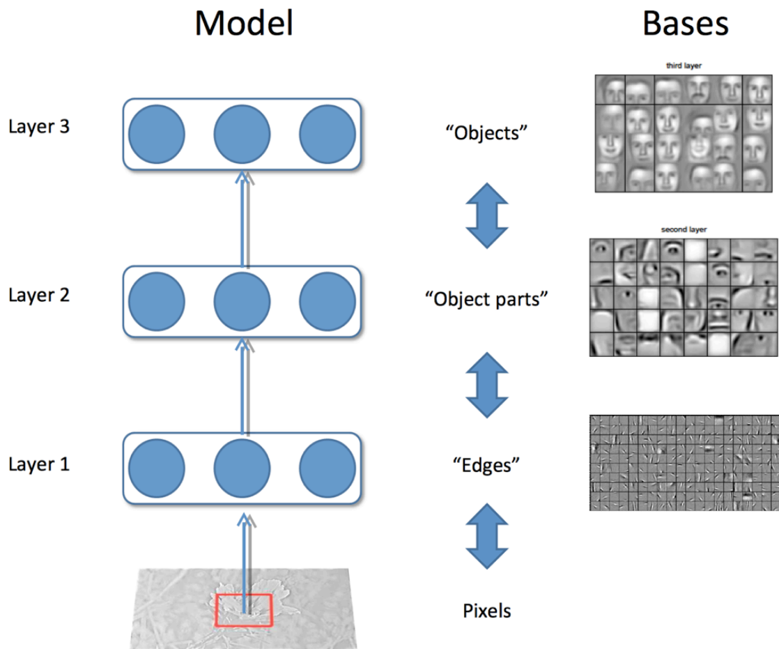
Figure 1.2 – Deep learning example : When trained on images, the first layer of a deep learning system operates on the pixels and usually extracts some sort of edges from the image. The second layer operates on this representation in terms of edges and might extract small object parts that can be described as collections of small numbers of edges. The third layer operates on this representation in terms of object parts and might extract entire objects that can be described as collections of small numbers of object parts. The exact results depend on the algorithm employed, model architecture, and formatting of the dataset. ( This image was joint work with Honglak Lee and Andrew Saxe, originally prepared for an oral presentation of (Goodfellow et al., 2009) )
