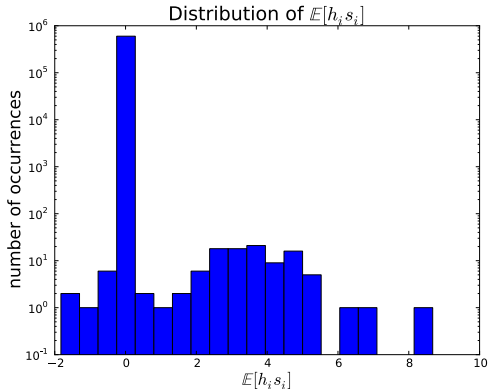
Figure 5.2 – This example histogram of \mathbb{E}_Q[h_i s_i] shows that Q is a sparse distribution. For this 6,000 hidden unit S3C model trained on 6 \times 6 image patches, Q(h_i = 1) < .01 99.7% of the time.
