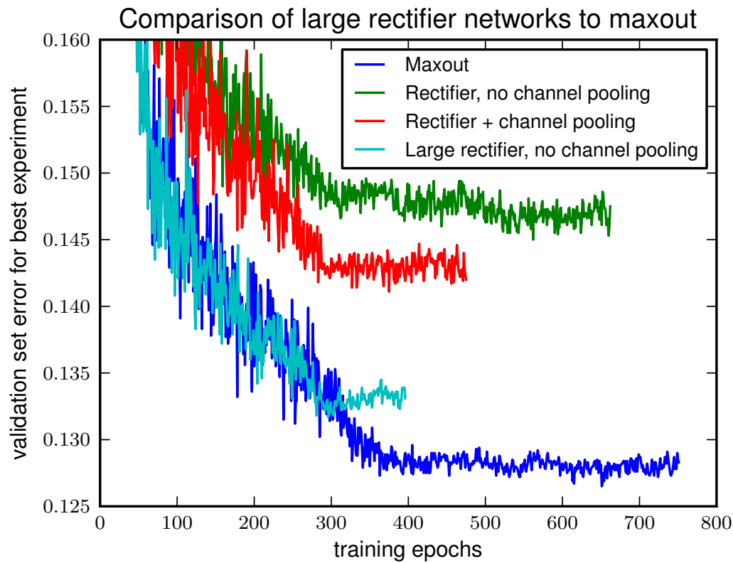
Figure 9.6 – We cross-validated the momentum and learning rate for four architectures of model: 1) Medium-sized maxout network. 2) Rectifier network with cross-channel pooling, and exactly the same number of parameters and units as the maxout network. 3) Rectifier network without cross-channel pooling, and the same number of units as the maxout network (thus fewer parameters). 4) Rectifier network without cross-channel pooling, but with k times as many units as the maxout network. Because making layer i have k times more outputs increases the number of inputs to layer i + 1 , this network has roughly k times more parameters than the maxout network, and requires significantly more memory and runtime. We sampled 10 learning rate and momentum schedules and random seeds for dropout, then ran each configuration for all 4 architectures. Each curve terminates after failing to improve the validation error in the last 100 epochs.
