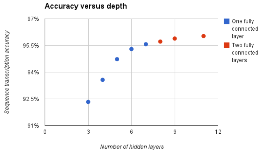
Figure 11.4 – Performance analysis experiments on the public SVHN dataset show that fairly deep architectures are needed to obtain good performance on the sequence transcription task.
