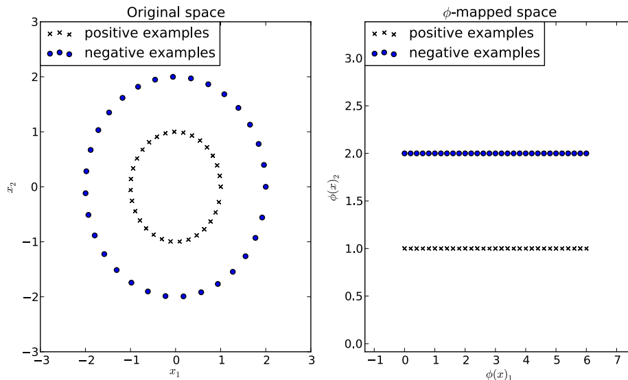
Figure 1.1 – Left: An example dataset for an SVM. Right: The same dataset transformed by \phi(x) , where \phi is conversion to polar coordinates.
