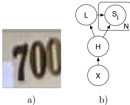
Figure 11.1 – a) An example input image to be transcribed. The correct output for this image is “700”. b) The graphical model structure of our sequence transcription model, depicted using plate notation (Buntine, 1994) to represent the multiple S_i . Note that the relationship between X and H is deterministic. The edges going from L to S_i are optional, but help draw attention to the fact that our definition of P(\mathbf{S} | X) does not query S_i for i > L .
