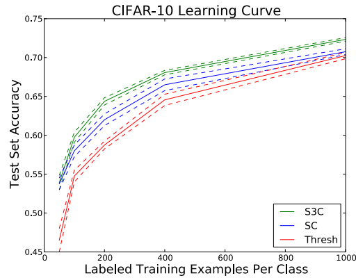
Figure 5.8 – Semi-supervised classification accuracy on subsets of CIFAR-10. Thresholding, the best feature extractor on the full dataset, performs worse than sparse coding when few labels are available. S3C improves upon sparse coding’s advantage.
