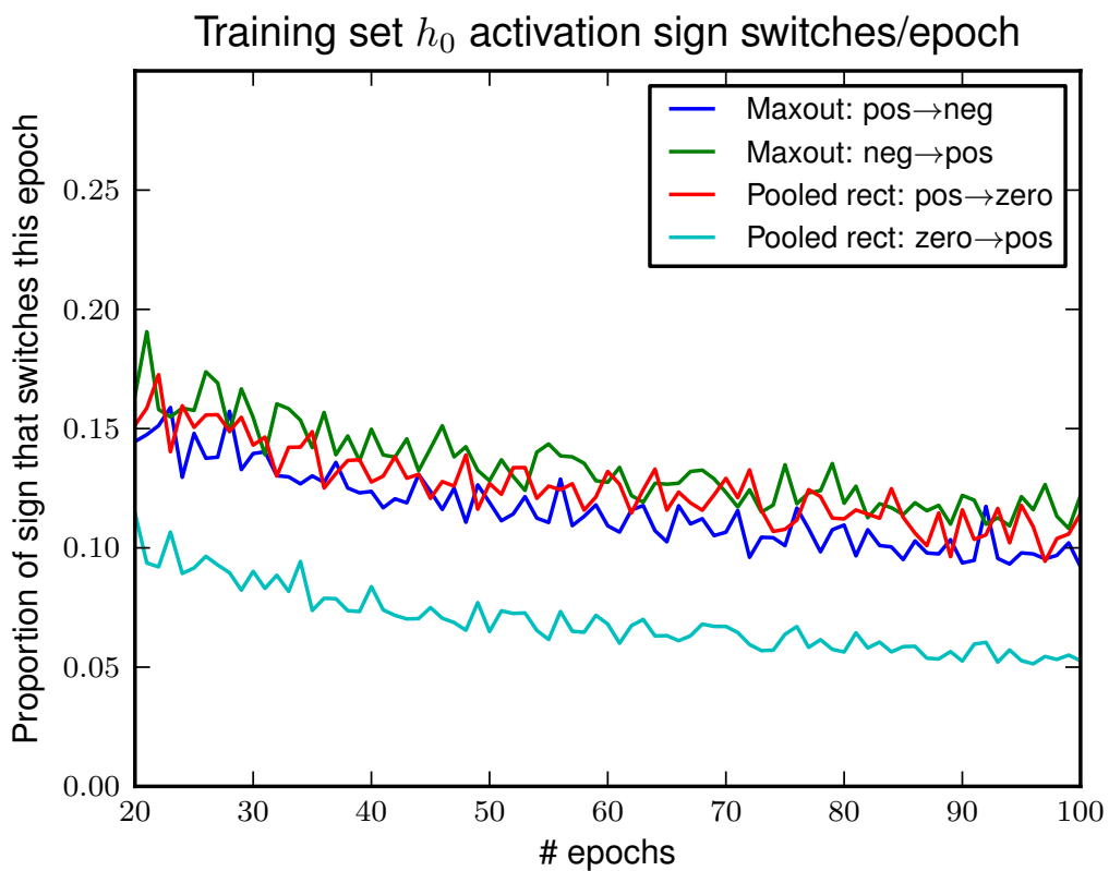
Figure 9.10 – During dropout training, rectifier units transition from positive to 0 activation more frequently than they make the opposite transition, resulting a preponderance of 0 activations. Maxout units freely move between positive and negative signs at roughly equal rates.
