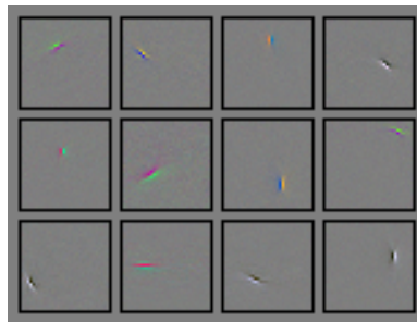
Figure 5.6 – Example filters from a dictionary of over 8,000 learned on full 32x32 images.
