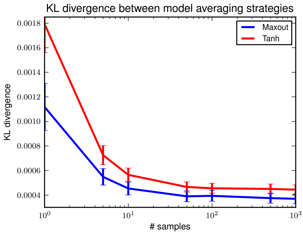
Figure 9.8 – The KL divergence between the distribution predicted using the dropout technique of dividing the weights by 2 and the distribution obtained by taking the geometric mean of the predictions of several sampled models decreases as the number of samples increases. This suggests that dropout does indeed do model averaging, even for deep networks. The approximation is more accurate for maxout units than for tanh units.
