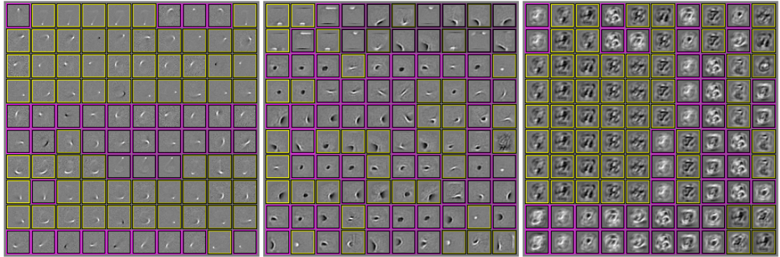
Figure 5.13 – Each panel shows a visualization of the weights for a different model. Each row represents a different second layer hidden unit. We show ten units for each model corresponding to those with the largest weight vector norm. Within each row, we plot the weight vectors for the ten most strongly connected first layer units. Black corresponds to inhibition, white to excitation, and gray to zero weight. This figure is best viewed in color—units plotted with a yellow border have excitatory second layer weights while units plotted with a magenta border have inhibitory second layer weights. Left: PD-DBM model trained jointly. Note that each row contains many similar filters. This is how the second layer weights achieve invariance to some transformations such as image translation. This is one way that deep architectures are able to disentangle factors of variation. One can also see how the second layer helps implement the correct prior for the generative task. For example, the unit plotted in the first row excites filters used to draw 7s and inhibits filters used to draw 1s. Also, observe that the first layer filters are much more localized and contained fewer templates than those in Fig. 5.11 right. This suggests that joint training has a significant effect on the quality of the first layer weights; greedy pretraining would have attempted to solve the generative task with more templates due to S3C’s independent prior. Center: DBM model with greedy pretraining followed by joint training. These weights show the same disentangling and invariance properties as those of the PD-DBM. Note that the filters have more black areas. This is because the RBM must use inhibitory weights to limit hidden unit activities, while S3C accomplishes the same purpose via the explaining-away effect. Right: DBM with joint training only. Note that many of the second layer weight vectors are duplicates of each other. This is because the second layer has a pathological tendency to focus on modeling a handful of first-layer units that learn interesting responses earliest in learning.
