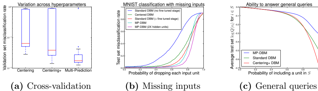
Figure 7.6 – Quantitative results on MNIST: (a) During cross-validation, MP training performs well for most hyperparameters, while both centering and centering with the special negative phase do not perform as well and only perform well for a few hyperparameter values. Note that the vertical axis is on a log scale. (b) Generic inference tasks: When classifying with missing inputs, the MP-DBM outperforms the other DBMs for most amounts of missing inputs. (c) When using approximate inference to resolve general queries, the standard DBM, centered DBM, and MP-DBM all perform about the same when asked to predict a small number of variables. For larger queries, the MP-DBM performs the best.
