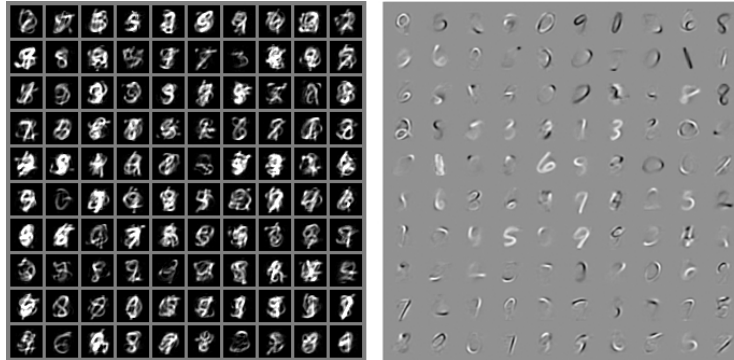
Figure 5.11 – Left : Samples drawn from an S3C model trained on MNIST. Right : The filters used by this S3C model.
