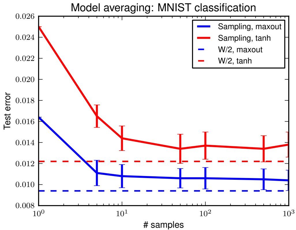
Figure 9.7 – The error rate of the prediction obtained by sampling several sub-models and taking the geometric mean of their predictions approaches the error rate of the prediction made by dividing the weights by 2. However, the divided weights still obtain the best test error, suggesting that dropout is a good approximation to averaging over a very large number of models. Note that the correspondence is more clear in the case of maxout.
