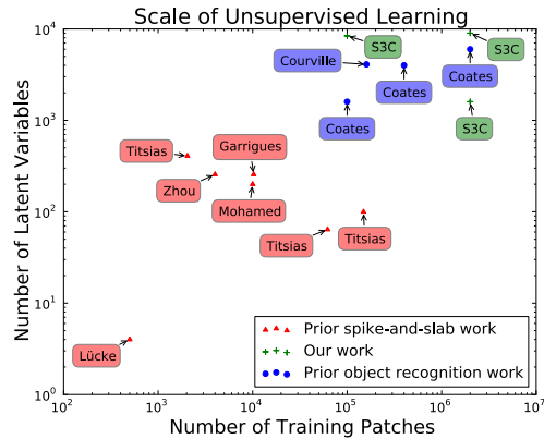
Figure 5.5 – Our inference scheme enables us to extend spike-and-slab modeling from small problems to the scale needed for object recognition. Previous object recognition work is from (Coates and Ng, 2011; Courville et al., 2011b). Previous spike-and-slab work is from (Mohamed et al., 2012; Zhou et al., 2009; Garrigues and Olshausen, 2008; Lücke and Sheikh, 2011; Titsias and Lázaro-Gredilla, 2011).
