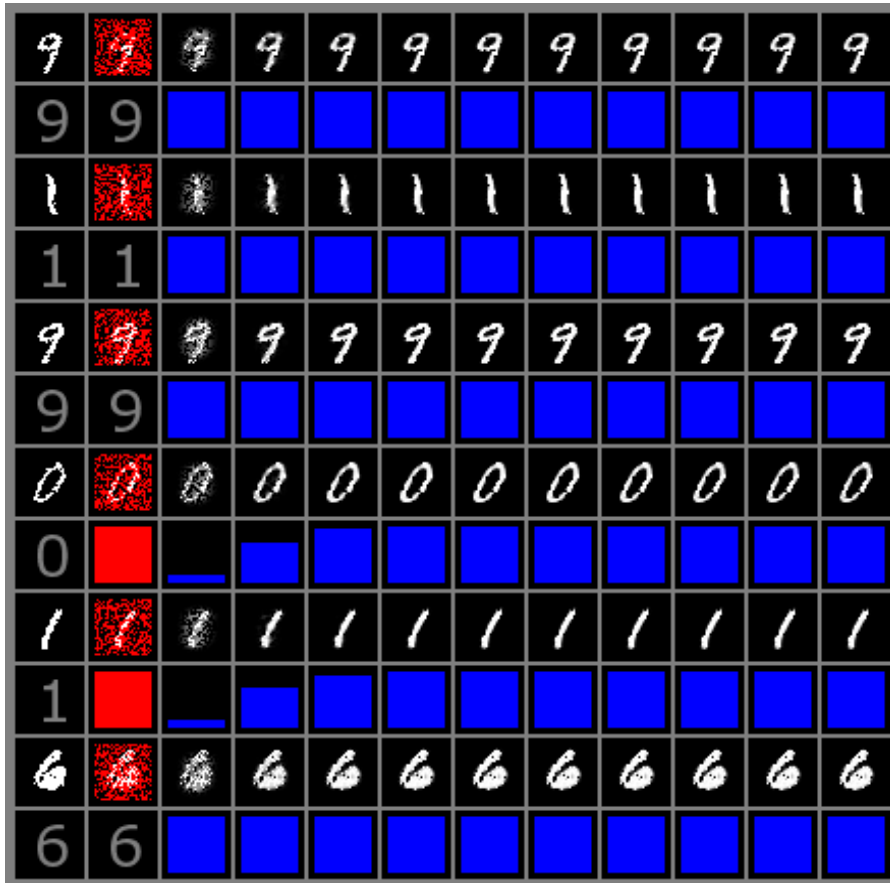
Figure 7.3 – Mean field inference applied to MNIST digits. Within each pair of rows, the upper row shows pixels and the lower row shows class labels. The first column shows a complete, labeled example. The second column shows information to be masked out, using red pixels to indicate information that is removed. The subsequent columns show steps of mean field. The images show the pixels being filled back in by the mean field inference, and the blue bars show the probability of the correct class under the mean field posterior.
