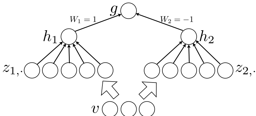
Figure 9.3 – An MLP containing two maxout units can arbitrarily approximate any continuous function. The weights in the final layer can set g to be the difference of h_1 and h_2 . If z_1 and z_2 are allowed to have arbitrarily high cardinality, h_1 and h_2 can approximate any convex function. g can thus approximate any continuous function due to being a difference of approximations of arbitrary convex functions.
