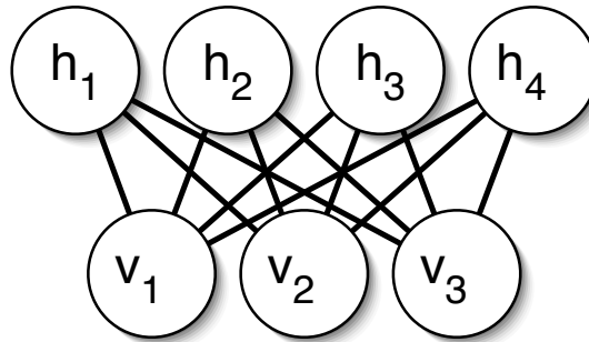
Figure 2.1 – An example RBM drawn as a Markov network
