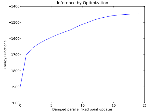
Figure 5.4 – The negative variational free energy of a batch of 5000 image patches increases during the course of variational inference.
