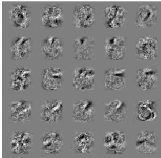
Figure 9.4 – Example filters learned by a maxout MLP trained with dropout on MNIST. Each row contains the filters whose responses are pooled to form a maxout unit.
