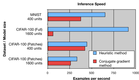
Figure 5.7 – The inference speed for each method was computed based on the inference time for the same set of 100 examples from each dataset. The heuristic method is consistently faster than the conjugate gradient method. The conjugate gradient method is slowed more by problem size than the heuristic method is, as shown by the conjugate gradient method’s low speed on the CIFAR-100 full image task. The heuristic method has a very low cost per iteration but is strongly affected by the strength of explaining-away interactions—moving from CIFAR-100 full images to CIFAR-100 patches actually slows it down because the degree of overcompleteness increases.
