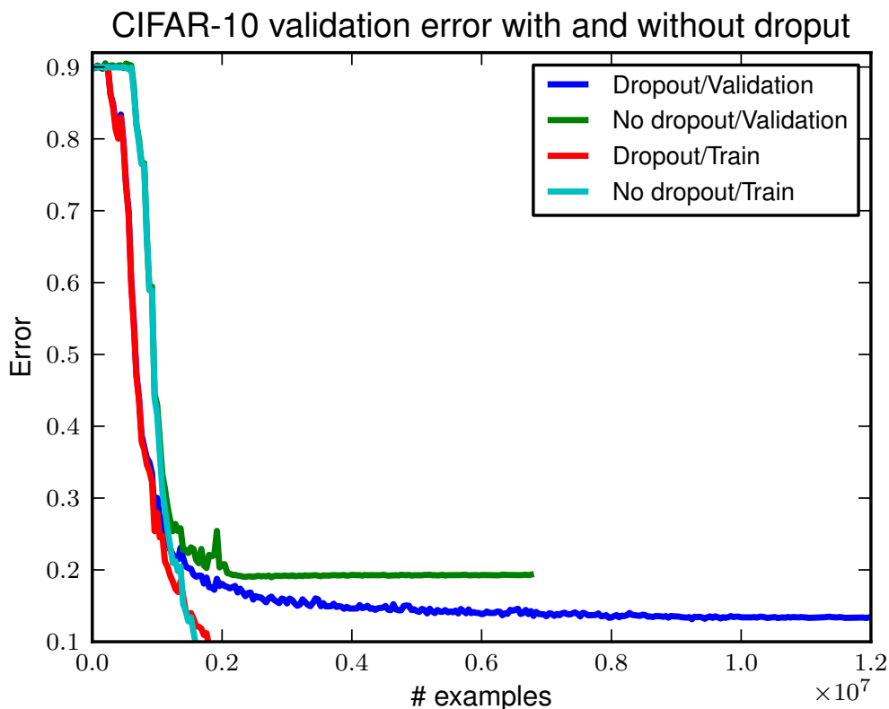
Figure 9.5 – When training maxout, the improvement in validation set error that results from using dropout is dramatic. Here we find a greater than 25% reduction in our validation set error on CIFAR-10.
