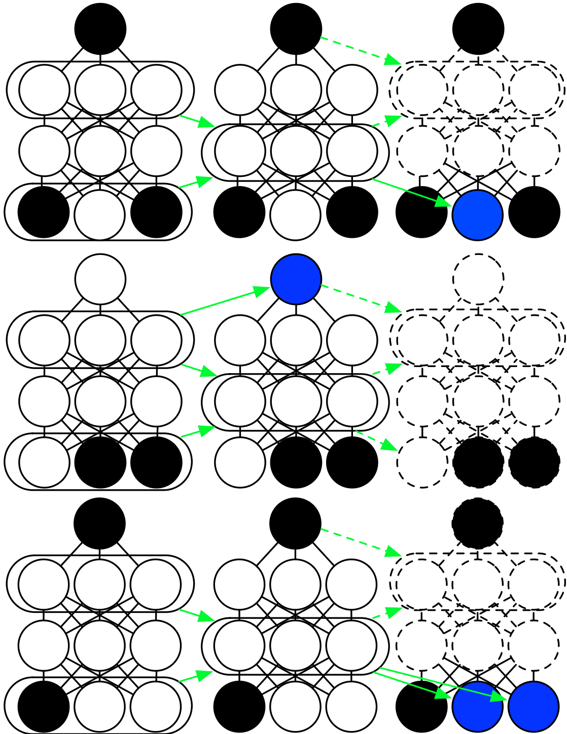
Figure 7.2 – Multi-prediction training : This diagram shows the neural nets instantiated to do multi-prediction training on one minibatch of data. The three rows show three different examples. Black circles represent variables the net is allowed to observe. Blue circles represent prediction targets. Green arrows represent computational dependencies. Each column shows a single mean field fixed point update. Each mean field iteration consists of two fixed point updates. Here we show only one iteration to save space, but in a real application MP training should be run with 5-15 iterations.
