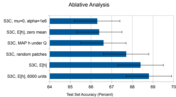
Figure 5.10 – Performance of several limited variants of S3C
