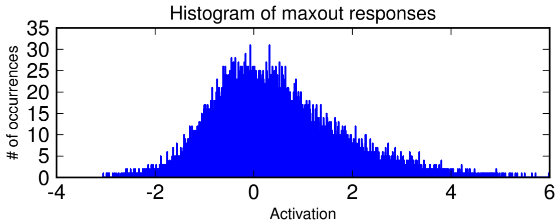
Figure 9.2 – The activations of maxout units are not sparse.
