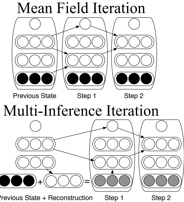
Figure 7.4 – Multi-inference trick : When estimating y given v , a mean field iteration consists of first applying a mean field update to h^{(1)} and y , then applying one to h^{(2)} . To use the multi-inference trick, start the iteration by computing r as the mean field update v would receive if it were not observed. Then use 0.5(r + v) in place of v and run a regular mean field iteration.
