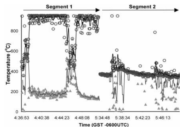
Figure 4. Temperature values derived from radiance flux dataset showing two-component thermal surface for segment 1 and homogeneous surface for segment 2. T_h is shown in solid circles and T_c is shown in gray solid triangles. 15s moving average for T_h and T_c are shown in solid black and gray solid lines respectively.
