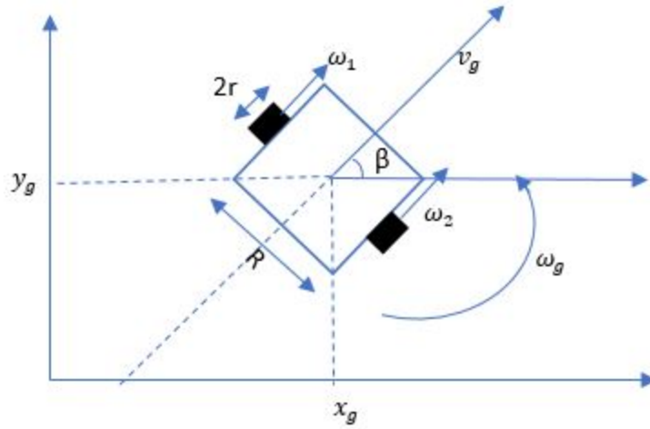
Figure 6.2: Vehicle in an Initial Frame of Reference
