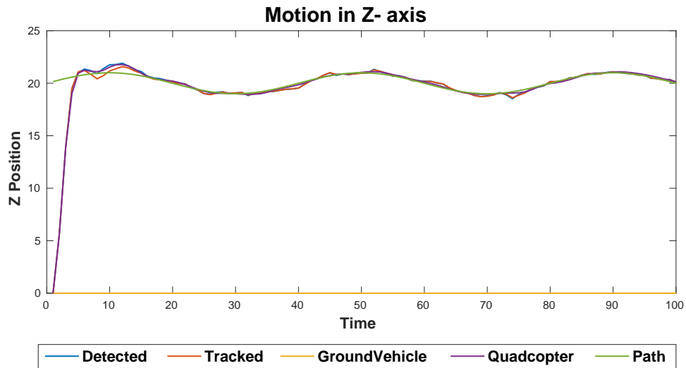
Figure 7.36: Case 5: Results for Closed Loop when z varies
