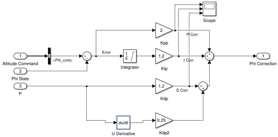
Figure 7.19: Conventional PID with Feed Forward Control
