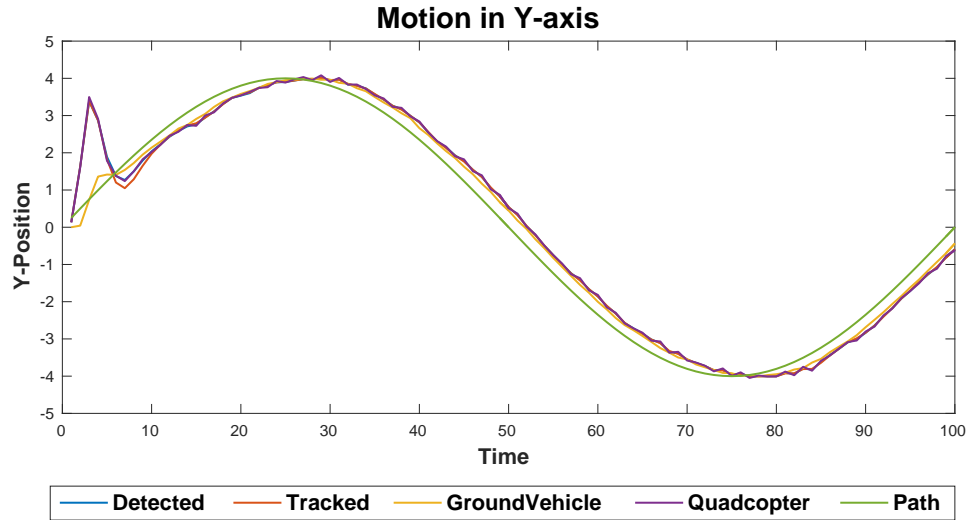
Figure 7.1: Case 1:Results for Closed Loop for Varying y
