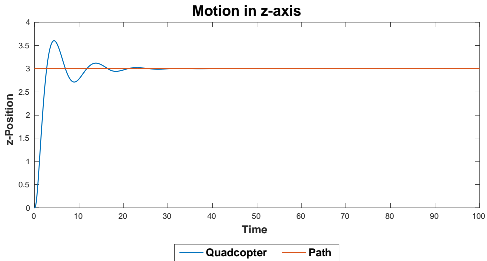
Figure 4.9: Plot of Position Controller Action in z direction
