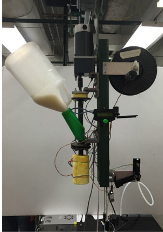
Figure 2.1 Verticle DC recyclebot. The white hopper is on the upper left and the black spooler is on the upper right. The motor in the upper middle drives and auger that feeds plastic into the hot zone (insulated in yellow). Filament is produced and looped through a light sensor to maintain loop length and thus filament diameter automatically. In this setup up the length and diameter can be measured continually.
