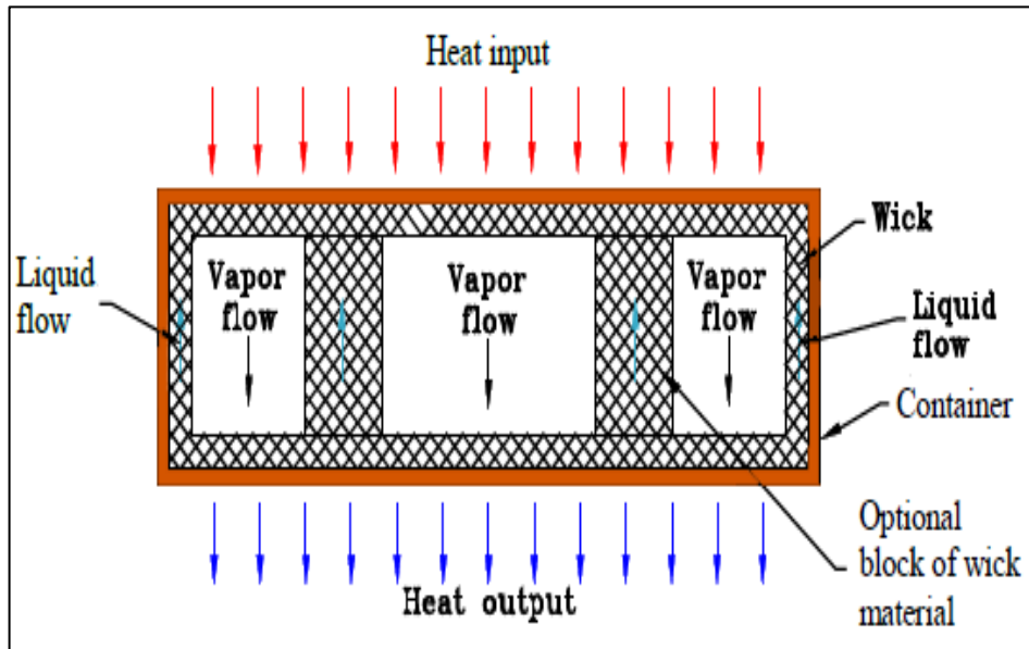
Figure 1.6 Vapor Chamber [1]
