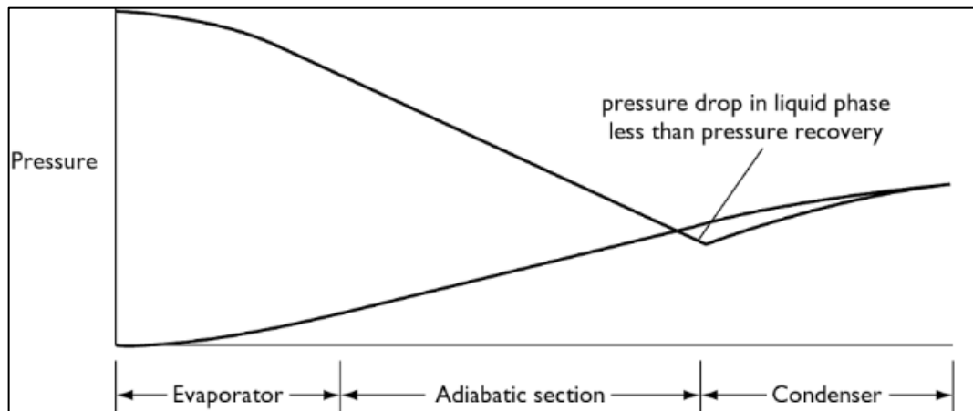
Figure 3.5 Pressure Recovery less than Vapor Phase [2]
