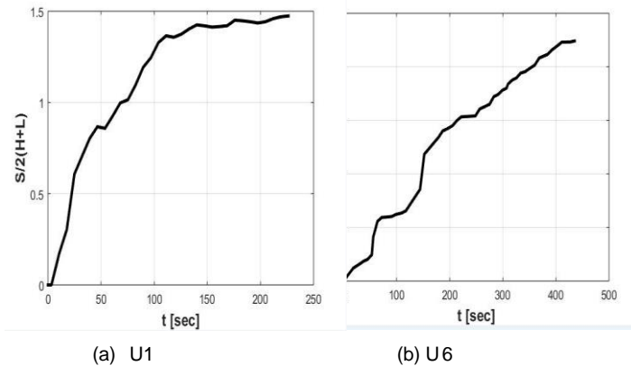
Figure 3.4: S Curve for water displacing oil at flowrate U1 and U6
