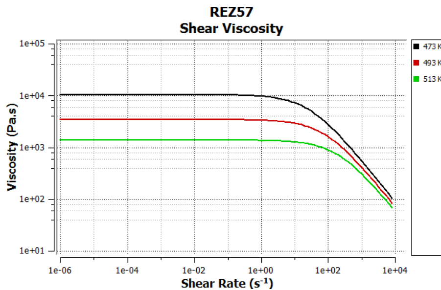
Figure 6 Polymer viscosity graph
