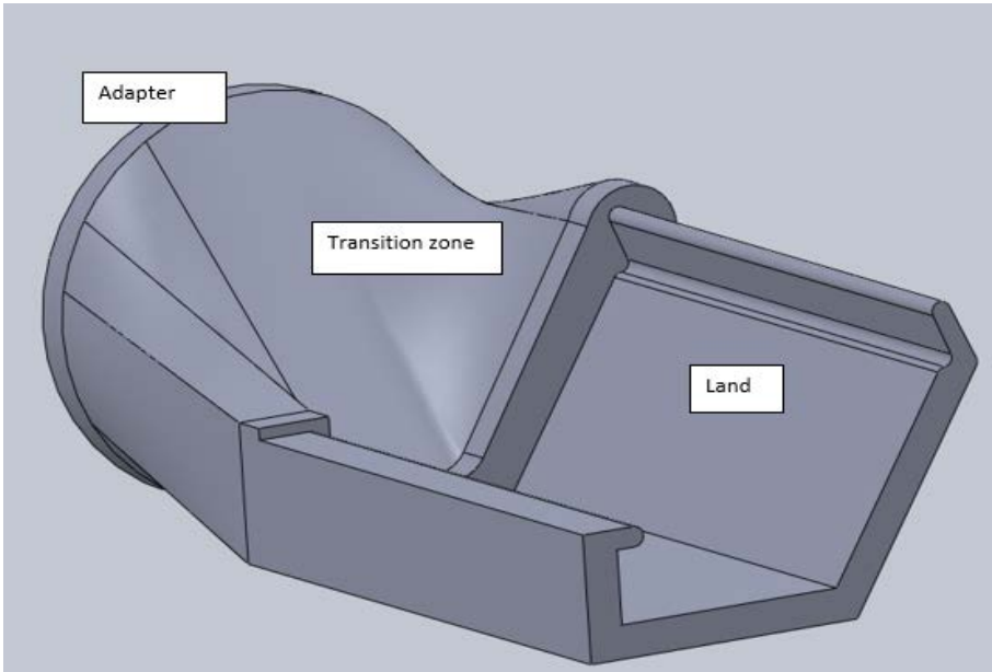
Figure 12 3-D model of initial extrusion die
