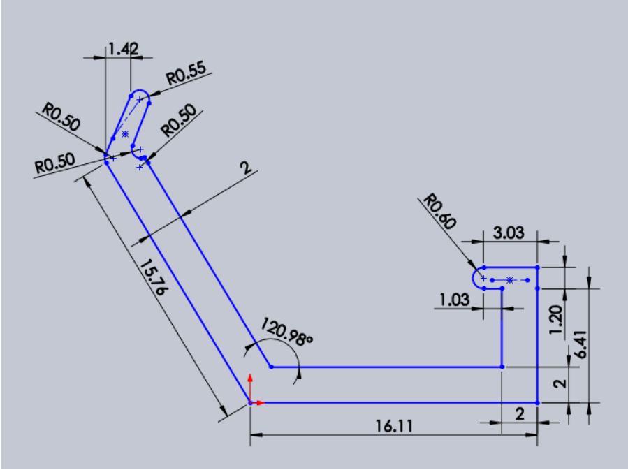
Figure 11 Extrudate dimensions (in mm)
