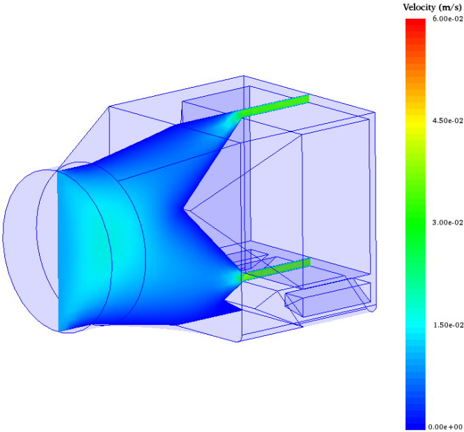
Figure 56 Flow simulation of modified die with no dead spots
