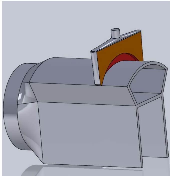
Figure 61 Modified co-extrusion die CAD model
