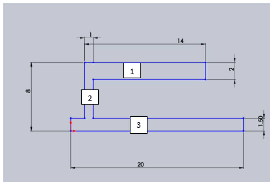
Figure 65 Extrudate dimensions (in mm)
