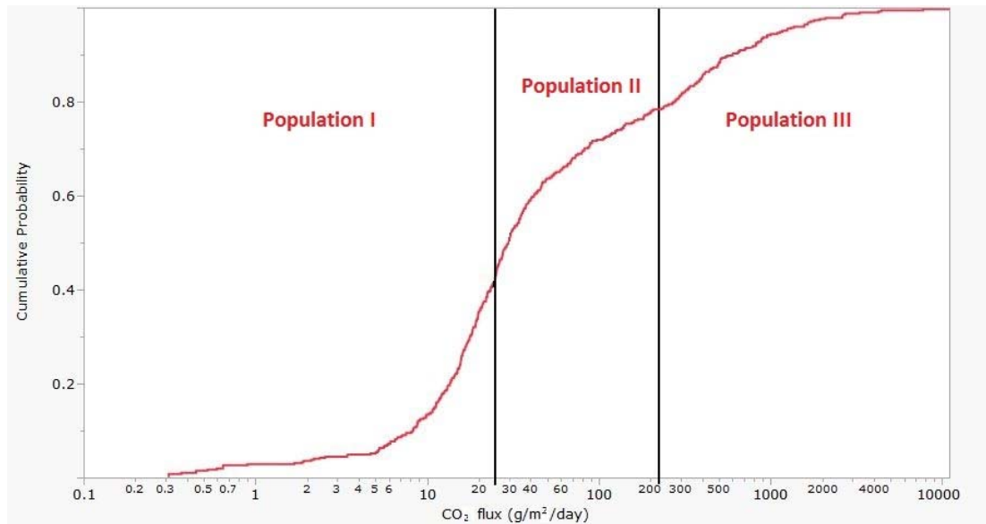
Fig. 9, CDP of the measurements in the LH area with population break points (black lines) at 25 and 225 g/m 2 /day, where population I is the background, population II the mixed group and population III the peak
