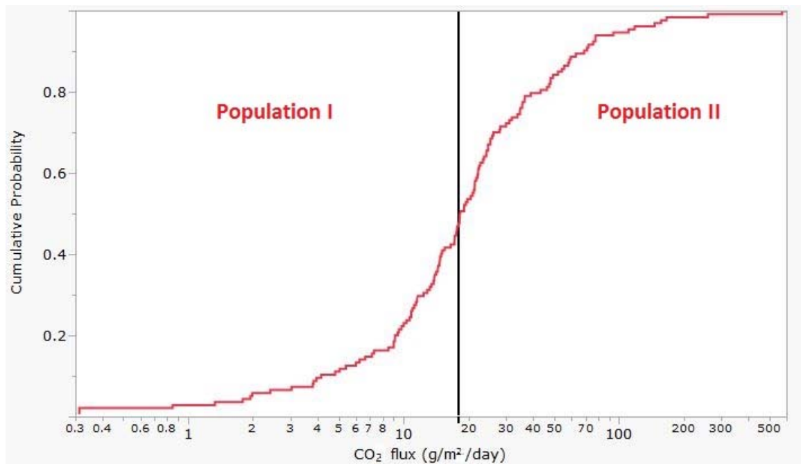
Fig. 16, CDF am of the CO 2 measurements in the LP area with a break point at 18 g/m 2 /day, separating background (population I) and peak (population II) flux
