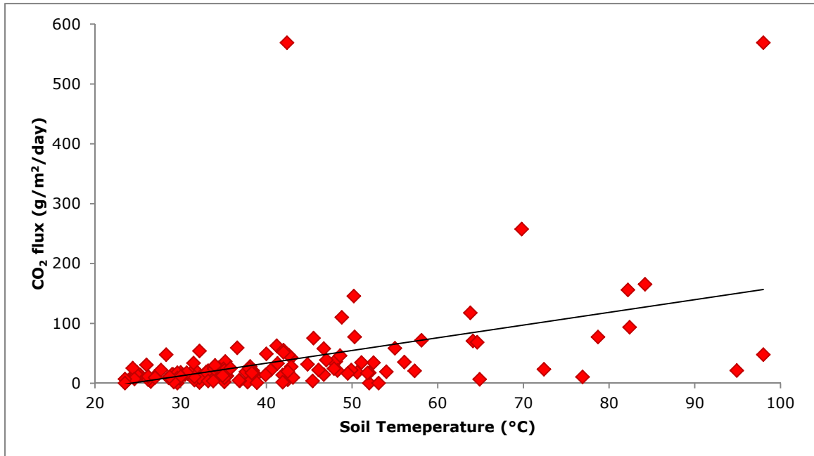
Fig. 19, Positive linear correlation (black line) of CO 2 flux and soil temperature in the LP study area
