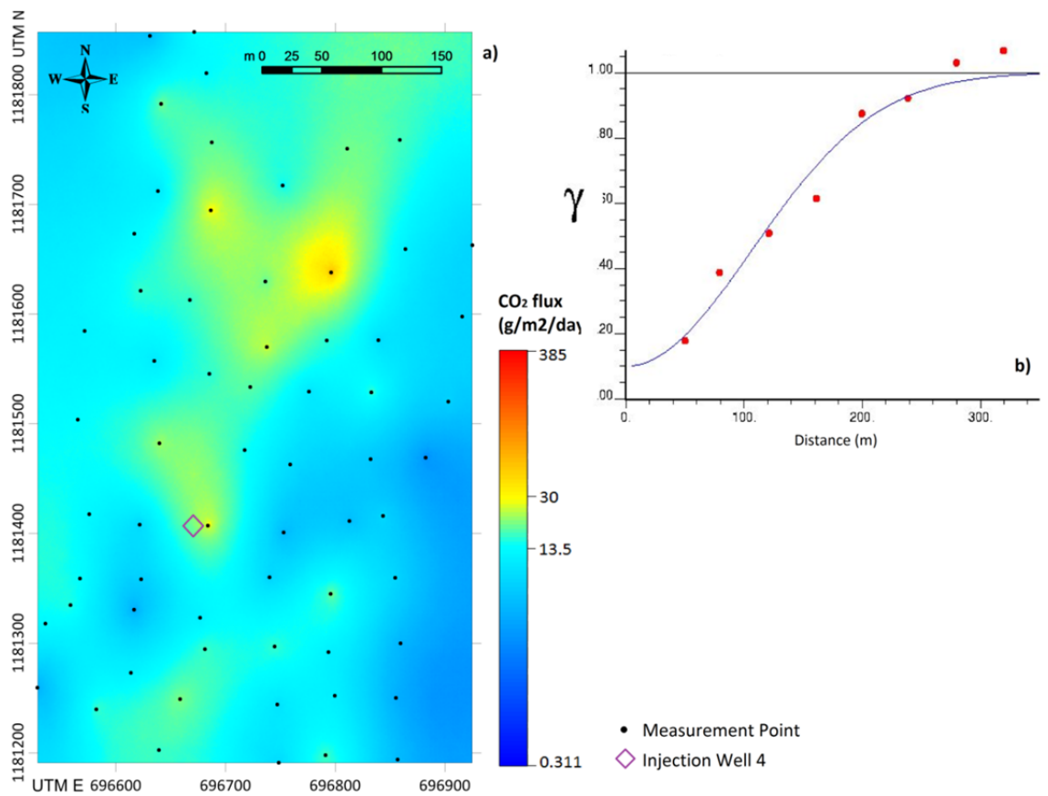
Fig. 15, a) CO 2 flux map of the IW 4 site with measurement locations represented by black dots, logarithmic color scale with significant flux values and b) empirical semi-variogram (red dots) and semi-variogram model (blue line) used for computing CO 2 flux with sGs, horizontal distance of measurement points on the x-axis and \gamma for the variance on the y-axis, where a value of 1 corresponds to a total absence of spatial auto-correlation
