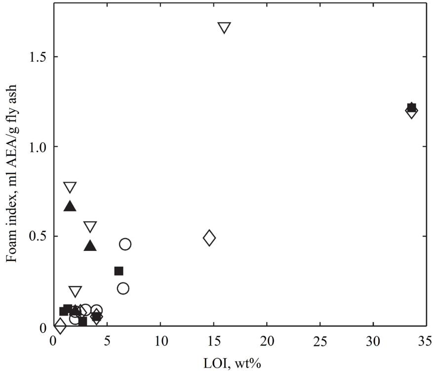
Figure 1.6* Foam index test versus LOI for five different studies, Courtesy of Perderson et al. (4). (∇)Freeman et al. (26);(◇) Yu et al. (27);(▲) Gao et al. (25); (■) Kúlaots et al. (11); and (○) Gao et al. (30) *Permission seen in Figure B-1
