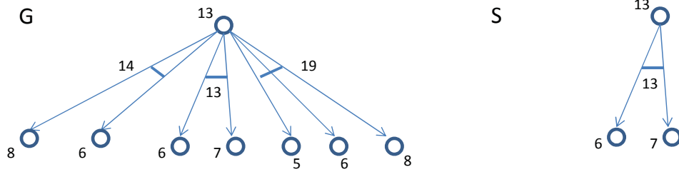
Figure 2.1: First expansion of the AND/OR graph.
