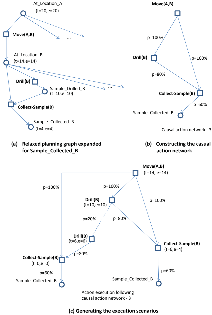
Figure 4.4: Example with actions that contain more than one precondition
