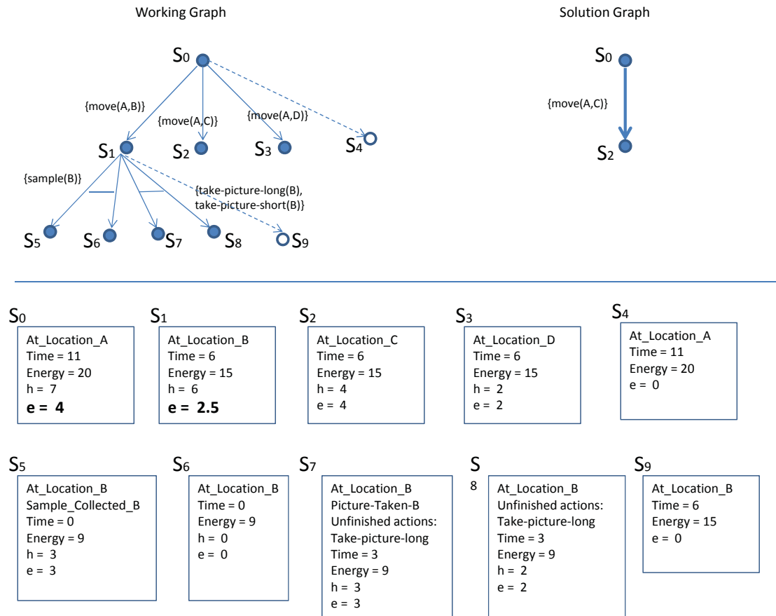
Figure 3.6: Update the expected reward for s_1 and s_0 , re-generate the solution graph.
