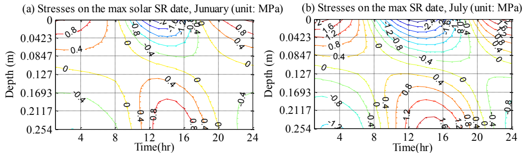
Figure 5.4. Predicted stress distribution in JPCP slabs during the maximum SR days in (a) January and (b) July (Tensile is Positive);
