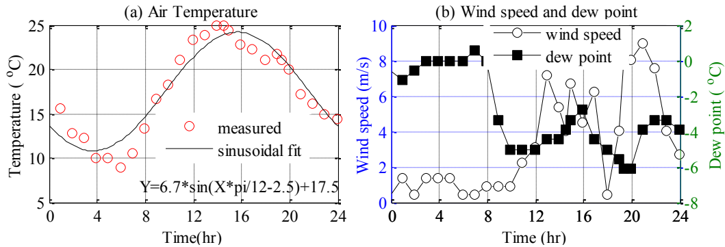
Figure 4.1 Air temperature and wind speed on July 12, 2010, in Reno, Nevada
