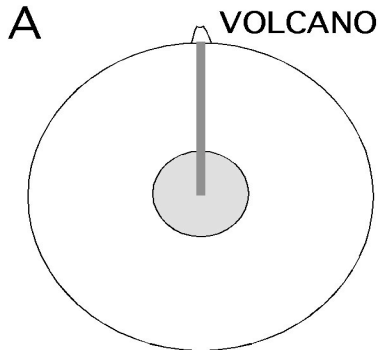
A. Material comes from the Earth's molten center
