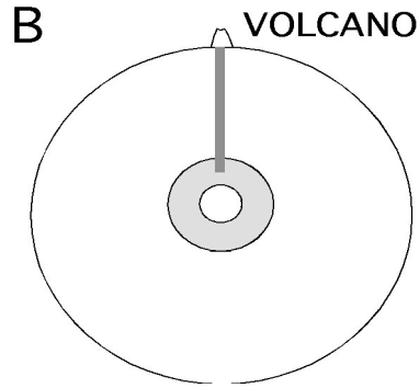
B. Material comes from a molten layer near the Earth's center
