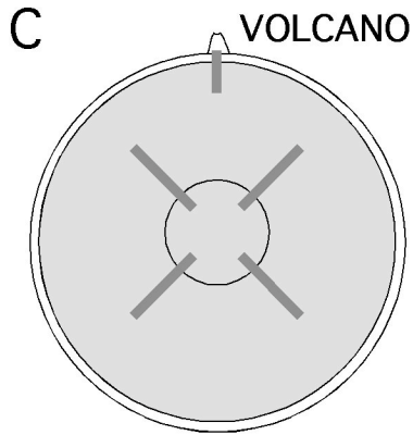
C. Material travels from the Earth's molten center and mixes with a molten layer beneath the Earth's surface
