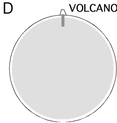
D. Material comes from a molten layer beneath the Earth's surface
