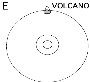
E. Material comes from pockets of molten material beneath the Earth's surface
